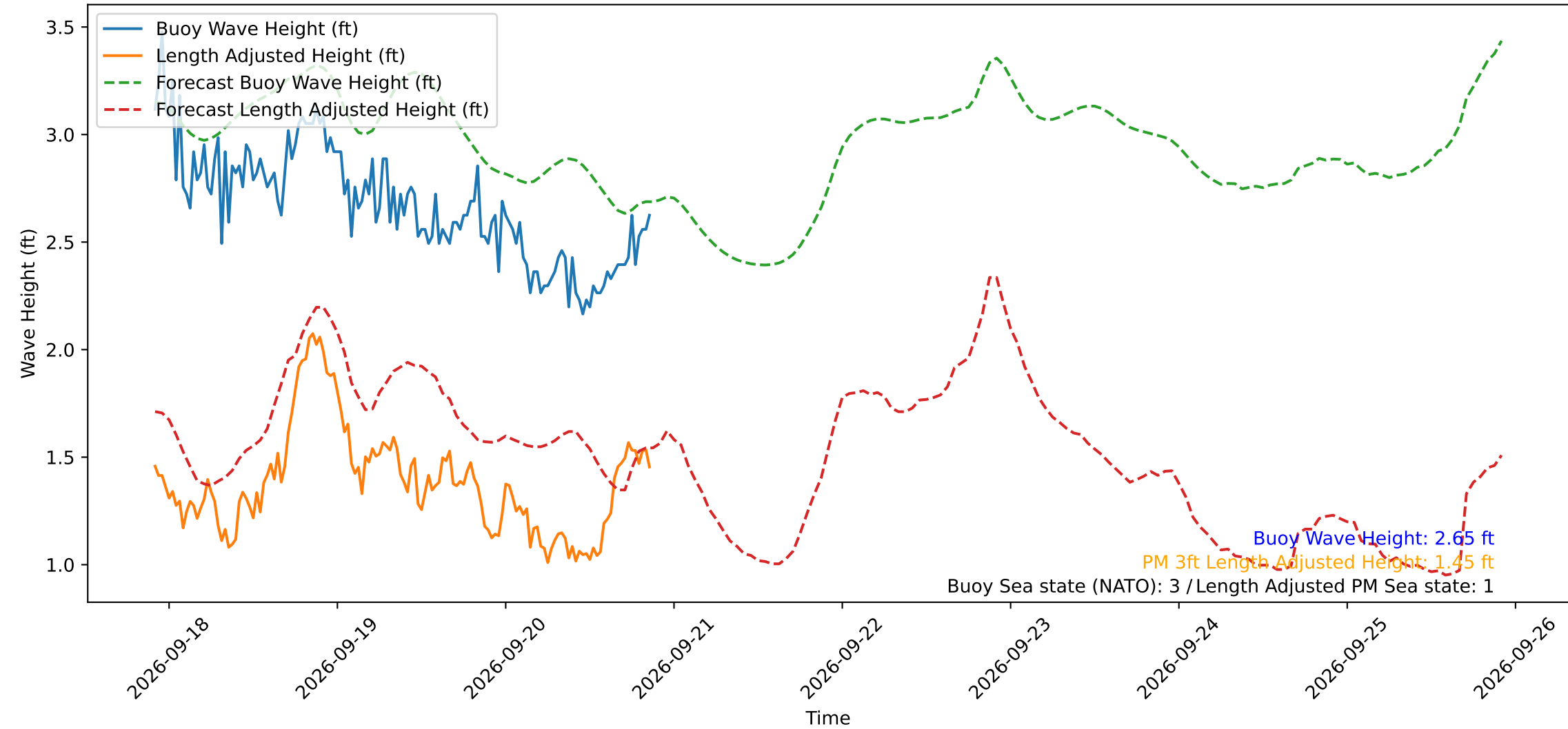
Wave Heights over Time for Green Beach at 2026-09-20 21:51:16
