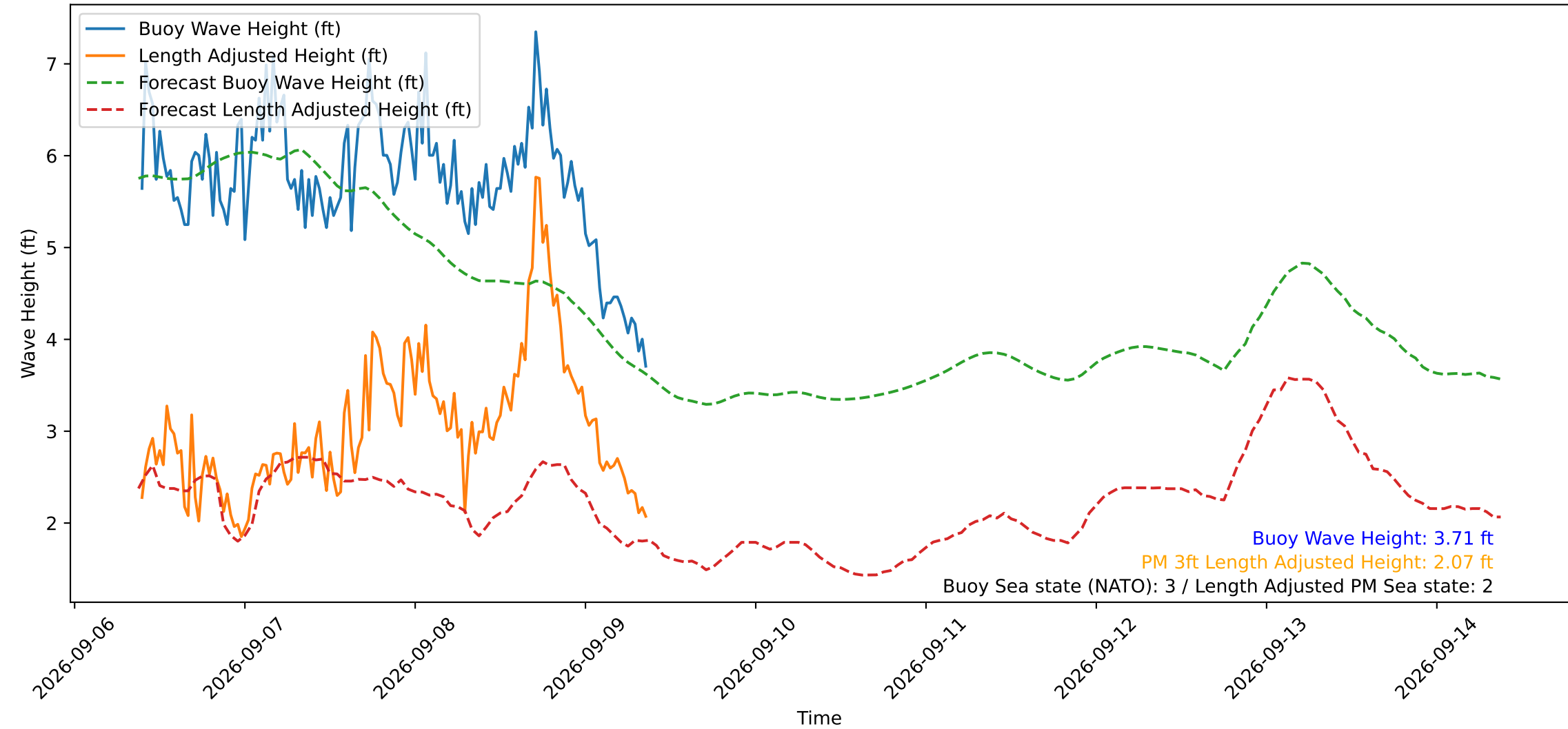
Wave Heights over Time for Oceanside Harbor at 2026-09-09 09:20:29
