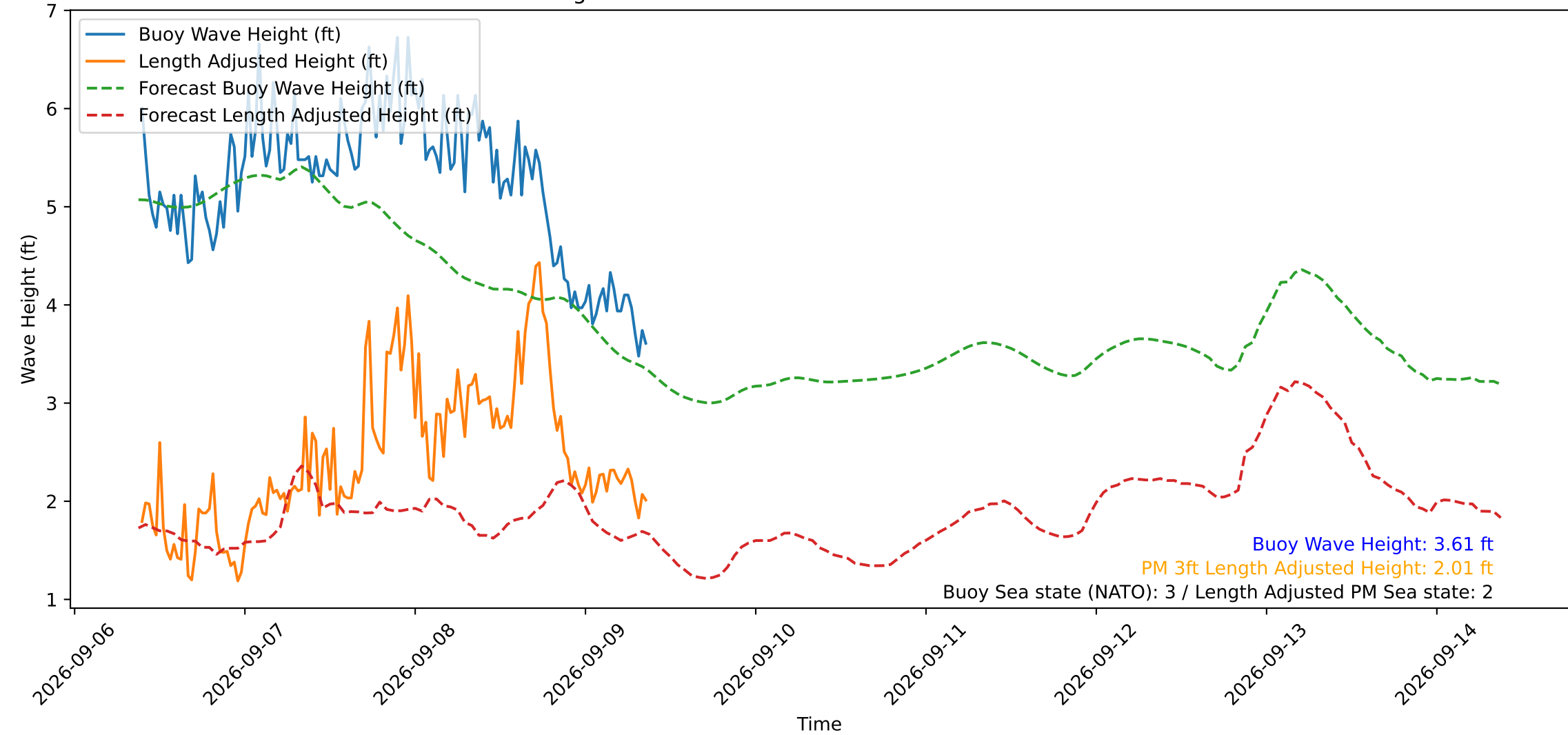
Wave Heights over Time for Red Beach at 2026-09-09 09:20:50
