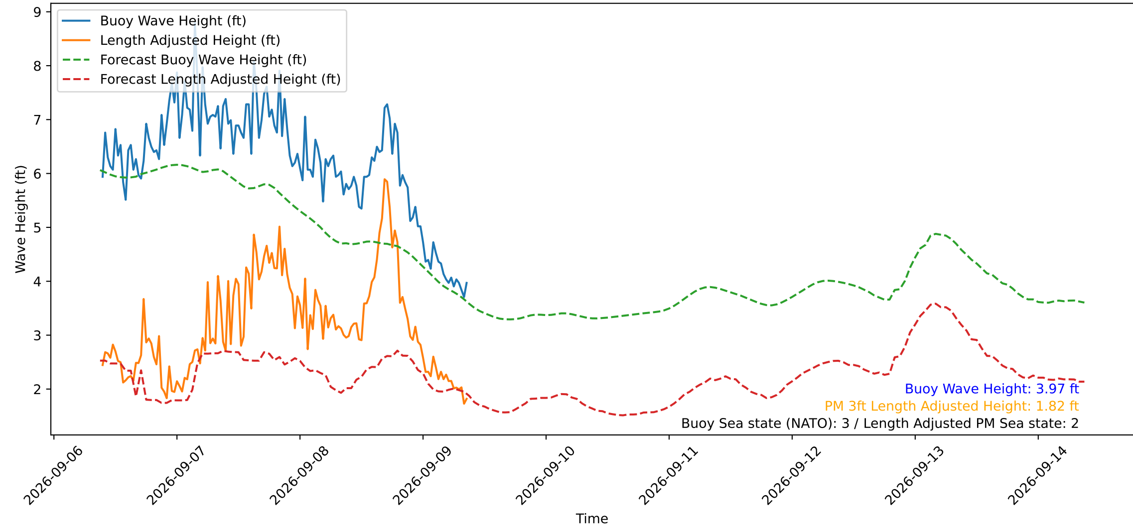
Wave Heights over Time for Green Beach at 2026-09-09 09:21:15
