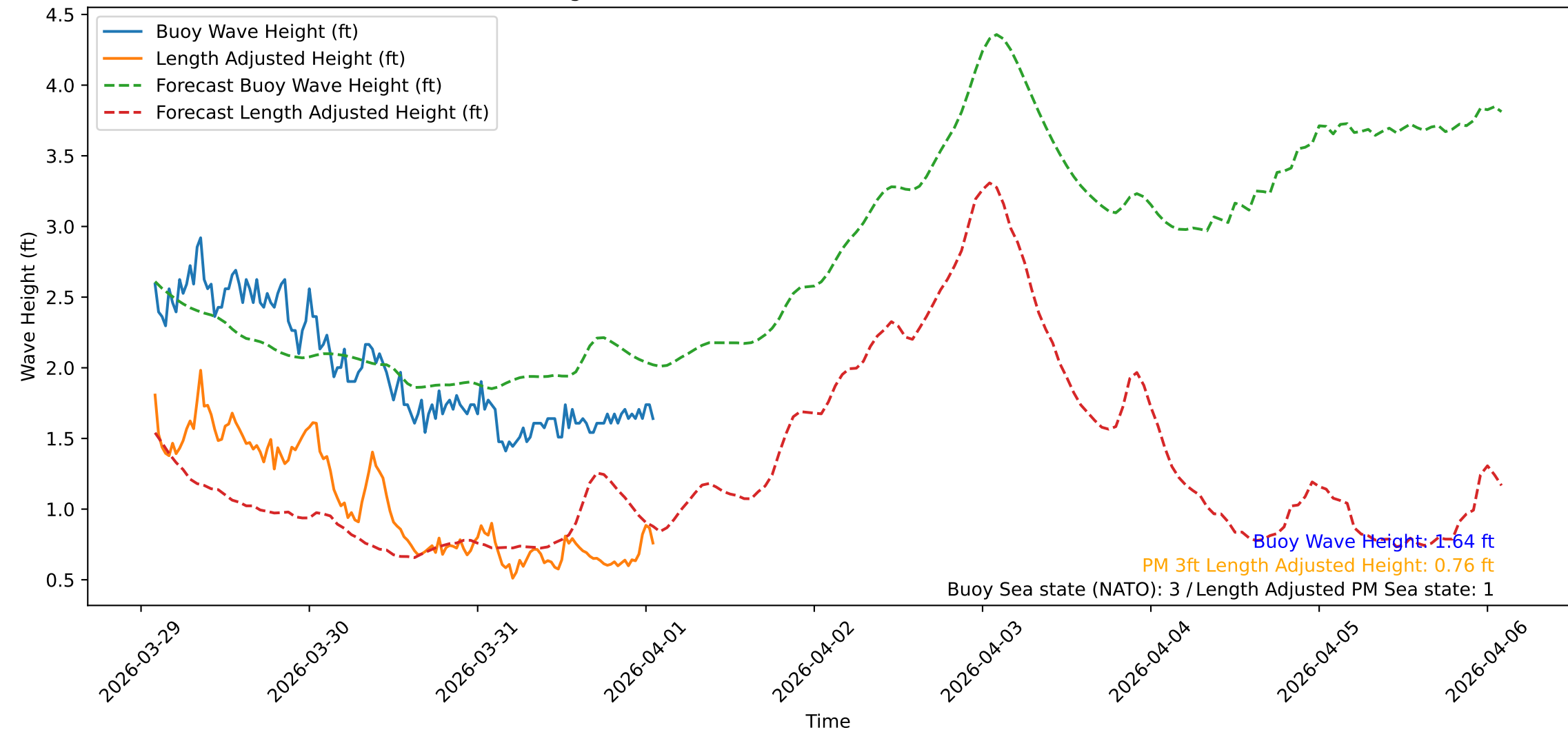
Wave Heights over Time for Green Beach at 2026-04-01 01:51:09
