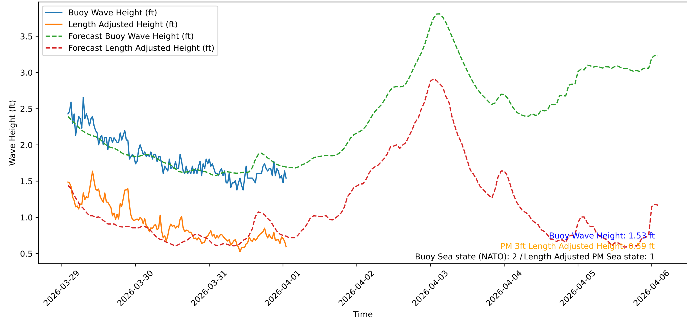
Wave Heights over Time for Red Beach at 2026-04-01 01:50:47
