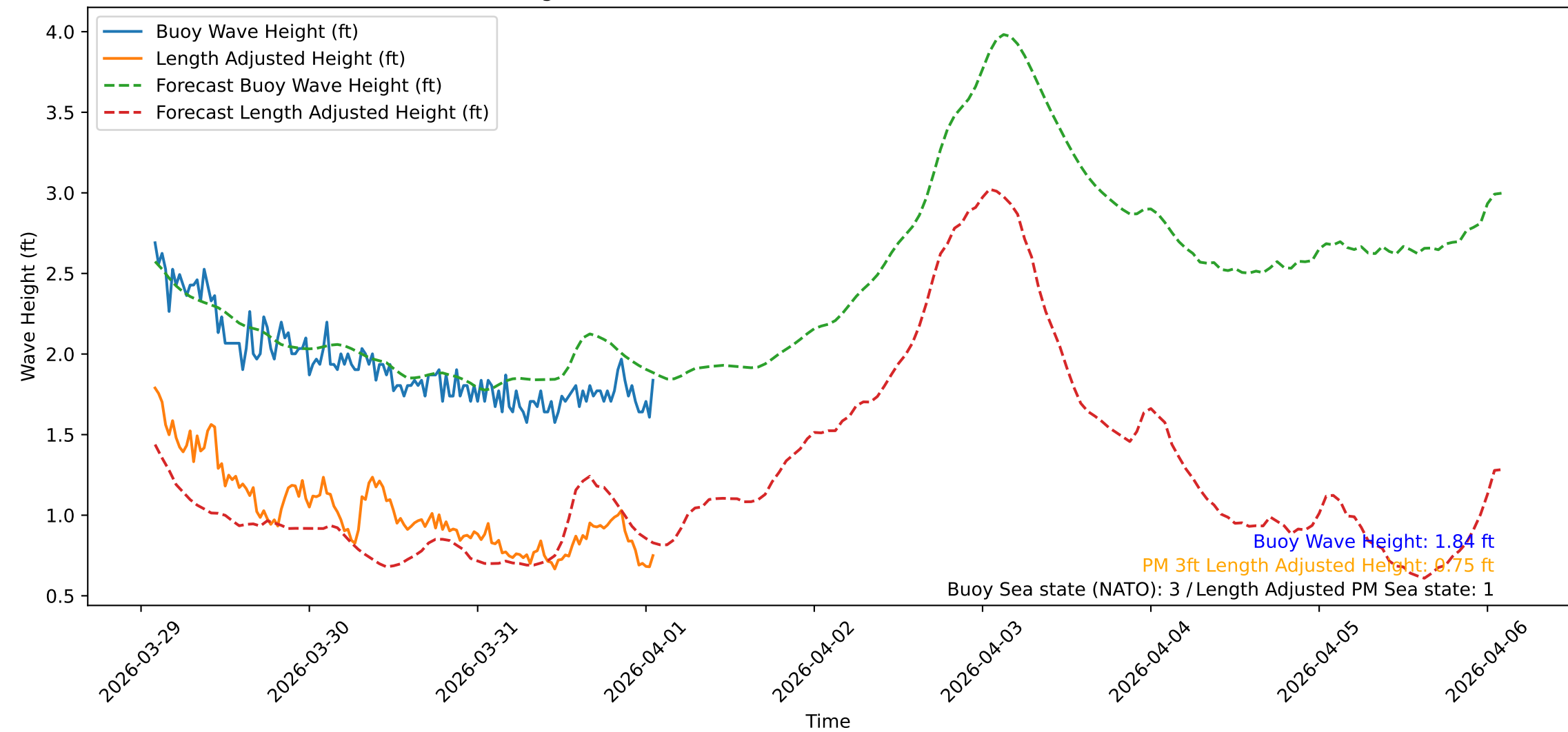
Wave Heights over Time for Oceanside Harbor at 2026-04-01 01:50:32
