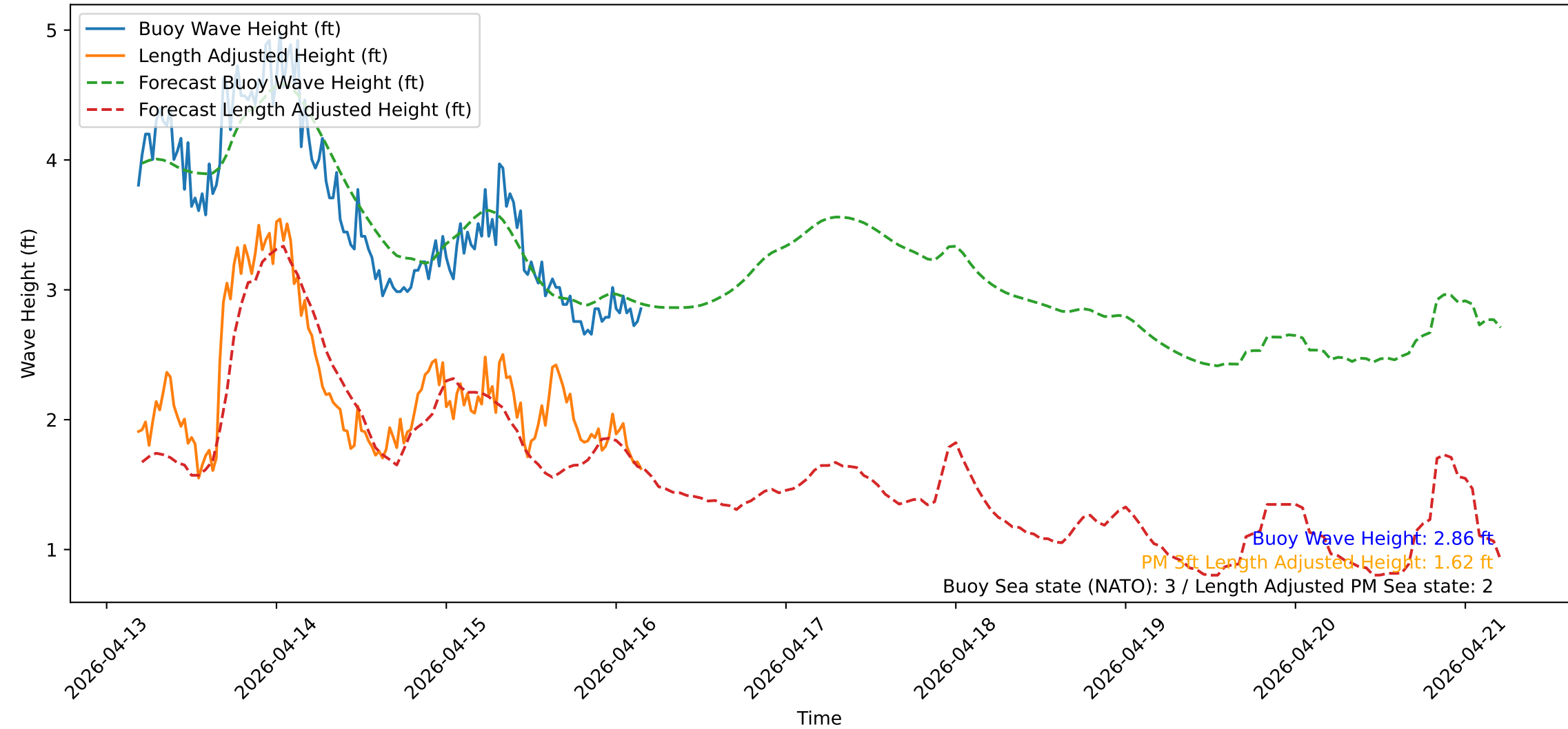
Wave Heights over Time for Green Beach at 2026-04-16 04:31:13
