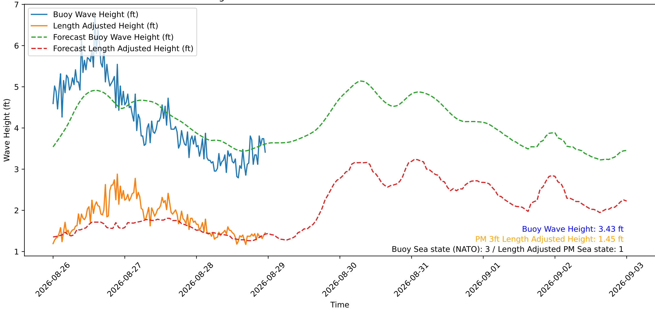
Wave Heights over Time for Oceanside Harbor at 2026-08-28 23:50:29
