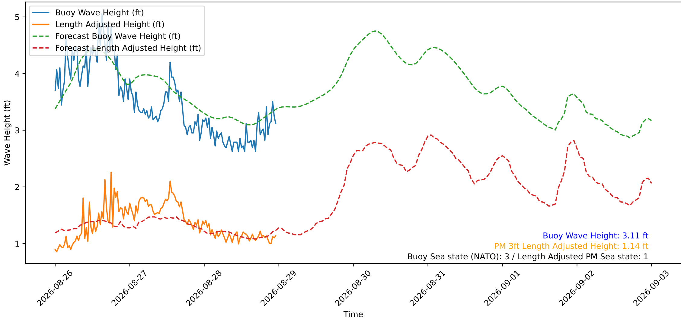
Wave Heights over Time for Red Beach at 2026-08-28 23:50:50
