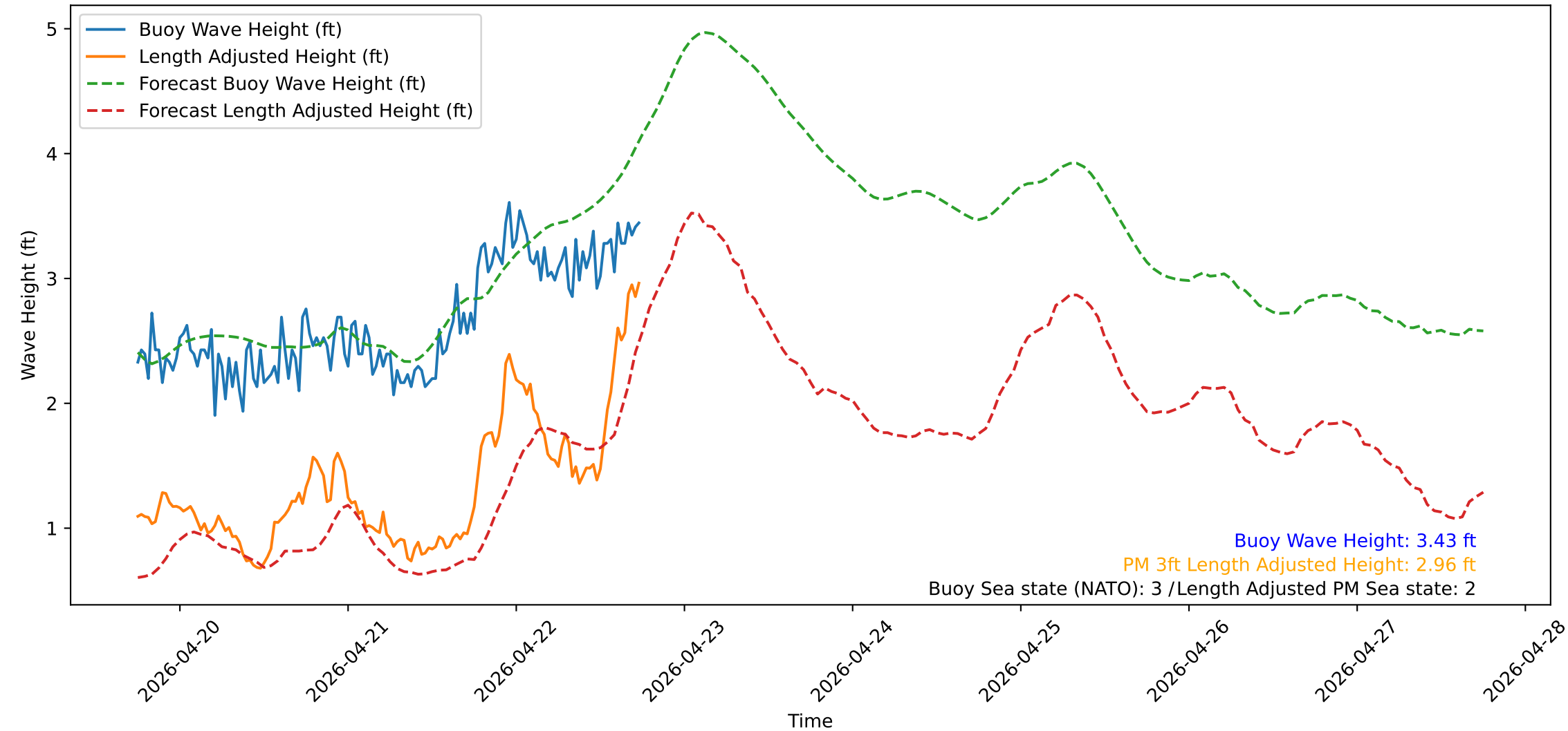
Wave Heights over Time for Oceanside Harbor at 2026-04-22 18:10:30
