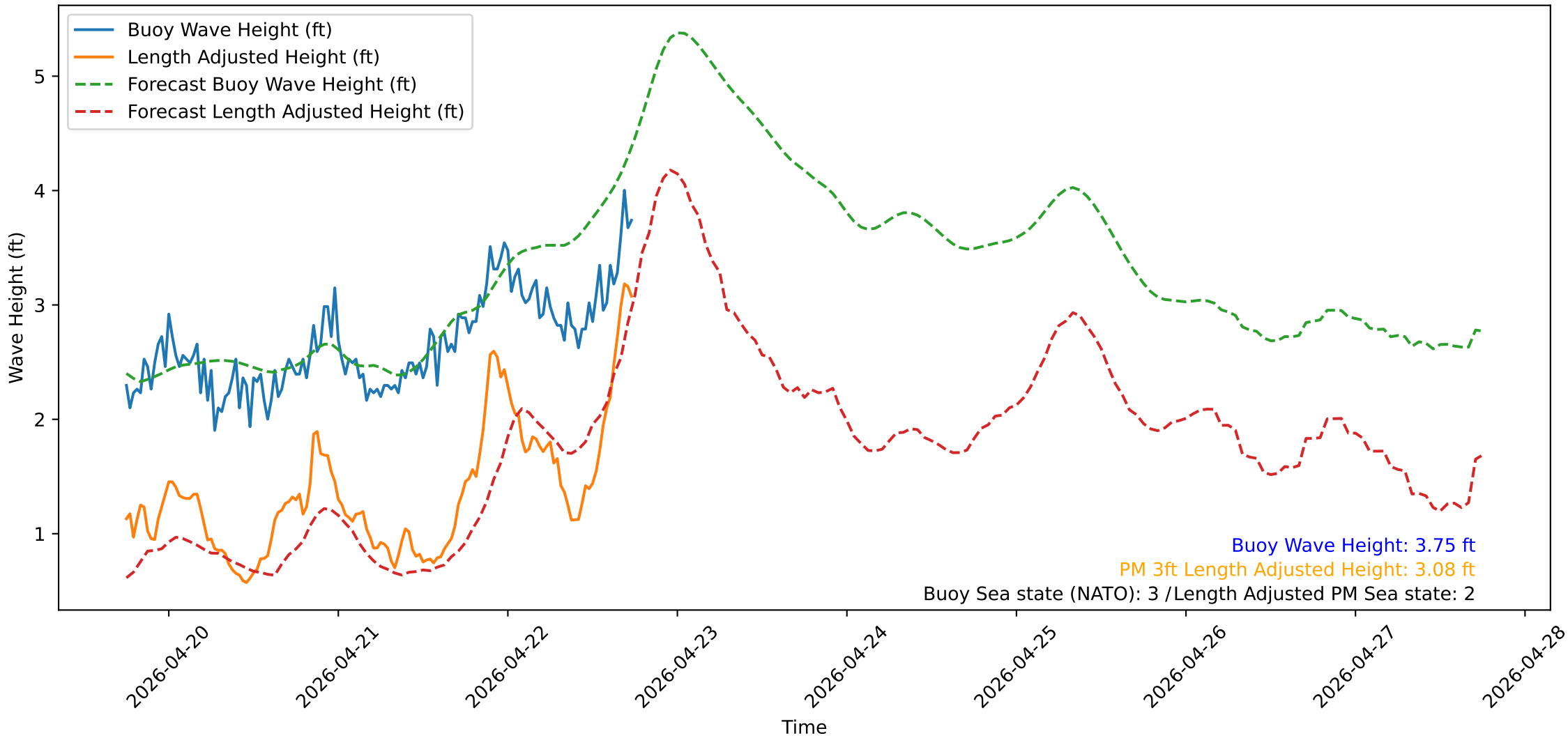
Wave Heights over Time for Green Beach at 2026-04-22 18:11:12
