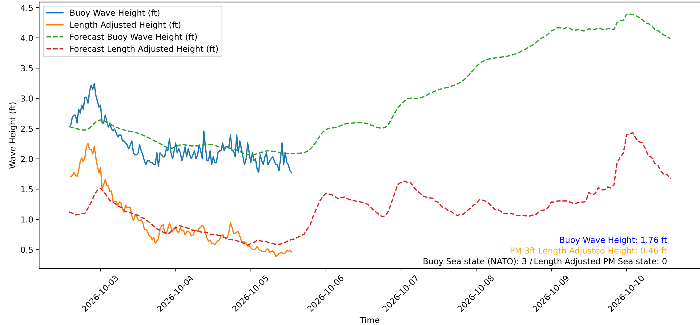
Wave Heights over Time for Red Beach at 2026-10-05 14:00:50
