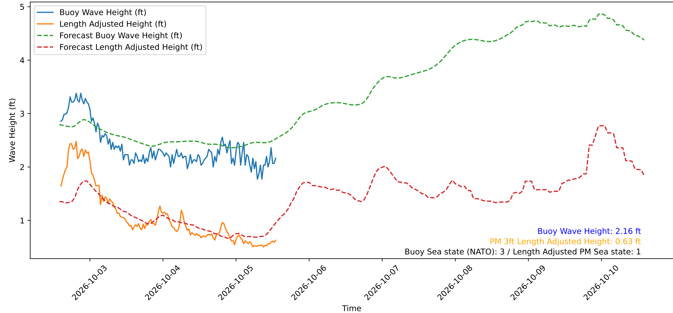
Wave Heights over Time for Green Beach at 2026-10-05 14:01:12
