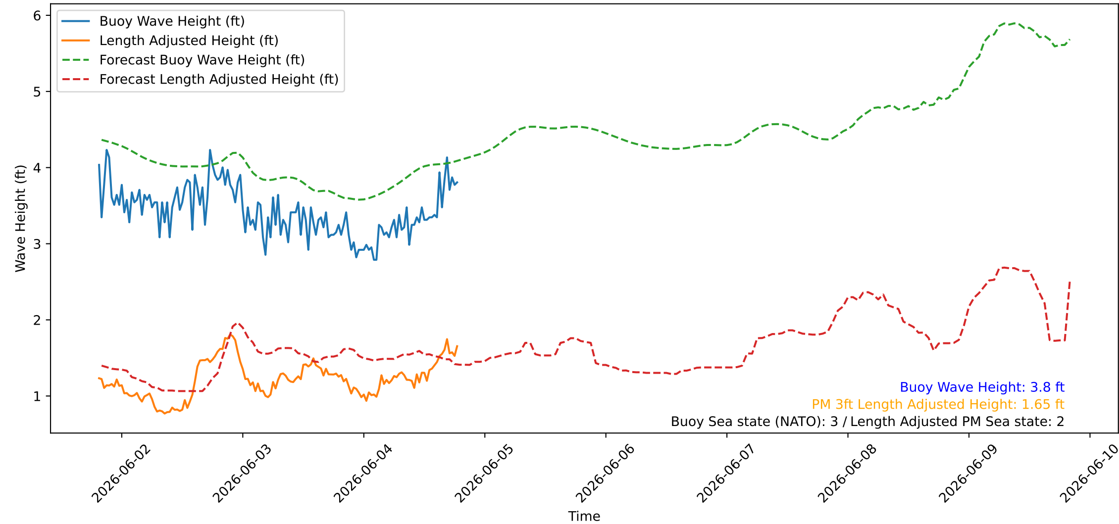
Wave Heights over Time for Green Beach at 2026-06-04 19:31:08
