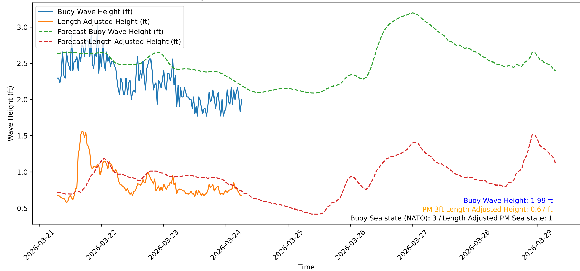
Wave Heights over Time for Oceanside Harbor at 2026-03-24 06:50:32
