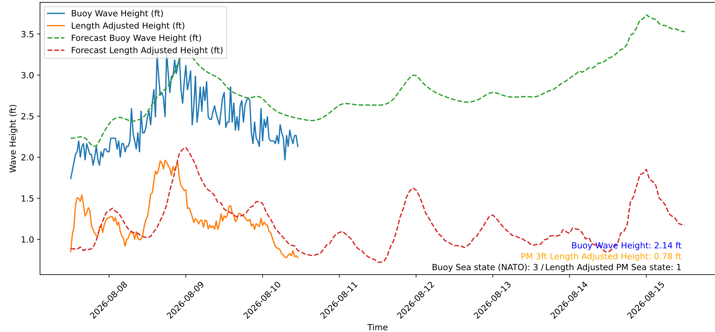
Wave Heights over Time for Oceanside Harbor at 2026-08-10 11:50:26
