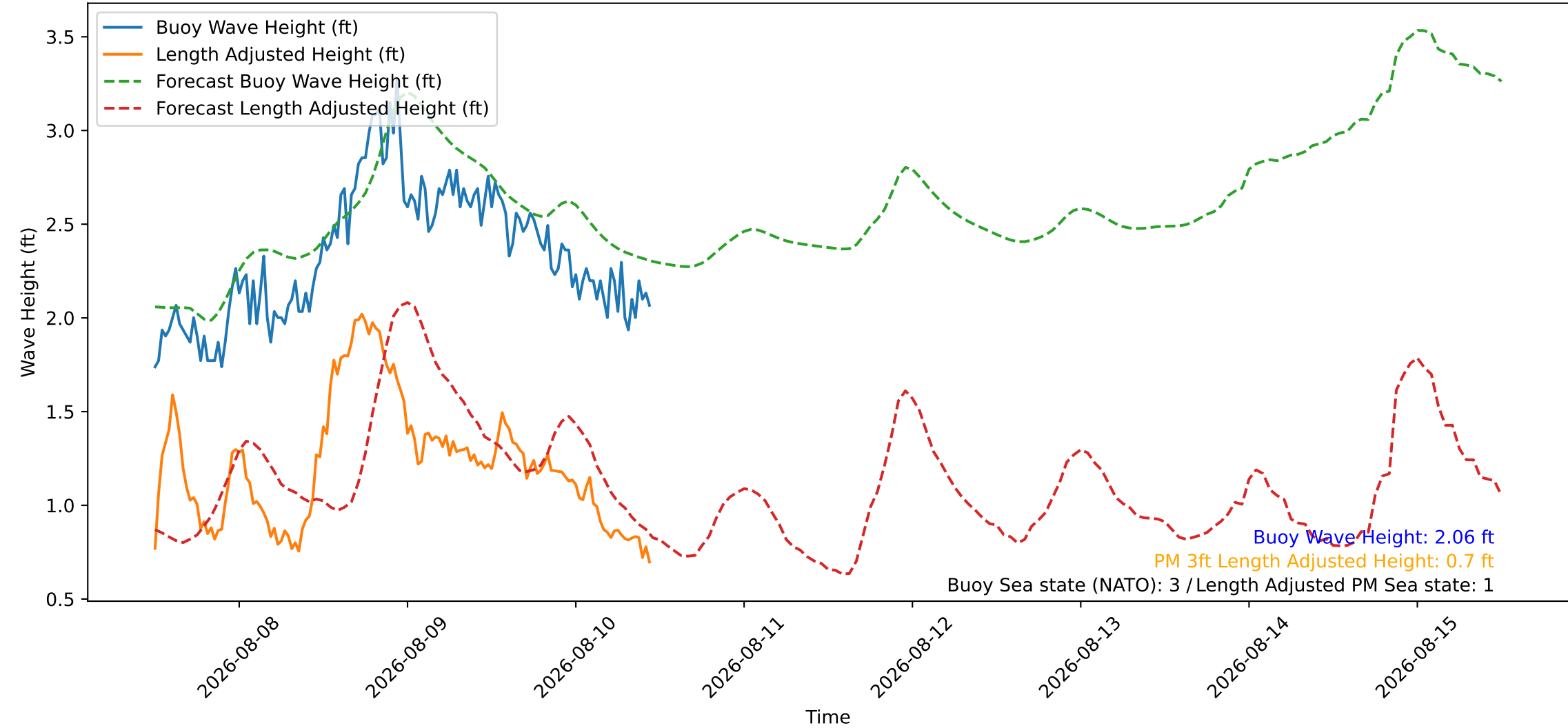
Wave Heights over Time for Red Beach at 2026-08-10 11:50:47
