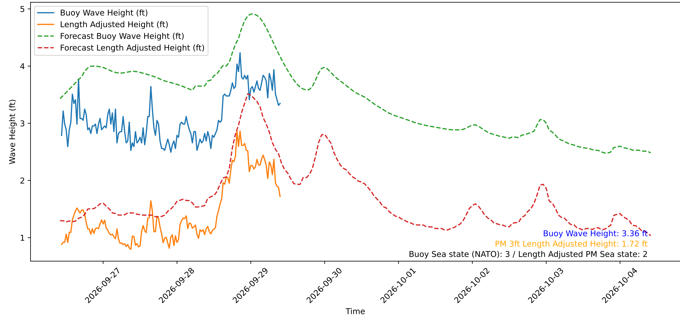
Wave Heights over Time for Oceanside Harbor at 2026-09-29 10:20:30
