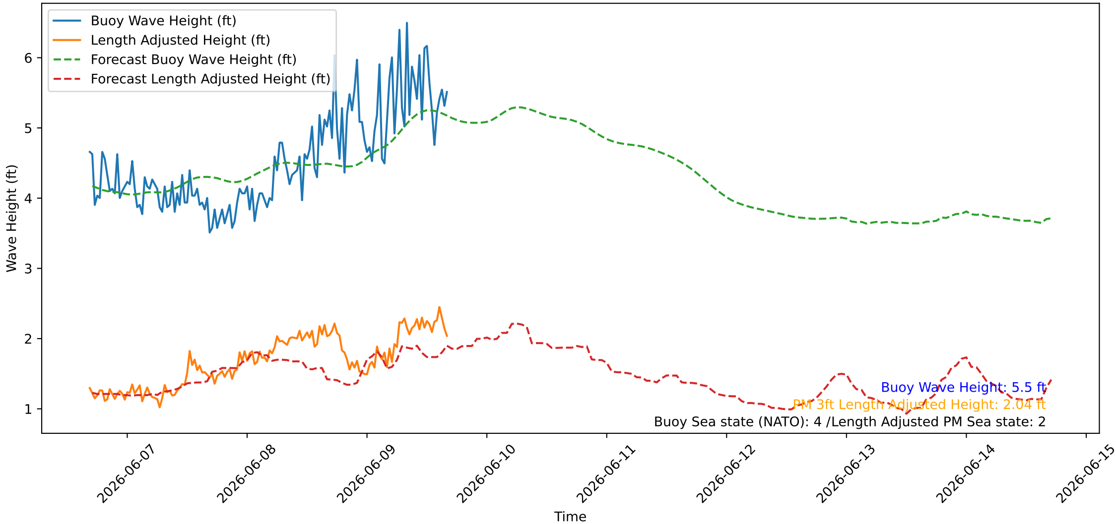
Wave Heights over Time for Oceanside Harbor at 2026-06-09 16:40:27
