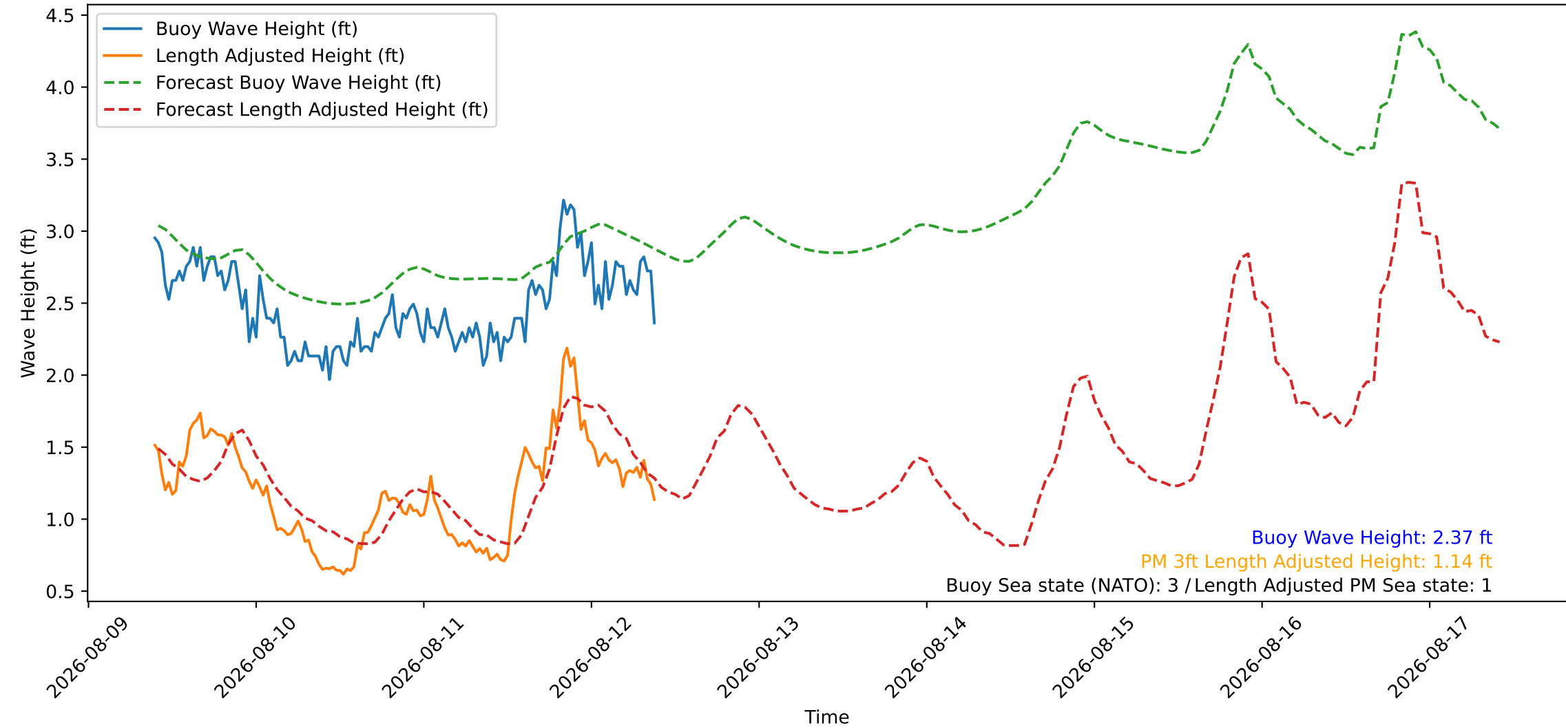
Wave Heights over Time for Green Beach at 2026-08-12 09:41:09
