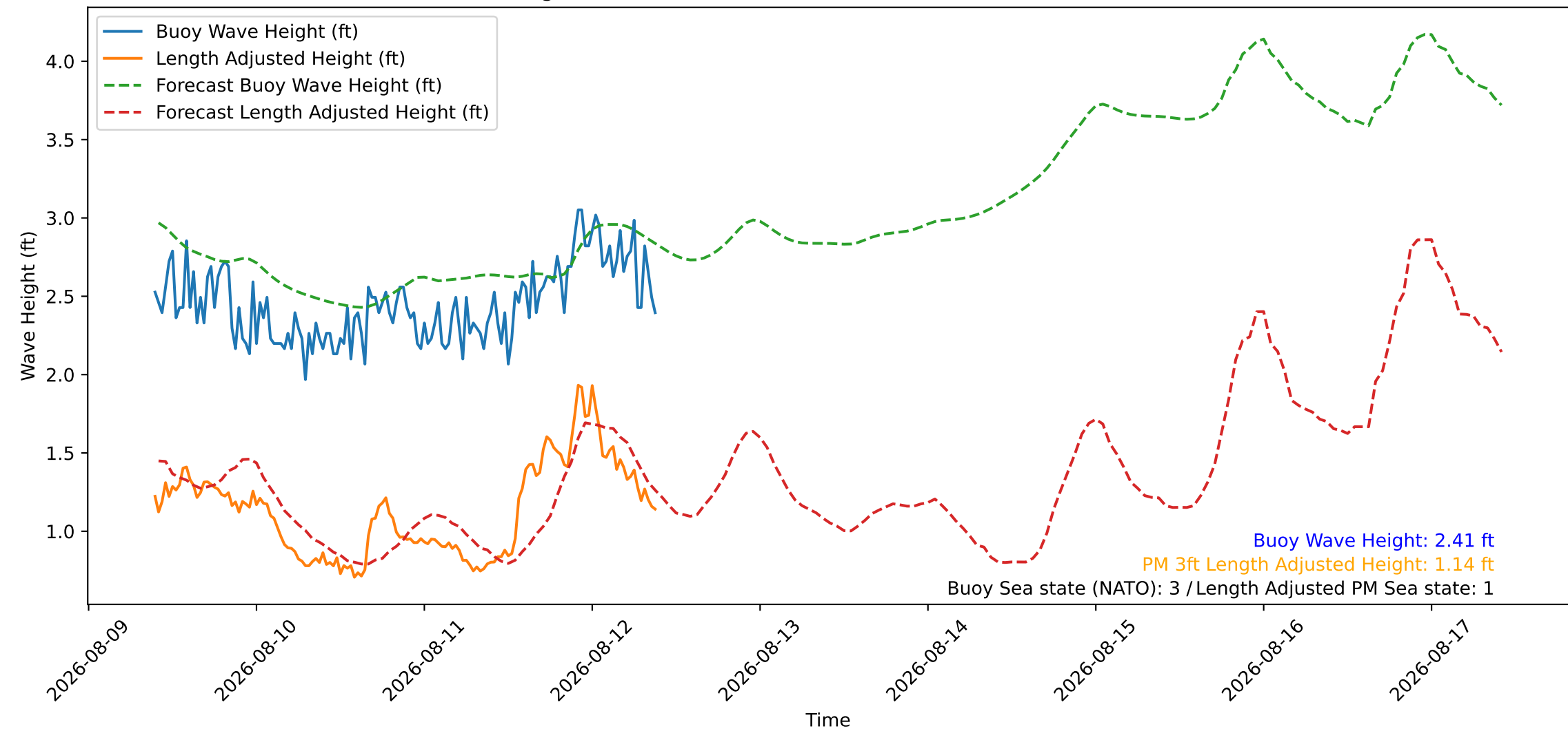
Wave Heights over Time for Oceanside Harbor at 2026-08-12 09:40:27
