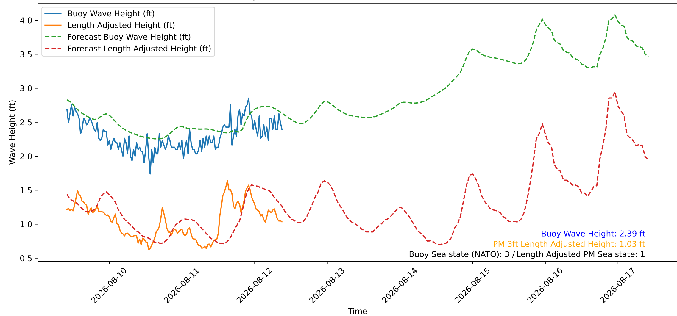
Wave Heights over Time for Red Beach at 2026-08-12 09:40:47
