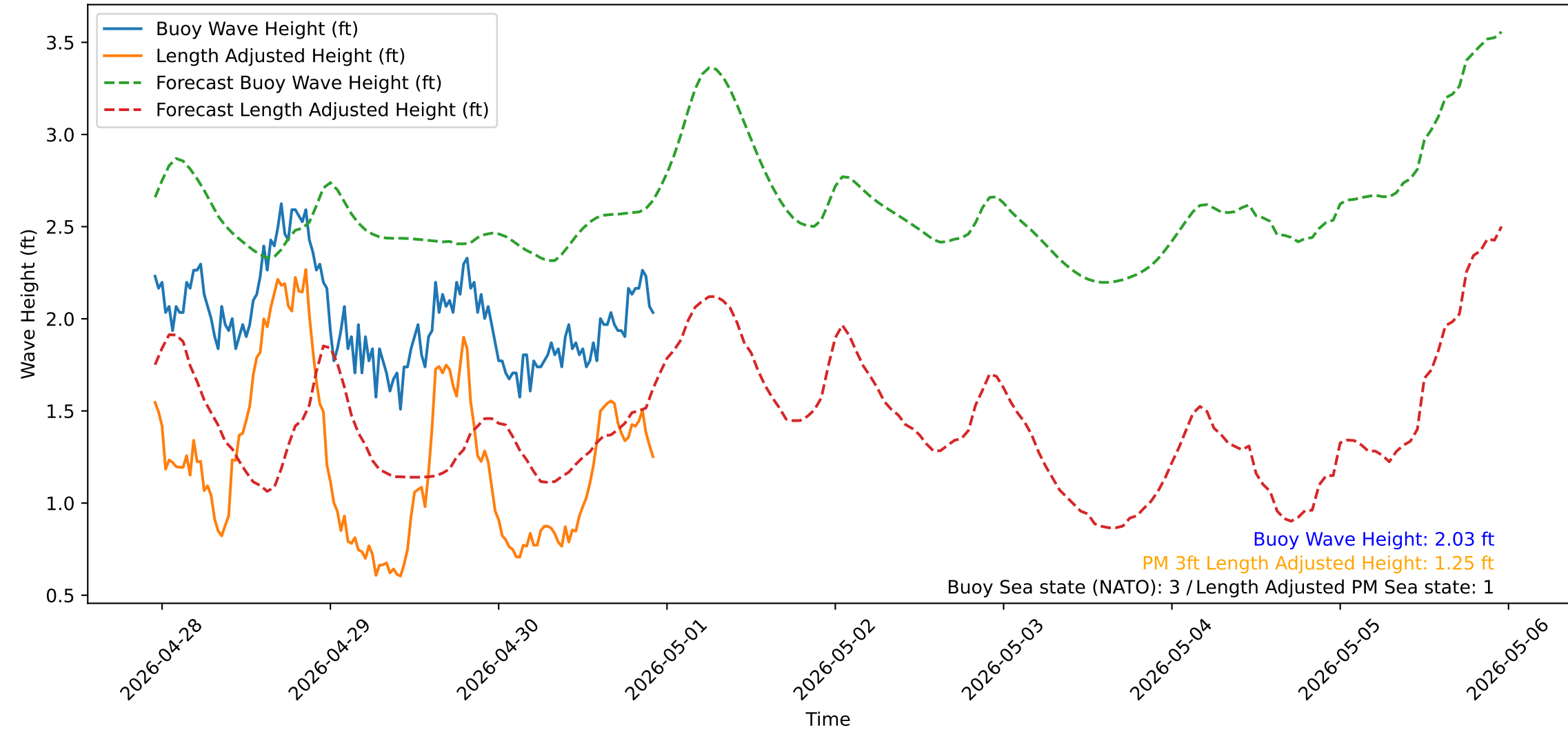
Wave Heights over Time for Red Beach at 2026-04-30 22:50:51
