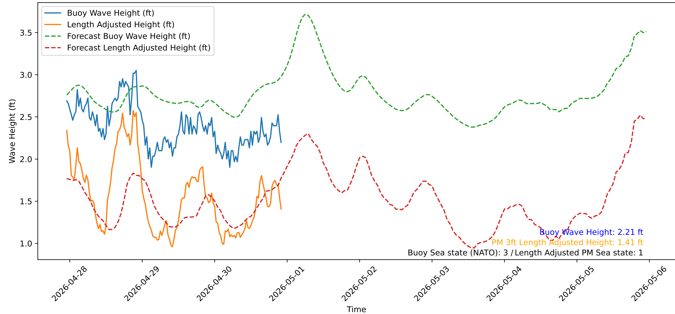
Wave Heights over Time for Oceanside Harbor at 2026-04-30 22:50:31
