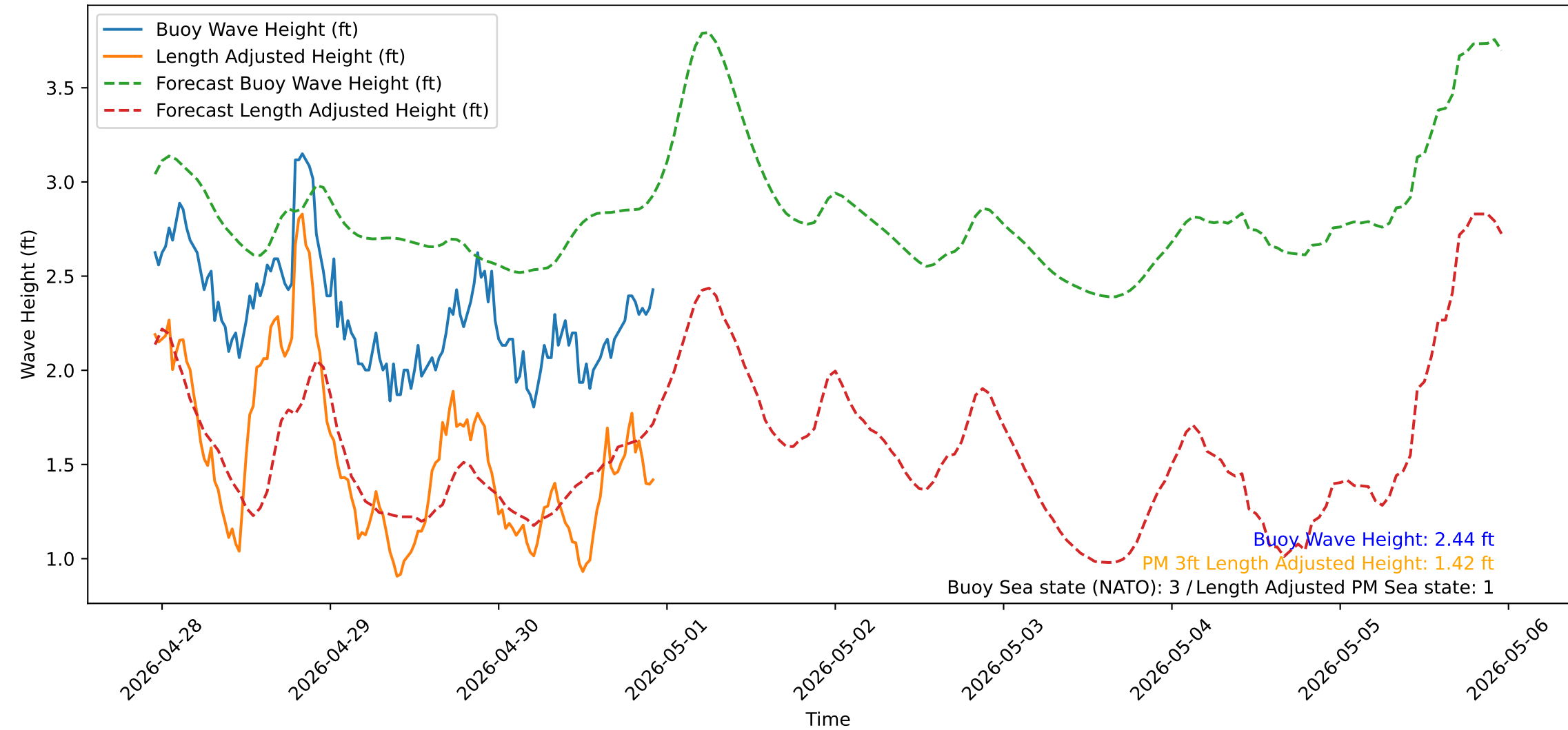
Wave Heights over Time for Green Beach at 2026-04-30 22:51:14
