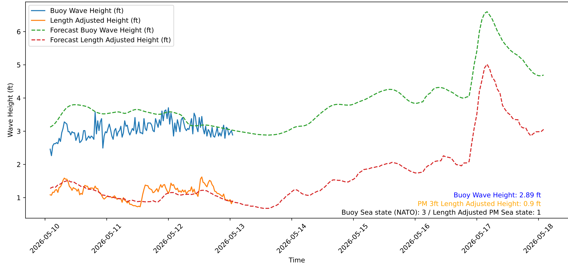
Wave Heights over Time for Oceanside Harbor at 2026-05-13 01:50:31
