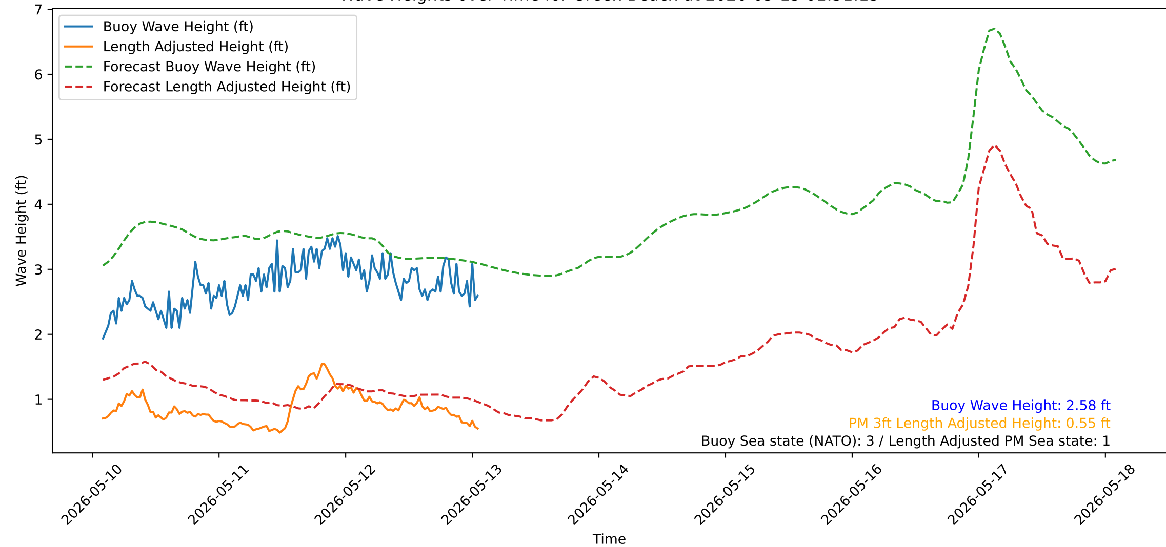
Wave Heights over Time for Green Beach at 2026-05-13 01:51:13
