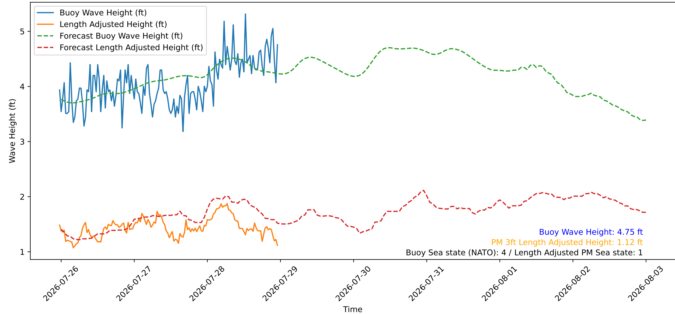
Wave Heights over Time for Oceanside Harbor at 2026-07-28 23:40:27
