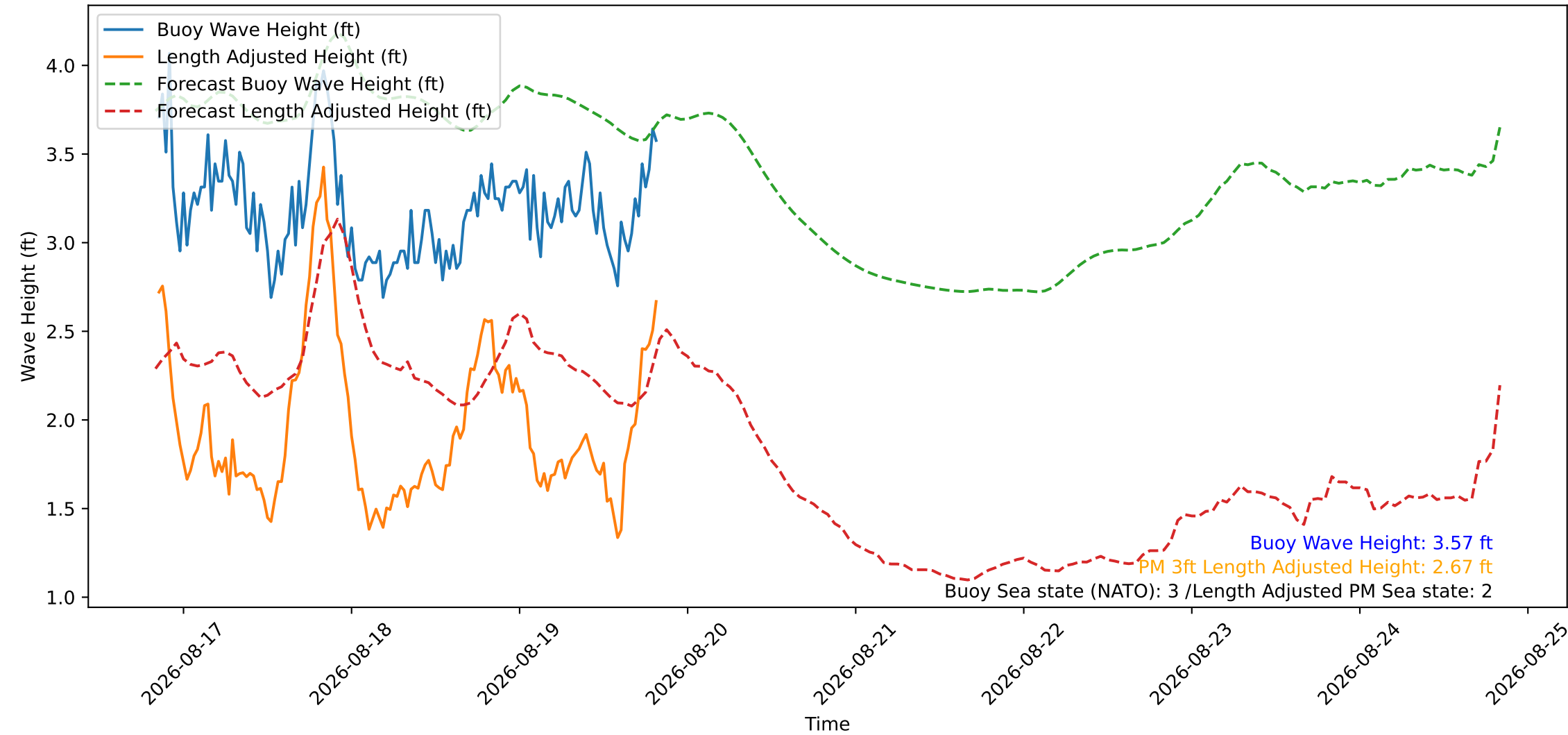
Wave Heights over Time for Green Beach at 2026-08-19 20:11:08
