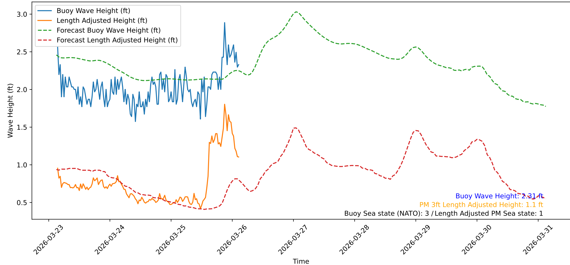
Wave Heights over Time for Oceanside Harbor at 2026-03-26 03:20:31
