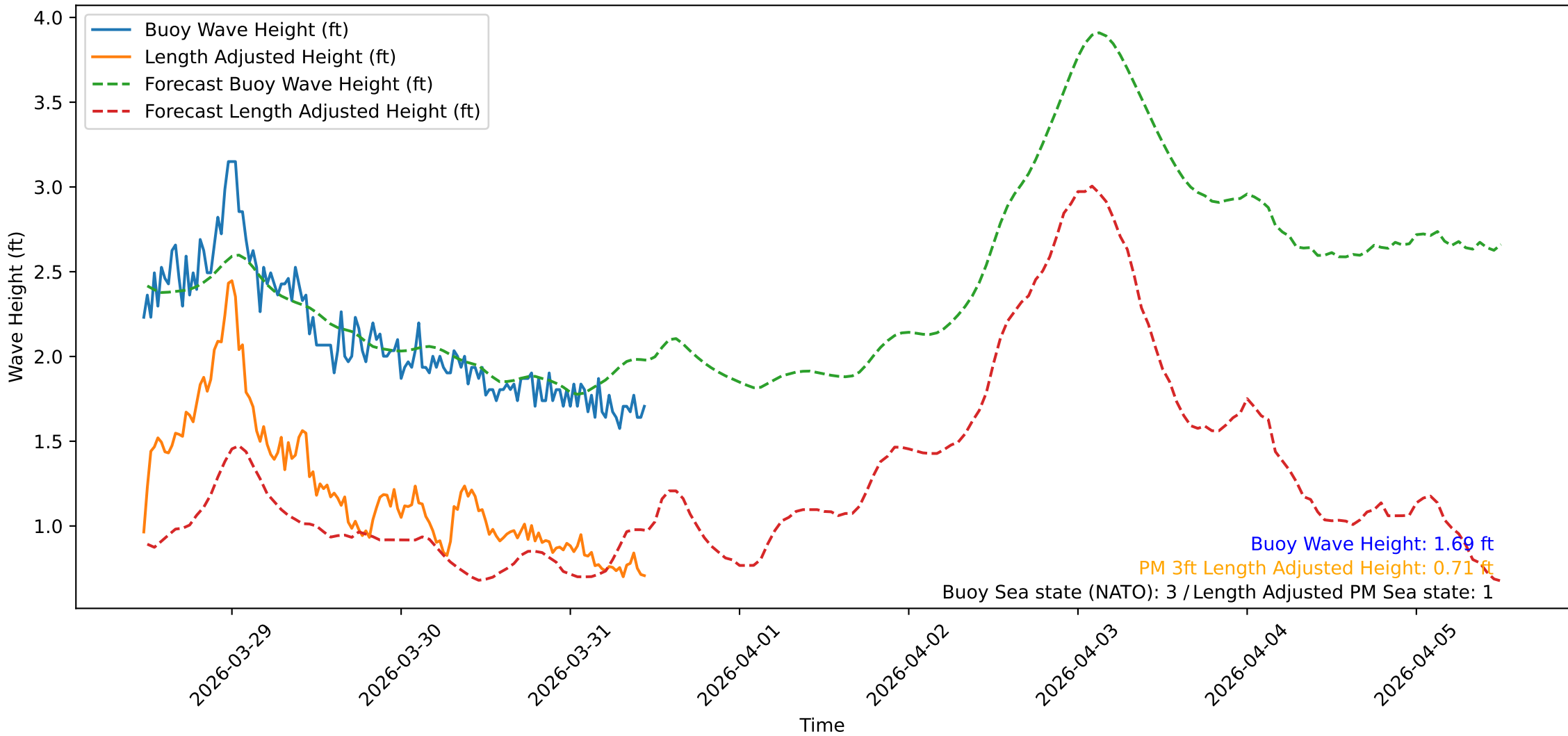
Wave Heights over Time for Oceanside Harbor at 2026-03-31 11:30:31
