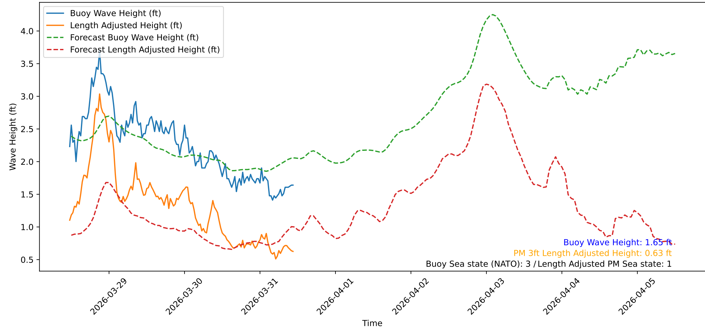
Wave Heights over Time for Green Beach at 2026-03-31 11:31:10
