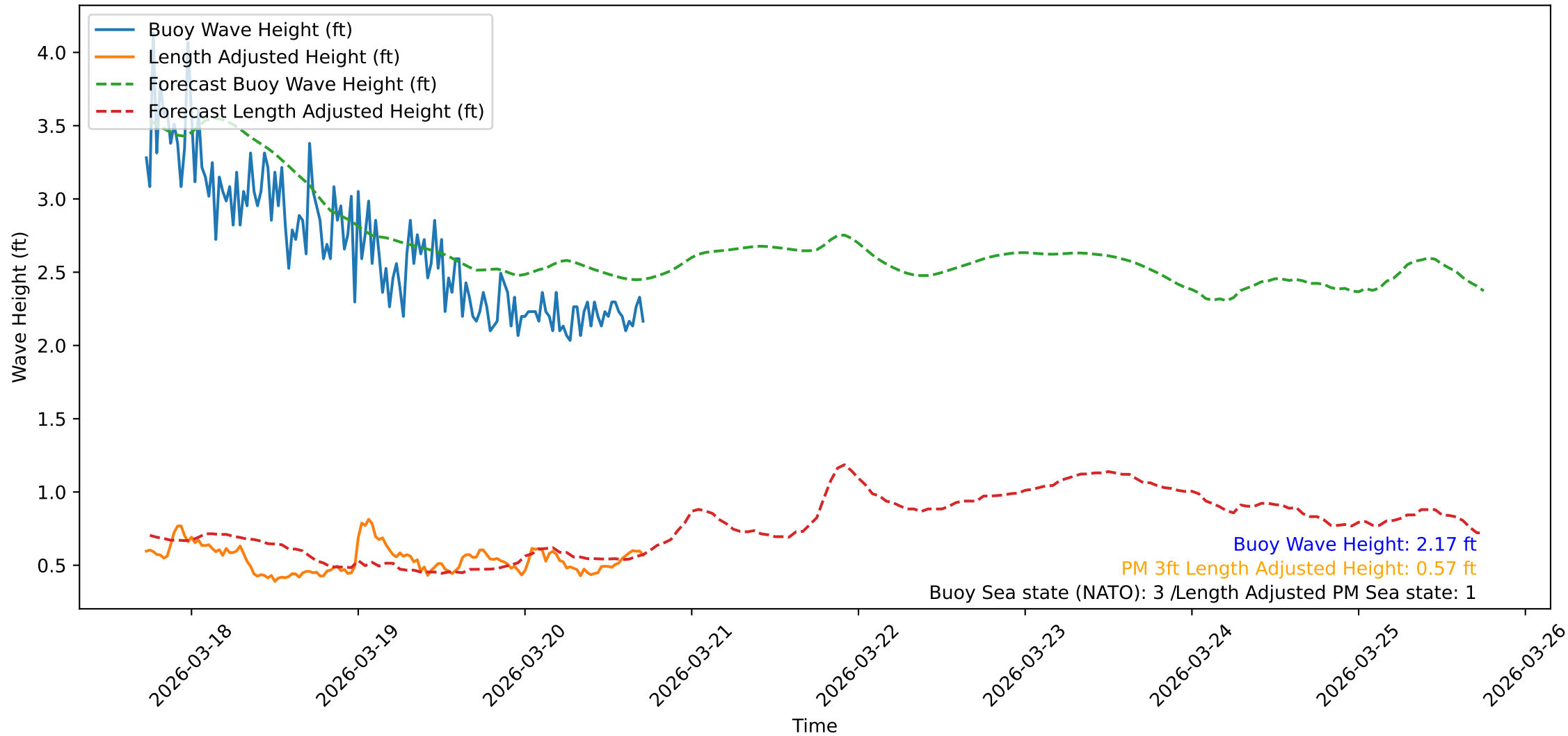
Wave Heights over Time for Green Beach at 2026-03-20 17:41:09
