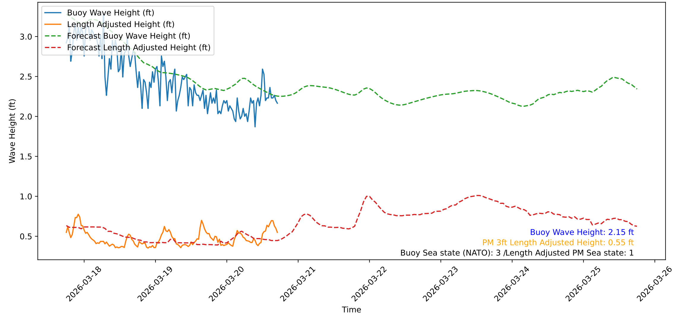
Wave Heights over Time for Red Beach at 2026-03-20 17:40:47
