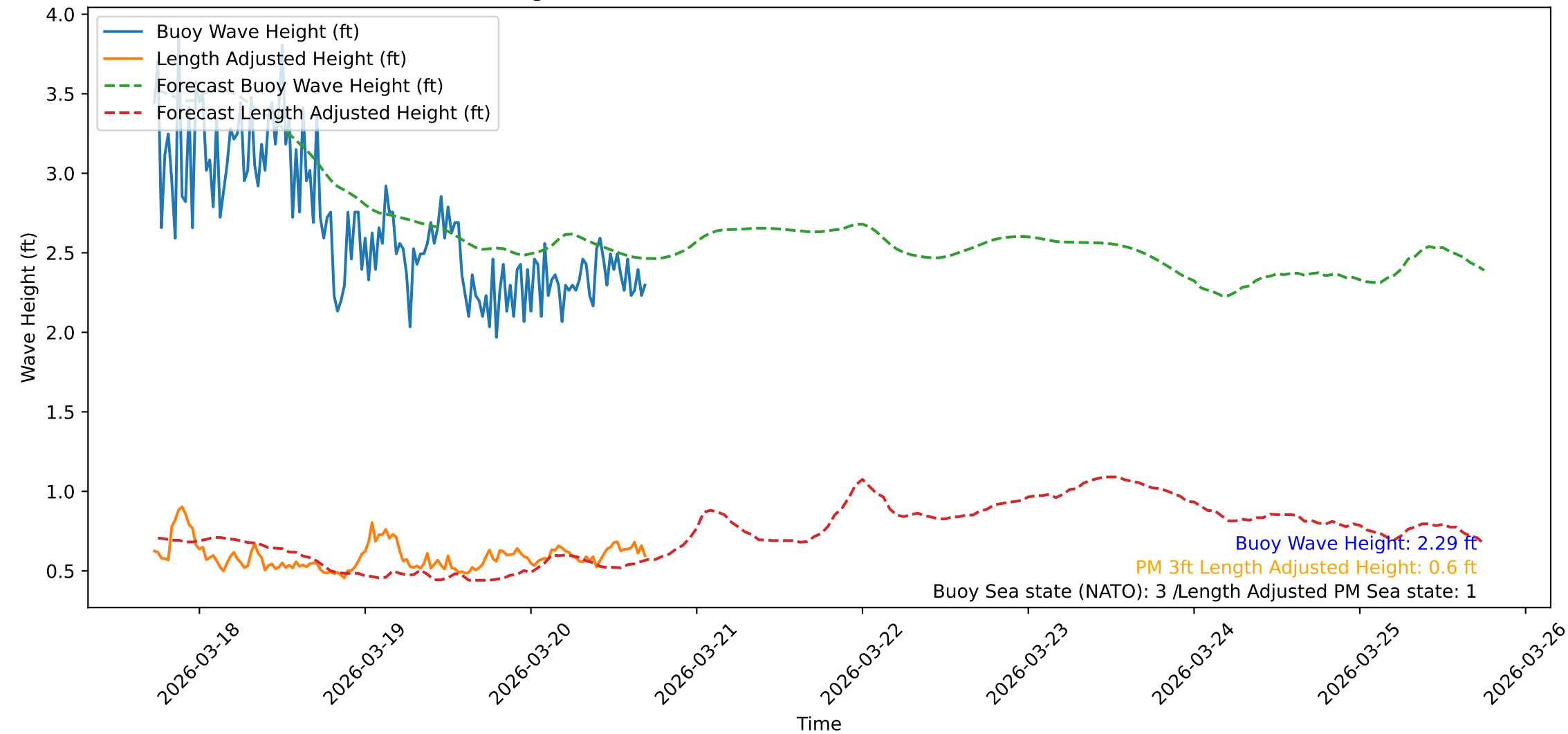
Wave Heights over Time for Oceanside Harbor at 2026-03-20 17:40:31
