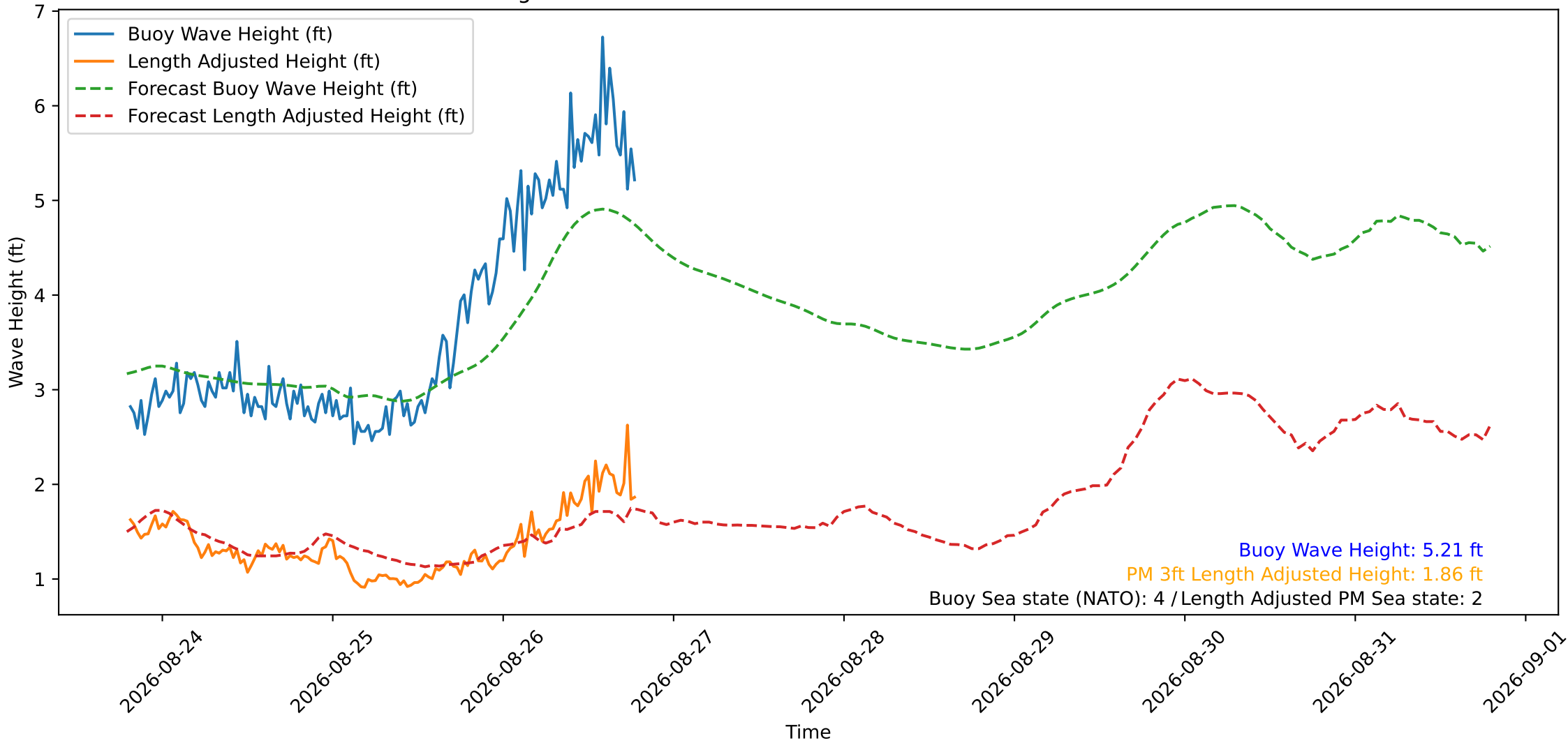
Wave Heights over Time for Oceanside Harbor at 2026-08-26 19:20:29
