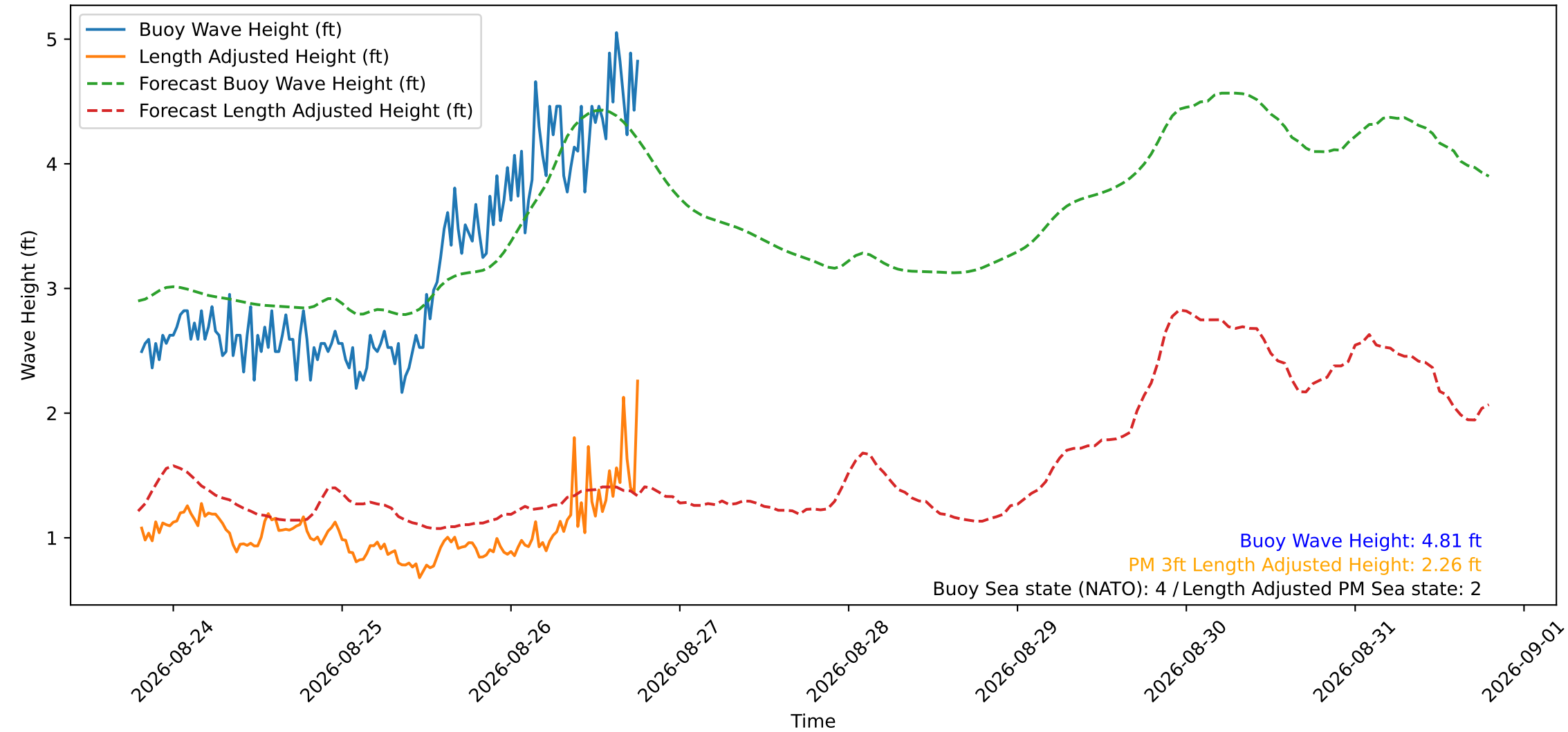
Wave Heights over Time for Red Beach at 2026-08-26 19:20:50
