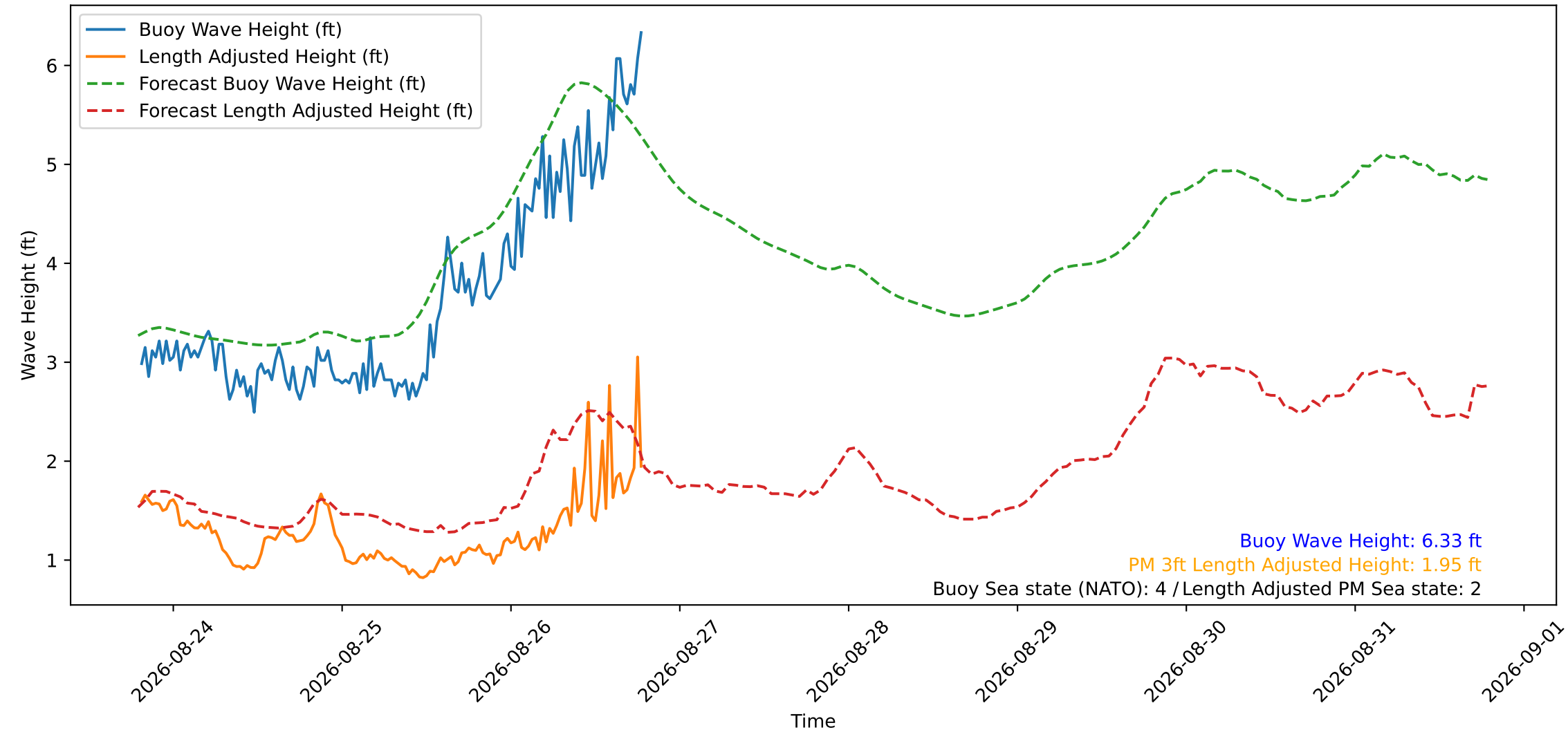
Wave Heights over Time for Green Beach at 2026-08-26 19:21:14
