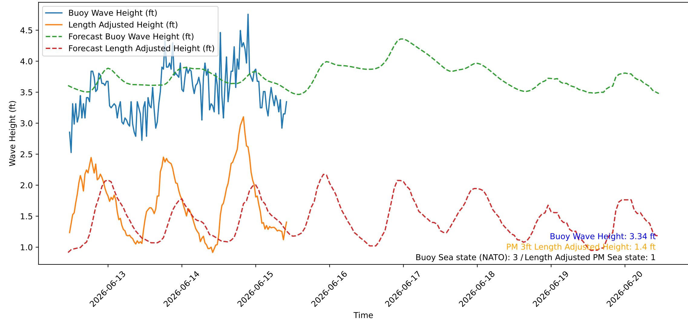
Wave Heights over Time for Red Beach at 2026-06-15 11:00:45
