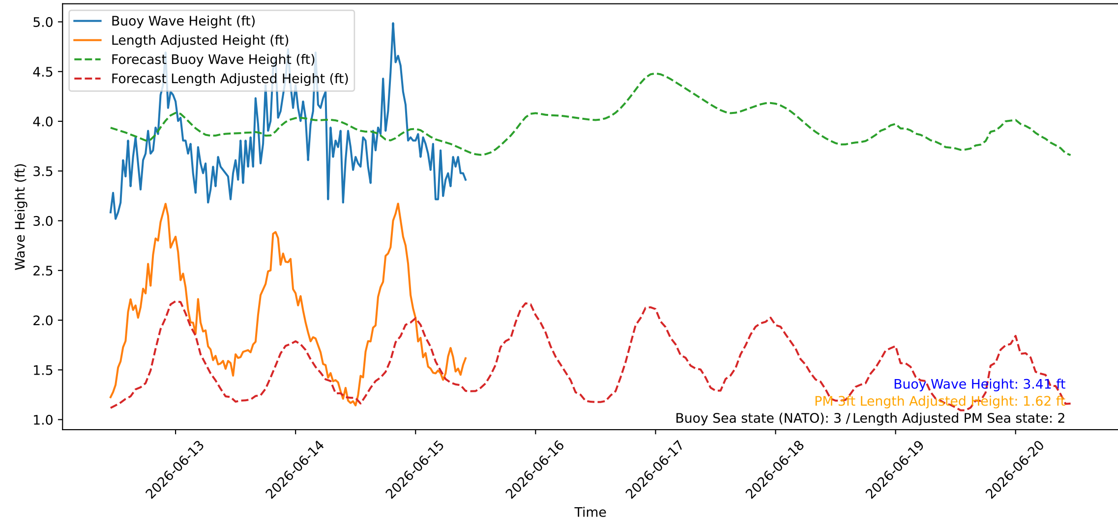
Wave Heights over Time for Oceanside Harbor at 2026-06-15 11:00:26
