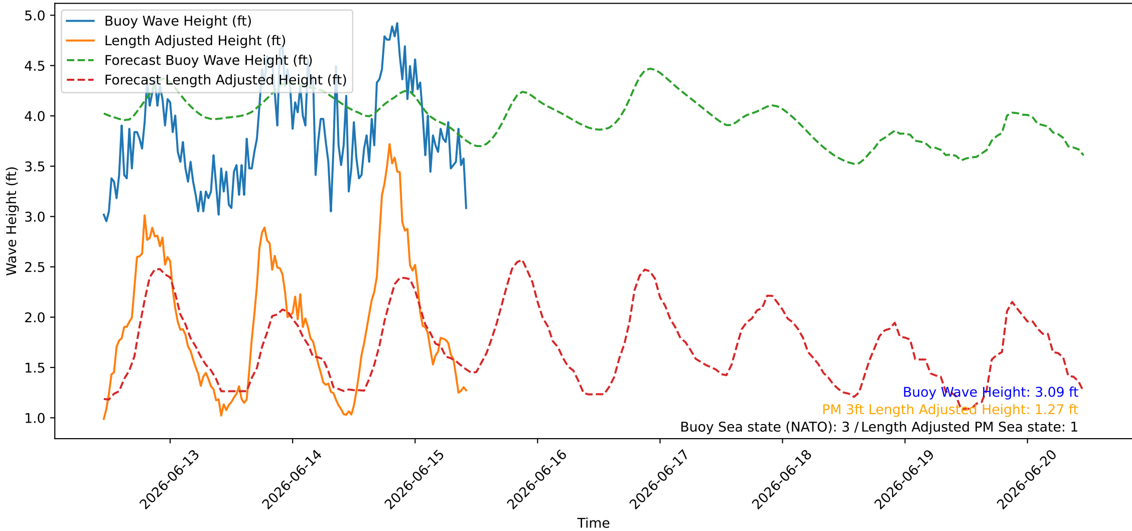
Wave Heights over Time for Green Beach at 2026-06-15 11:01:08
