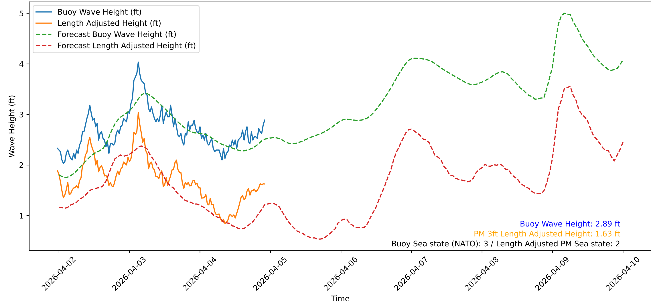
Wave Heights over Time for Oceanside Harbor at 2026-04-04 23:30:33
