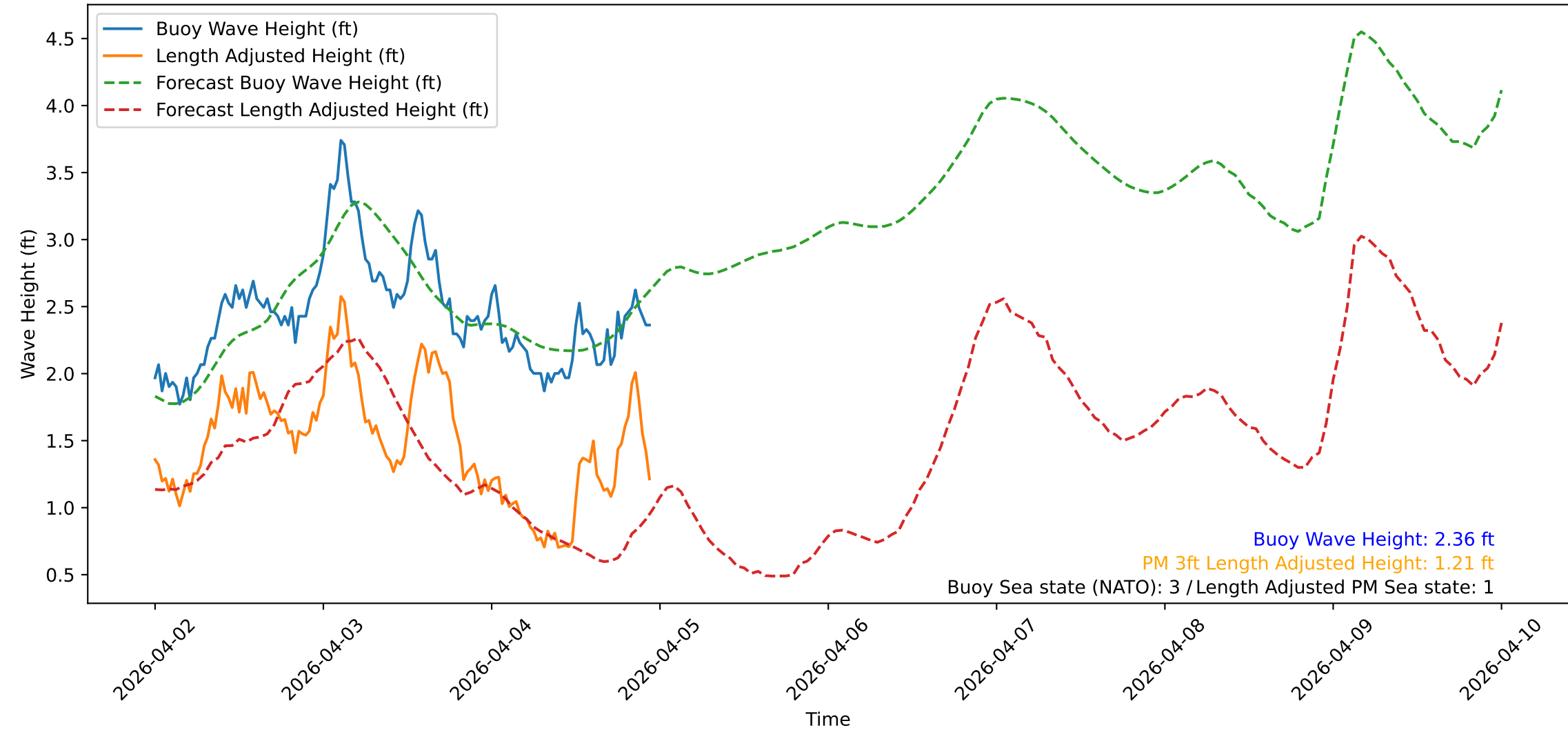
Wave Heights over Time for Red Beach at 2026-04-04 23:30:50
