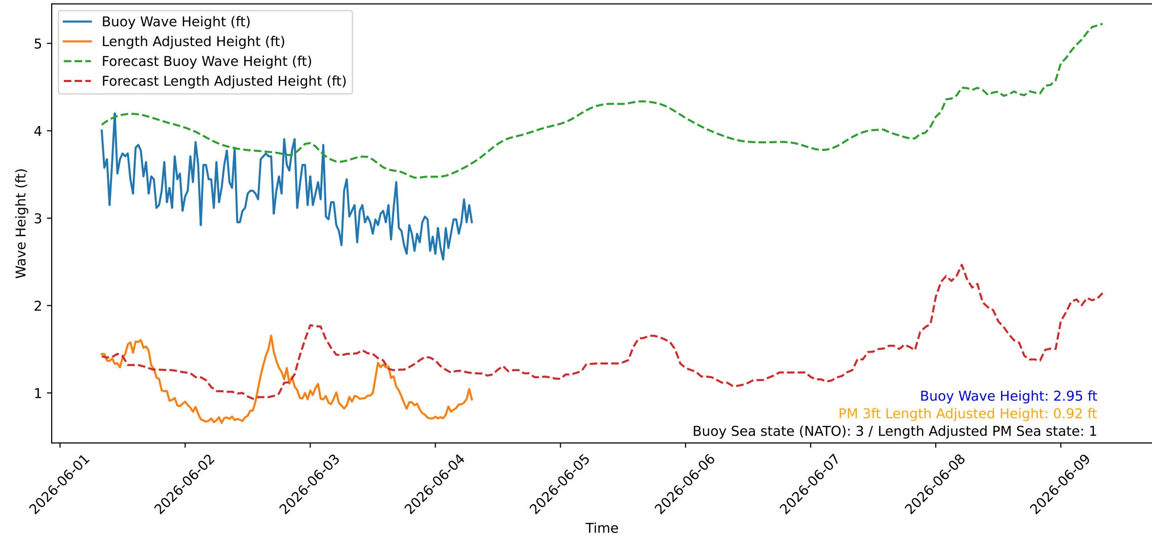
Wave Heights over Time for Red Beach at 2026-06-04 07:50:47
