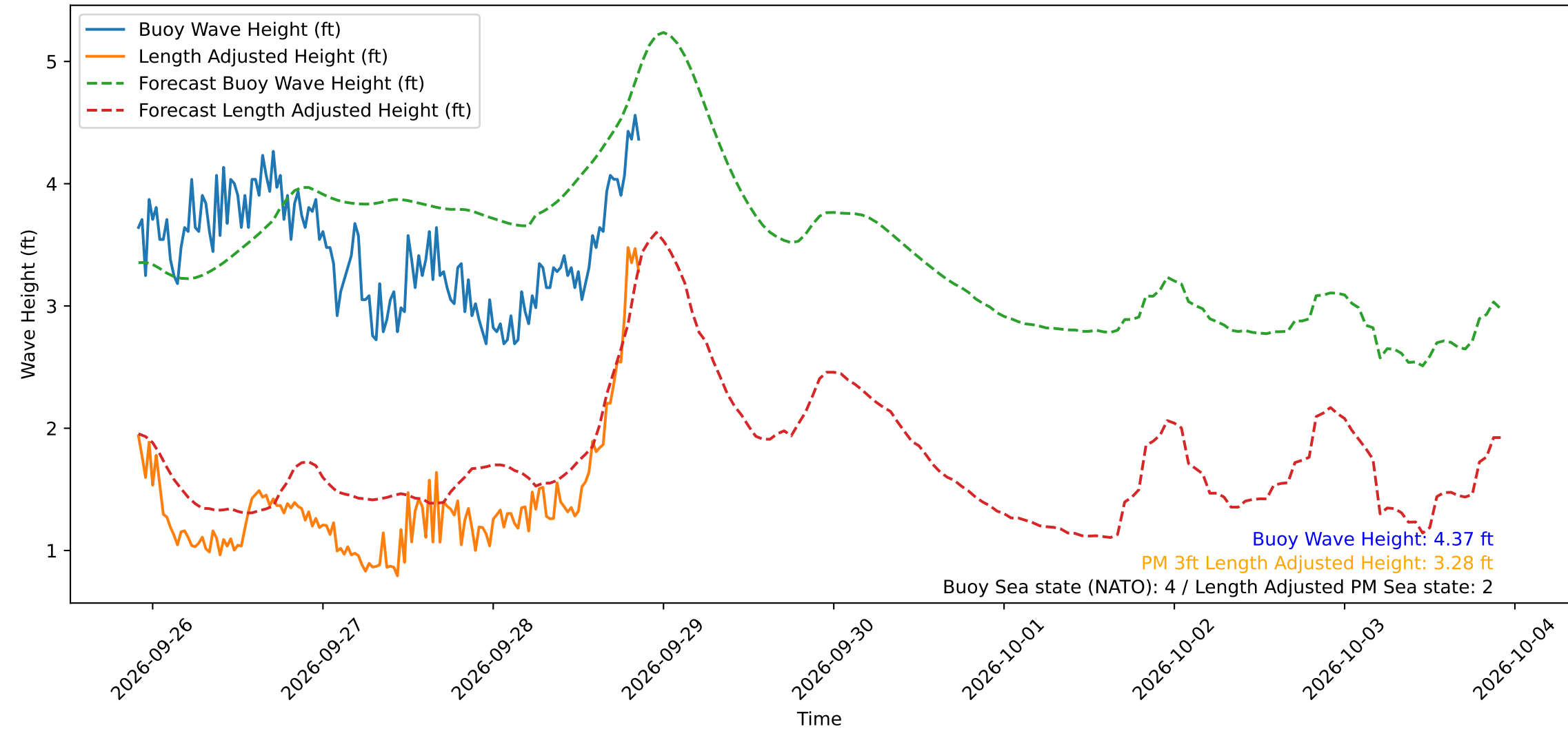
Wave Heights over Time for Green Beach at 2026-09-28 21:31:13
