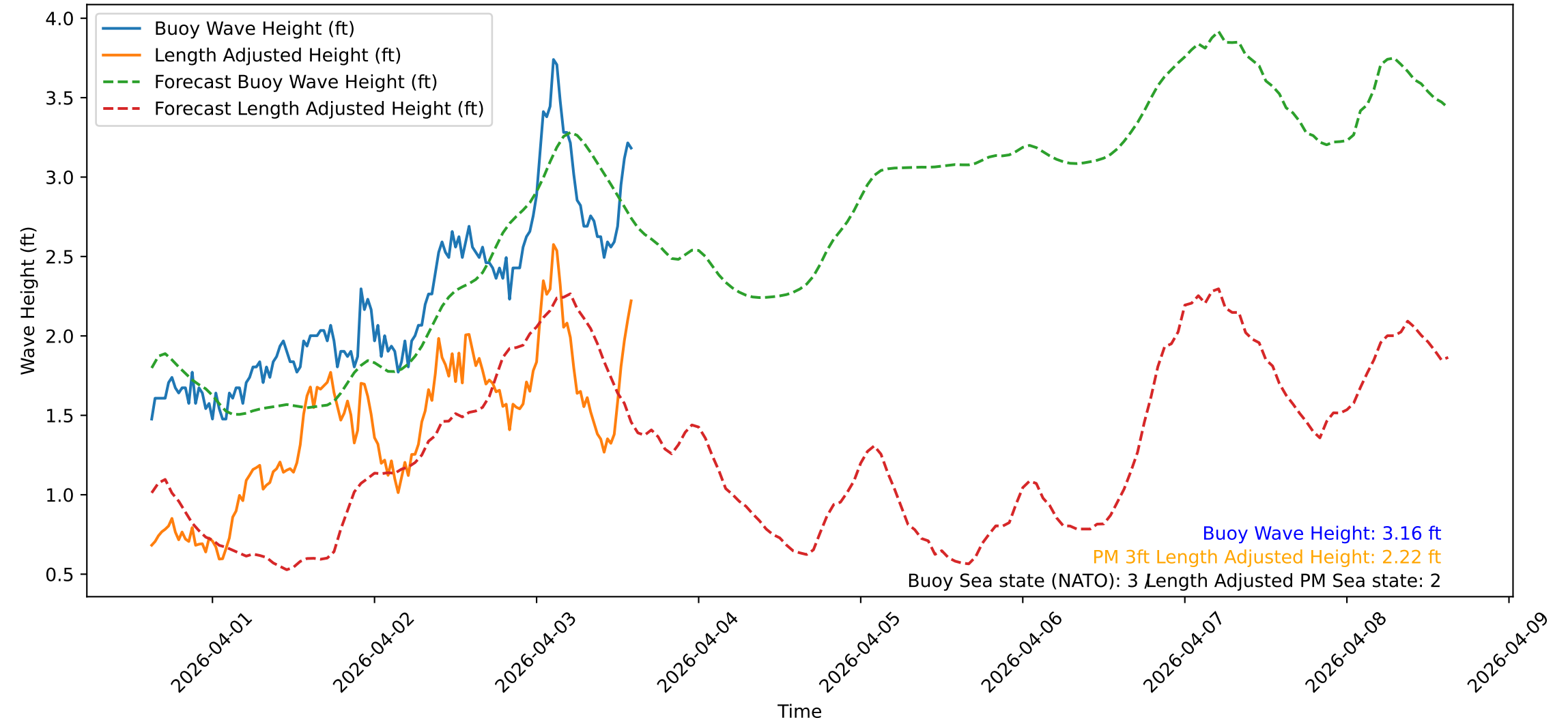
Wave Heights over Time for Red Beach at 2026-04-03 14:40:48
