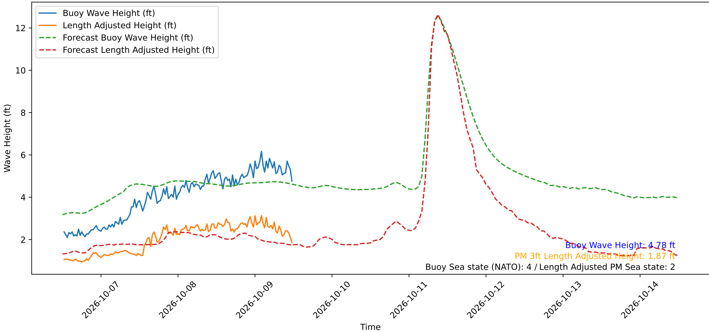
Wave Heights over Time for Green Beach at 2026-10-09 12:11:11
