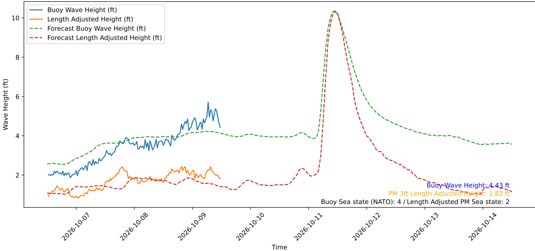
Wave Heights over Time for Red Beach at 2026-10-09 12:10:49
