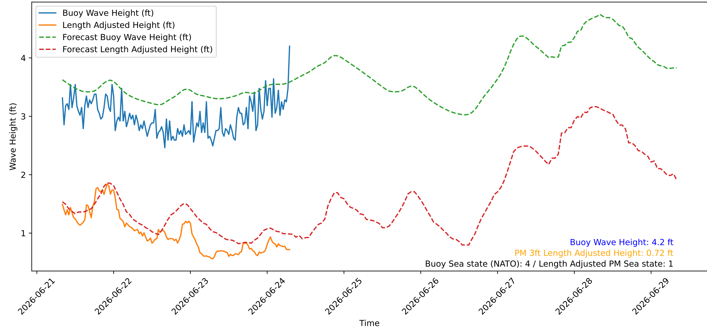
Wave Heights over Time for Green Beach at 2026-06-24 08:01:08
