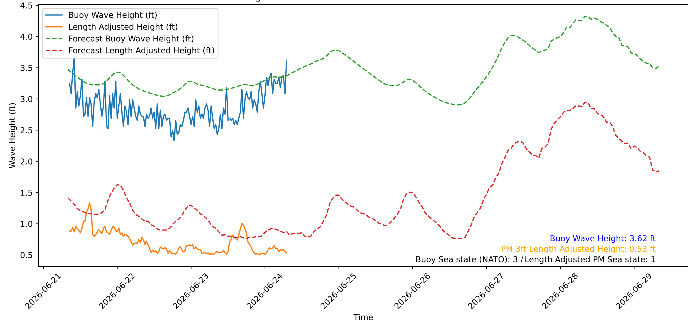
Wave Heights over Time for Red Beach at 2026-06-24 08:00:45
