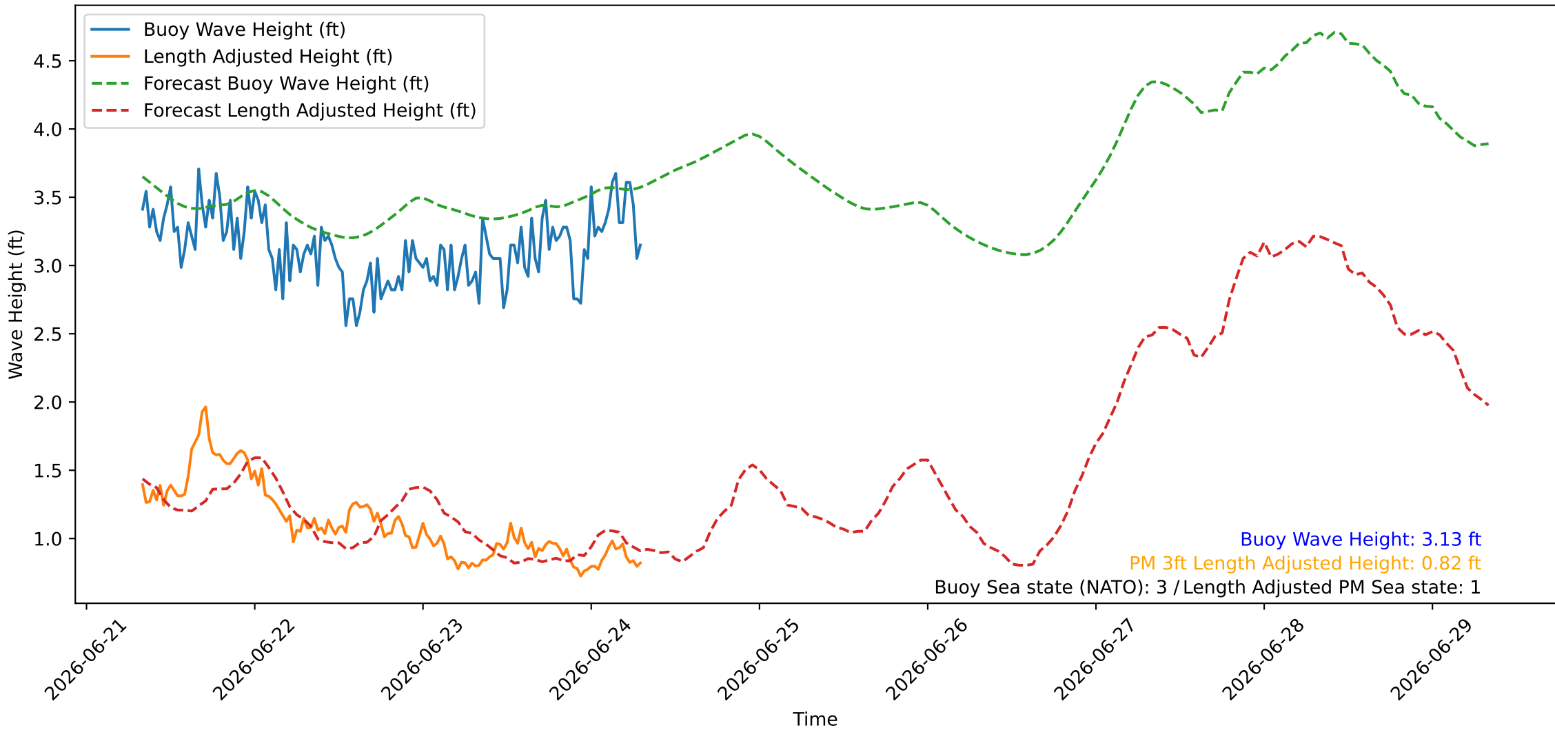
Wave Heights over Time for Oceanside Harbor at 2026-06-24 08:00:26
