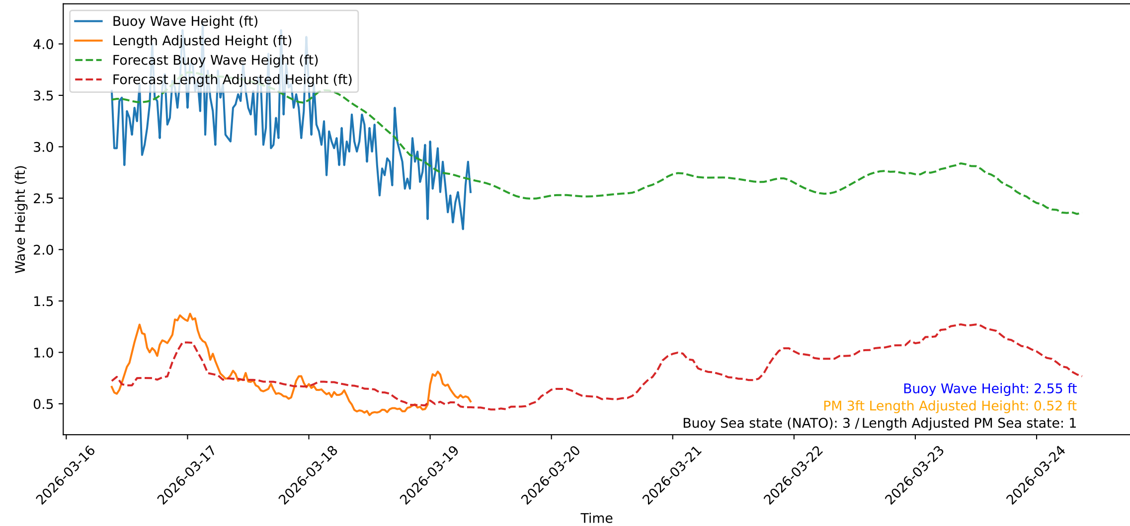
Wave Heights over Time for Green Beach at 2026-03-19 09:01:09
