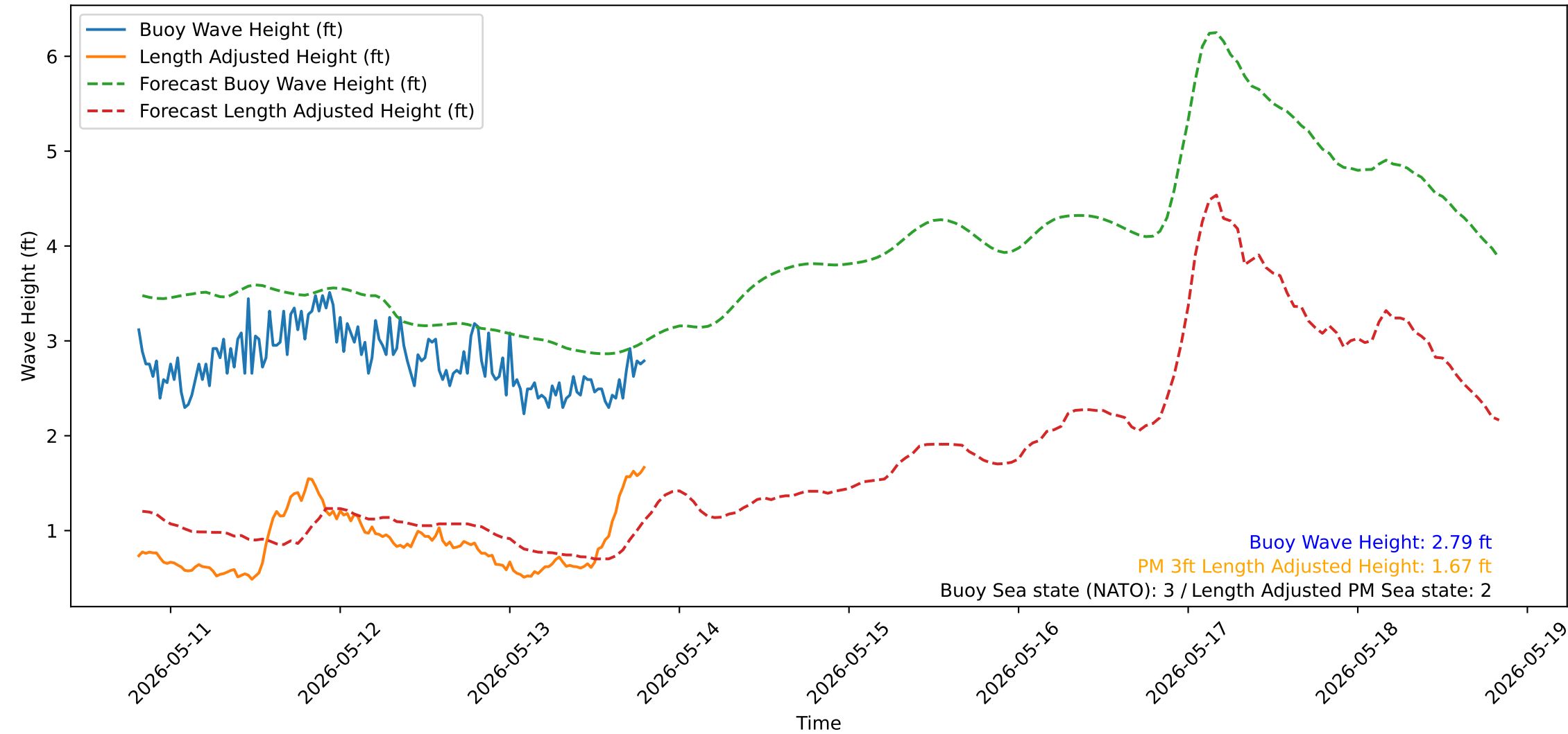
Wave Heights over Time for Green Beach at 2026-05-13 19:41:14
