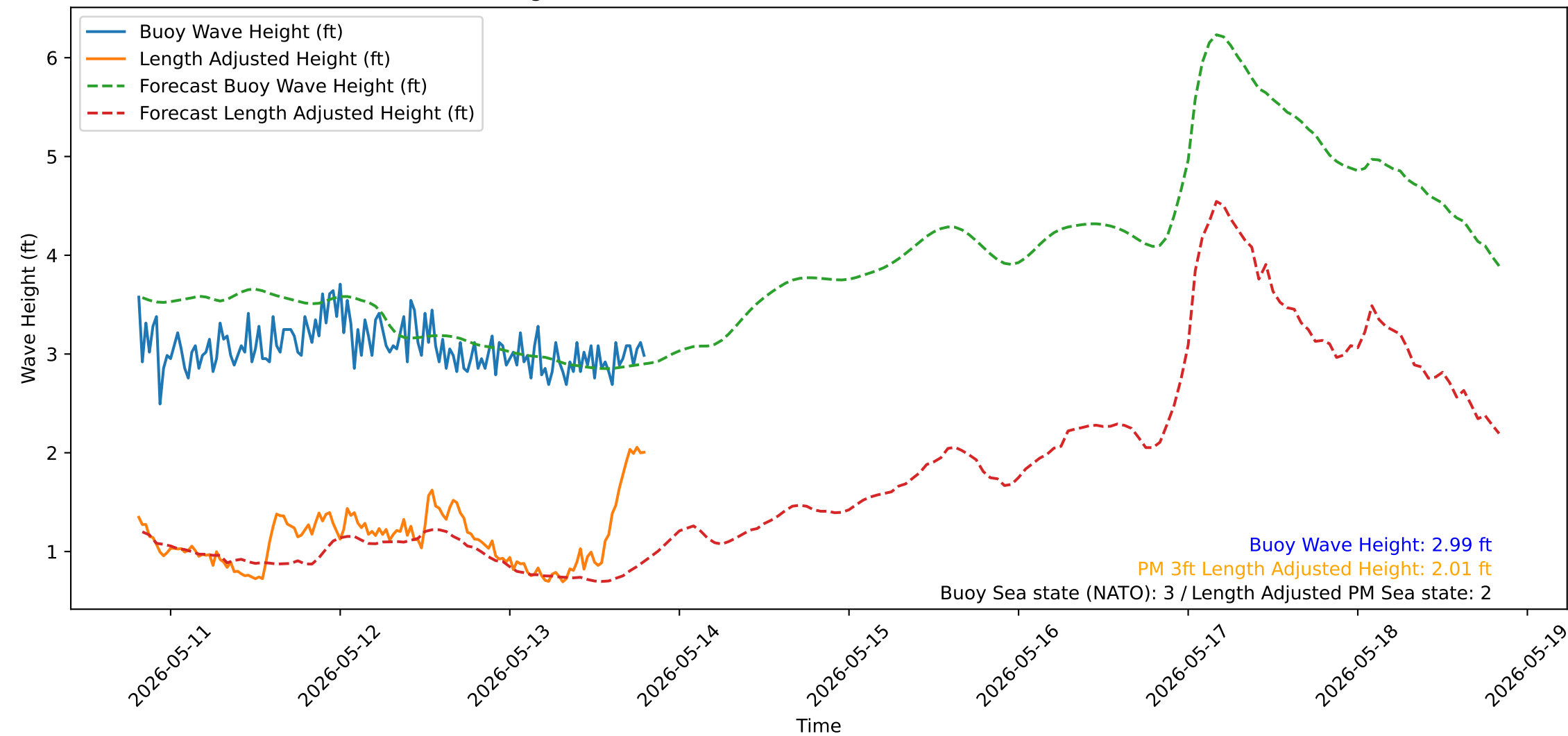
Wave Heights over Time for Oceanside Harbor at 2026-05-13 19:40:32
