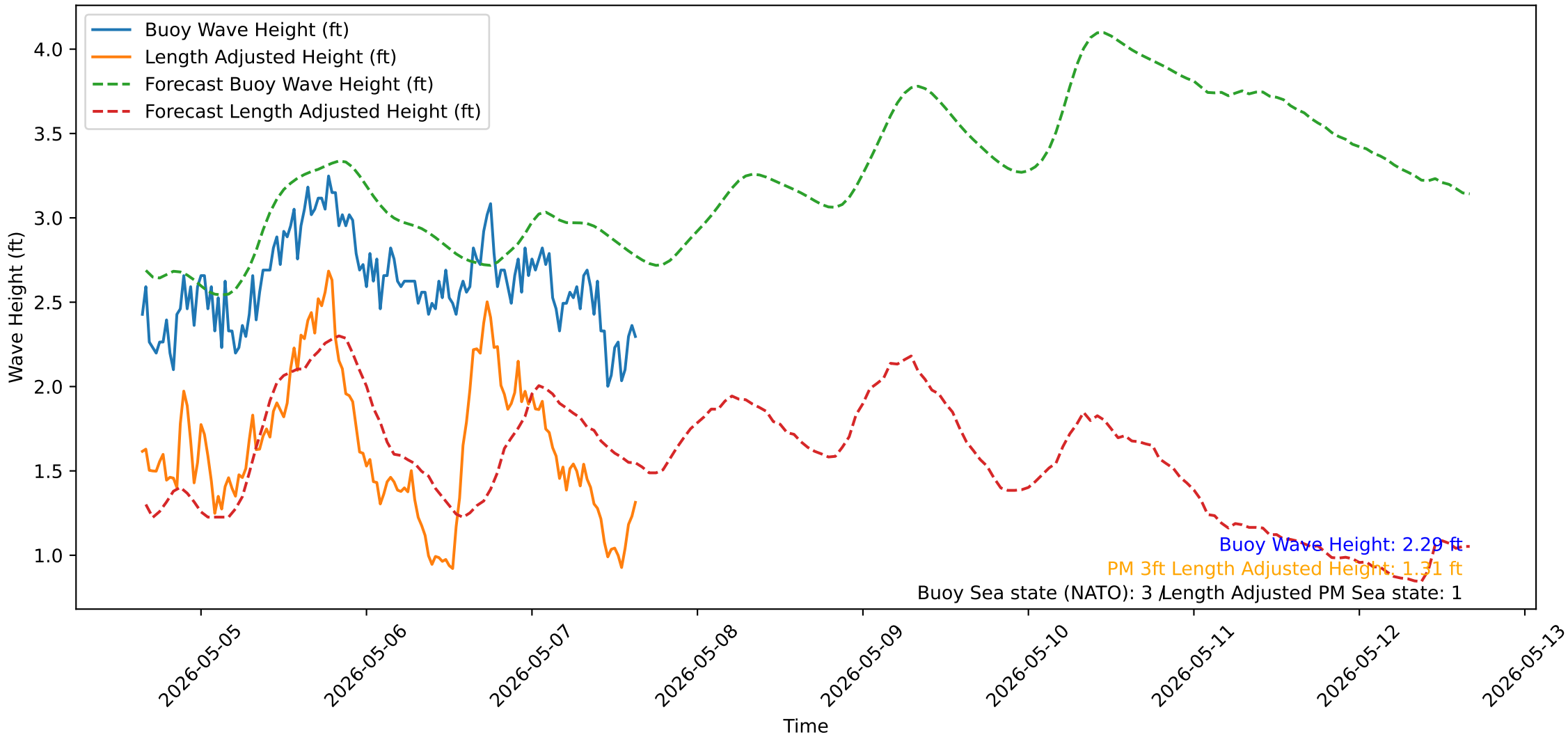
Wave Heights over Time for Oceanside Harbor at 2026-05-07 15:40:31
