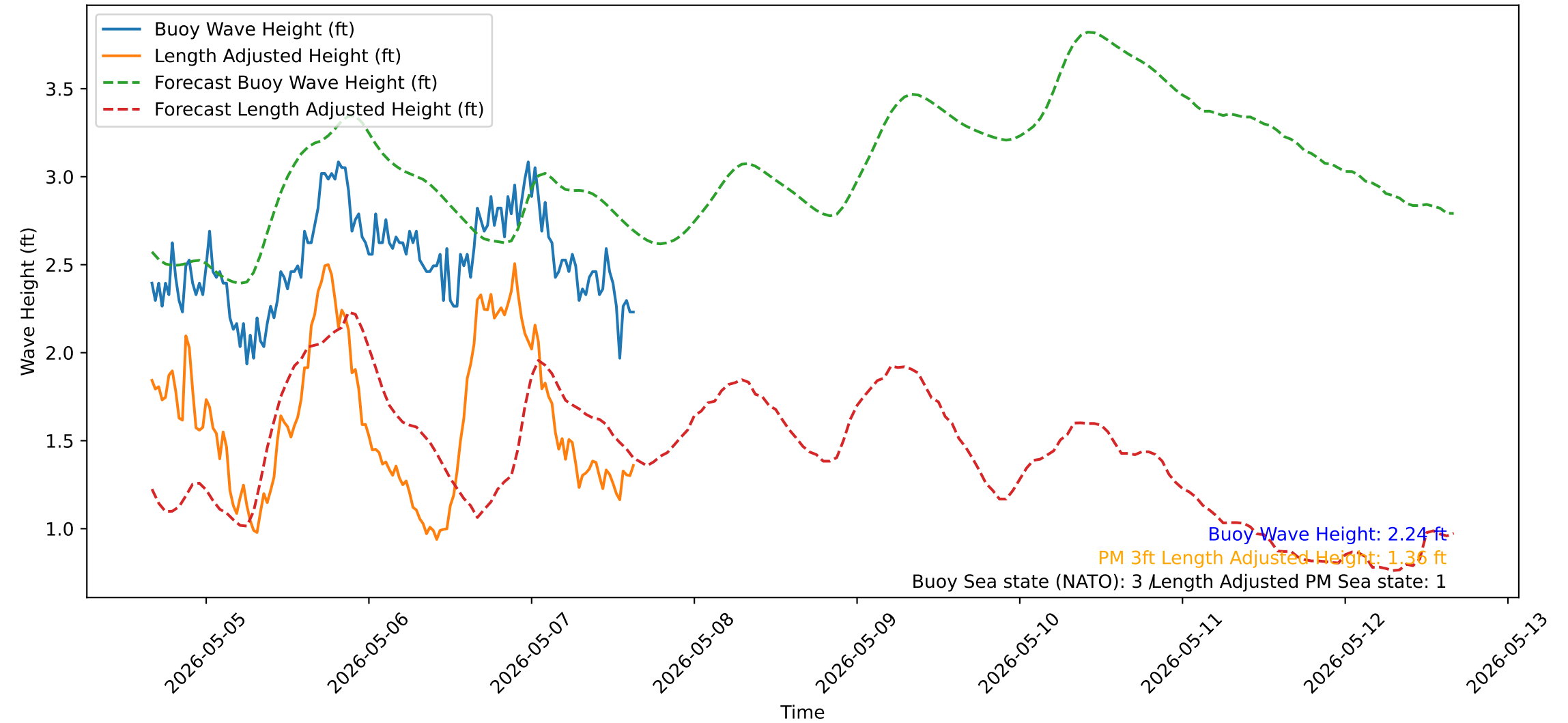
Wave Heights over Time for Red Beach at 2026-05-07 15:40:50
