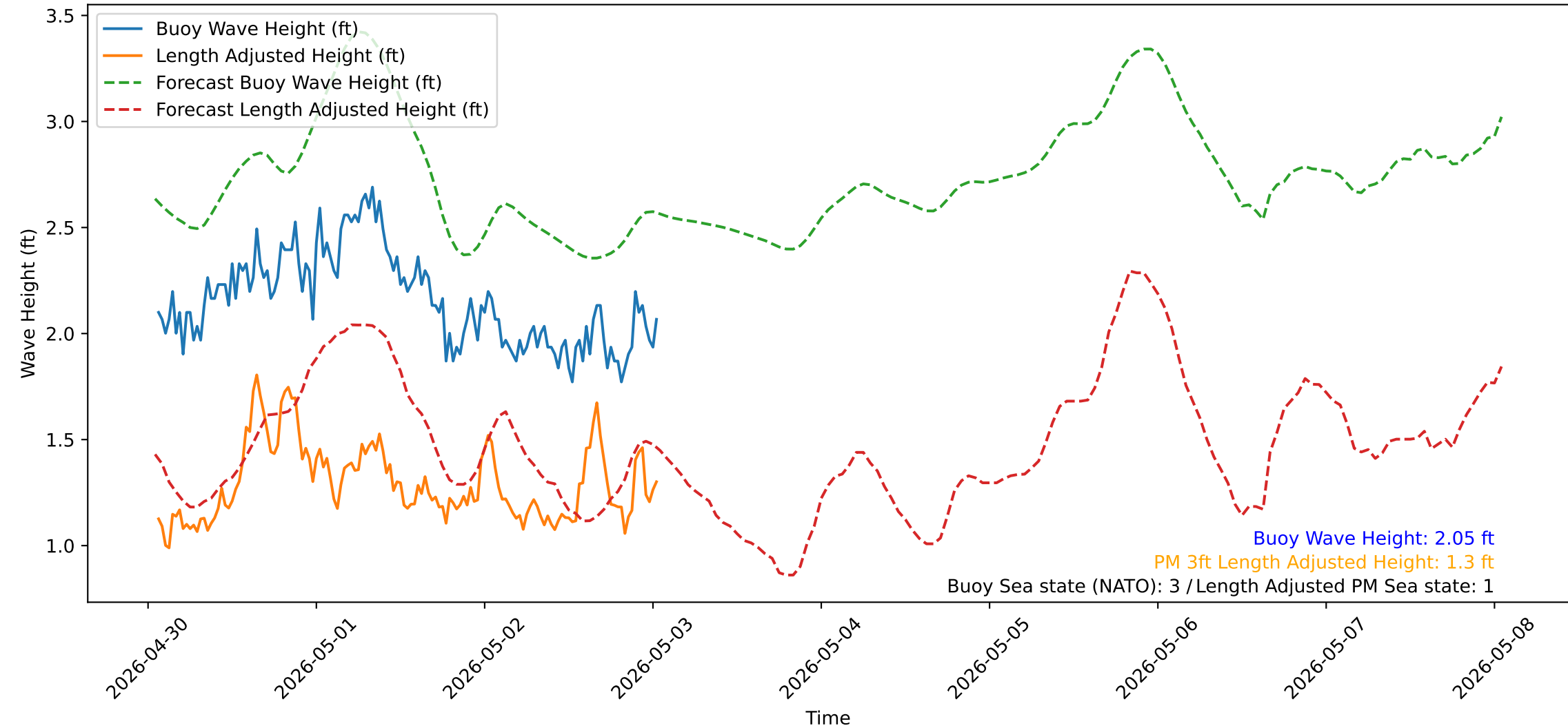
Wave Heights over Time for Oceanside Harbor at 2026-05-03 01:20:31
