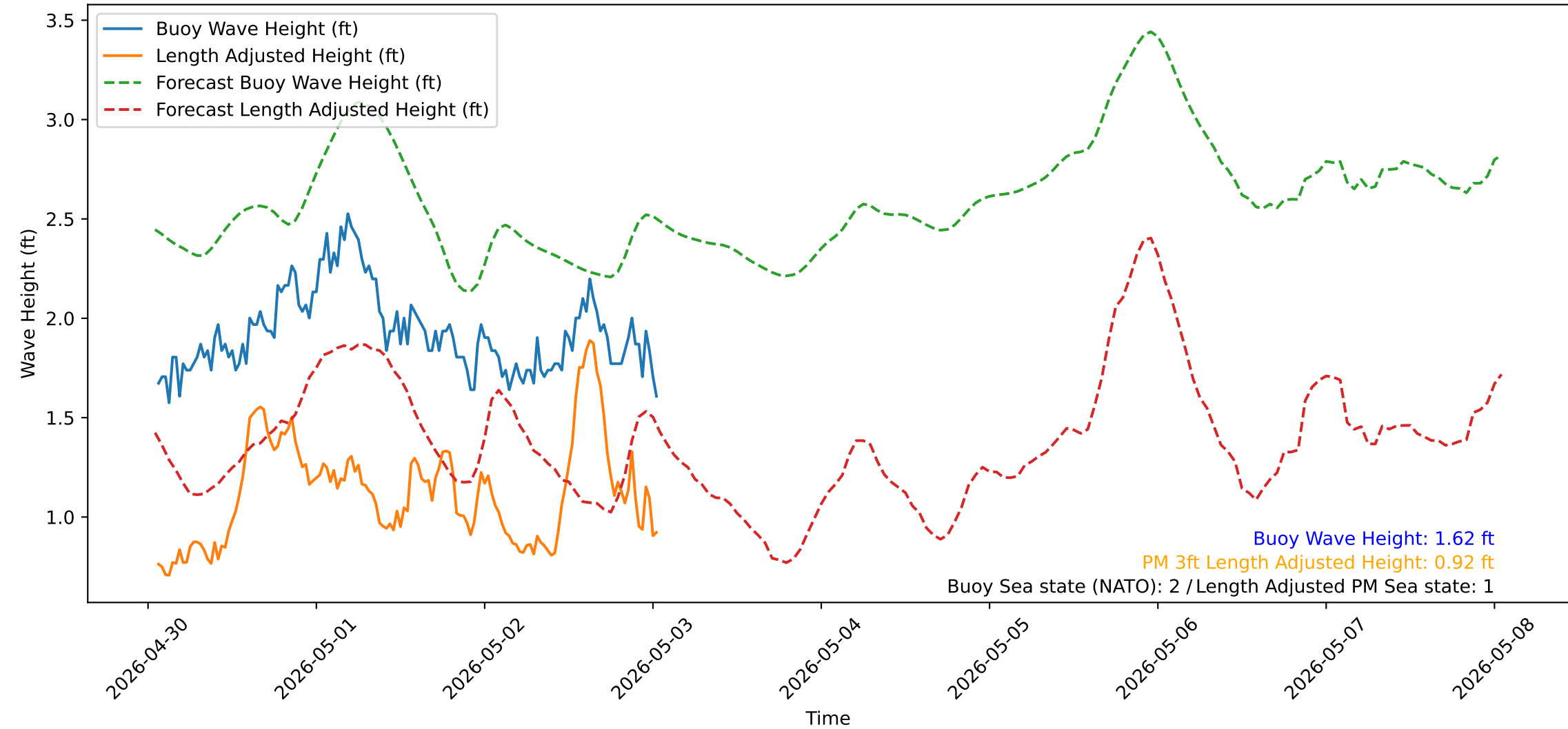
Wave Heights over Time for Red Beach at 2026-05-03 01:20:51
