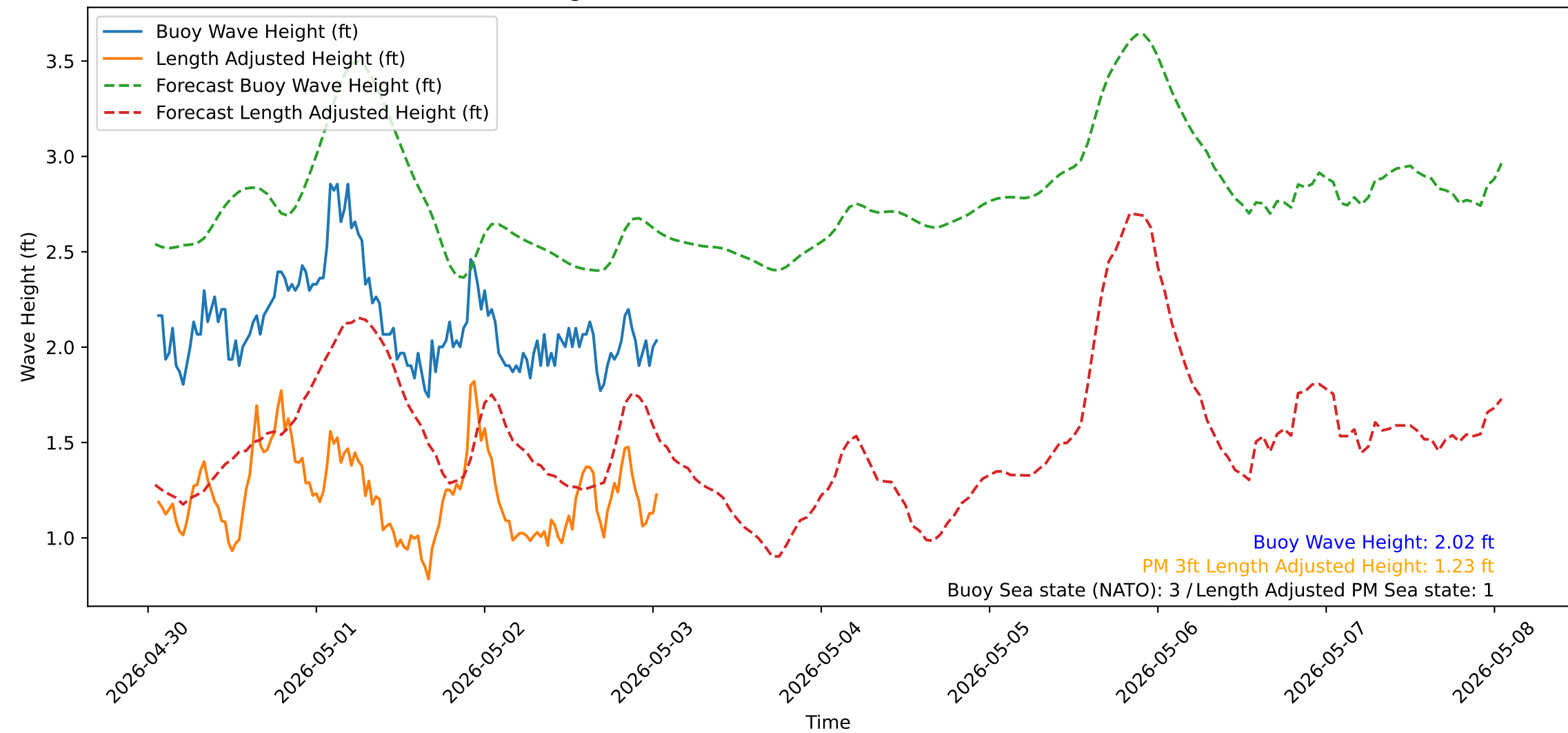
Wave Heights over Time for Green Beach at 2026-05-03 01:21:13
