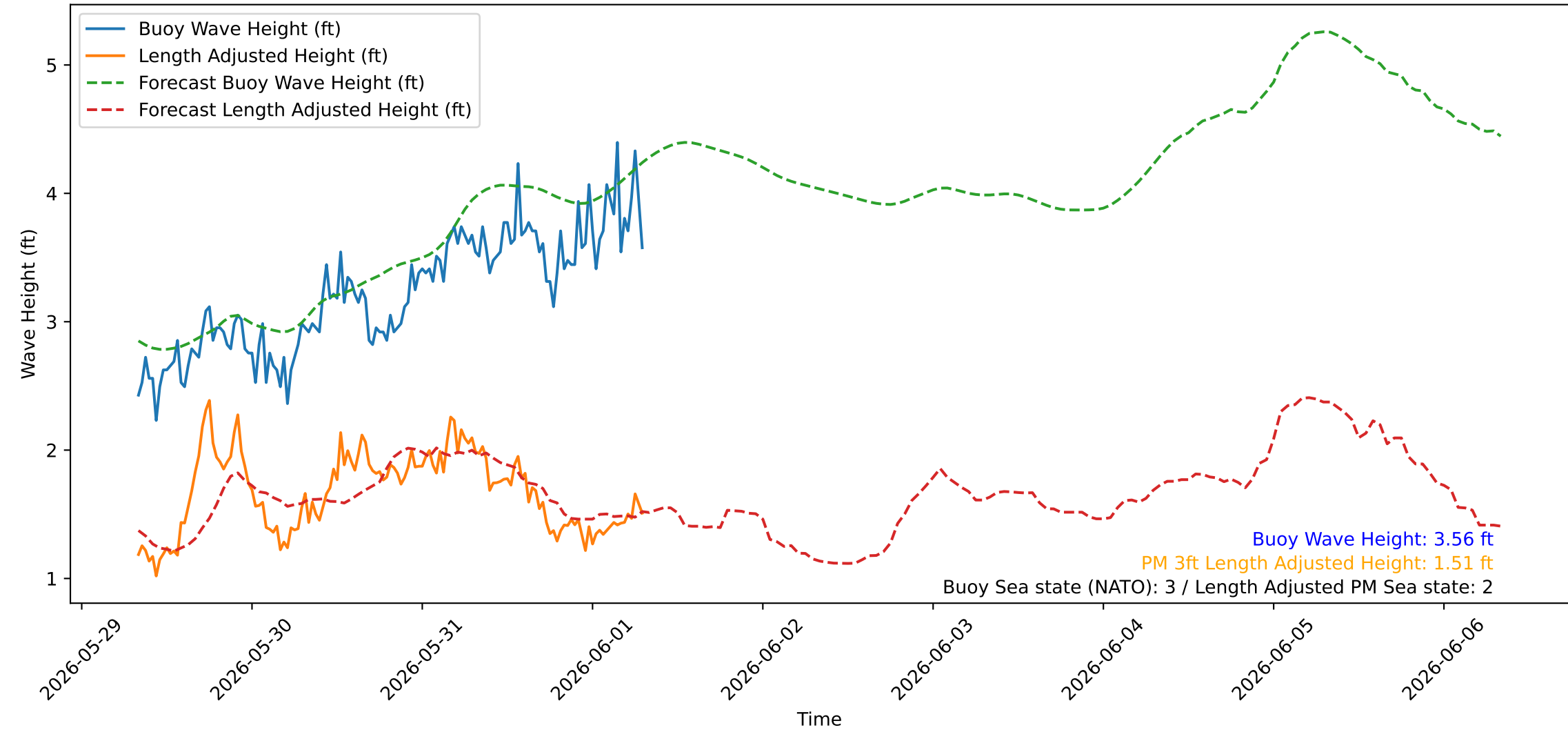
Wave Heights over Time for Oceanside Harbor at 2026-06-01 07:50:26
