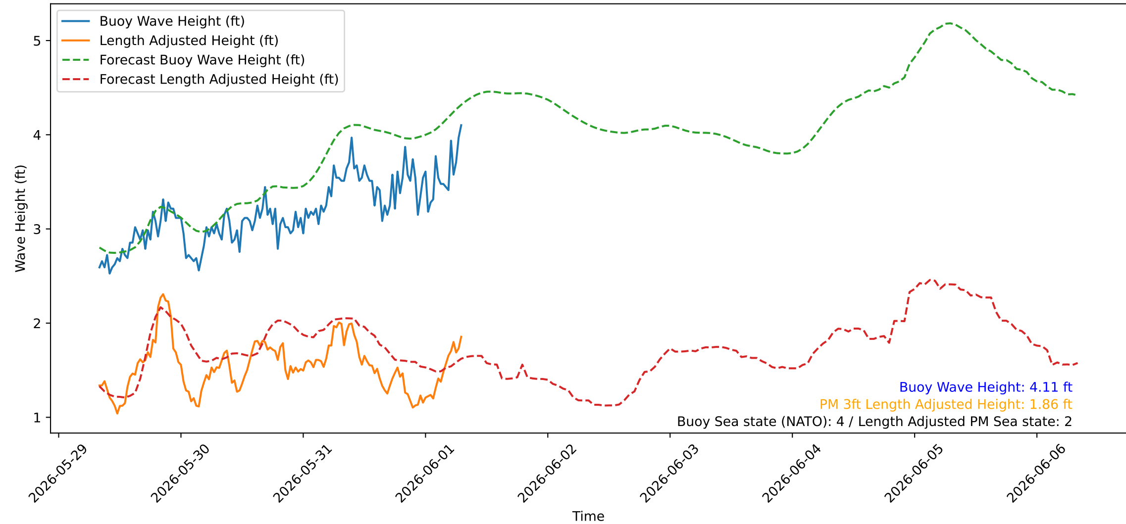
Wave Heights over Time for Green Beach at 2026-06-01 07:51:09
