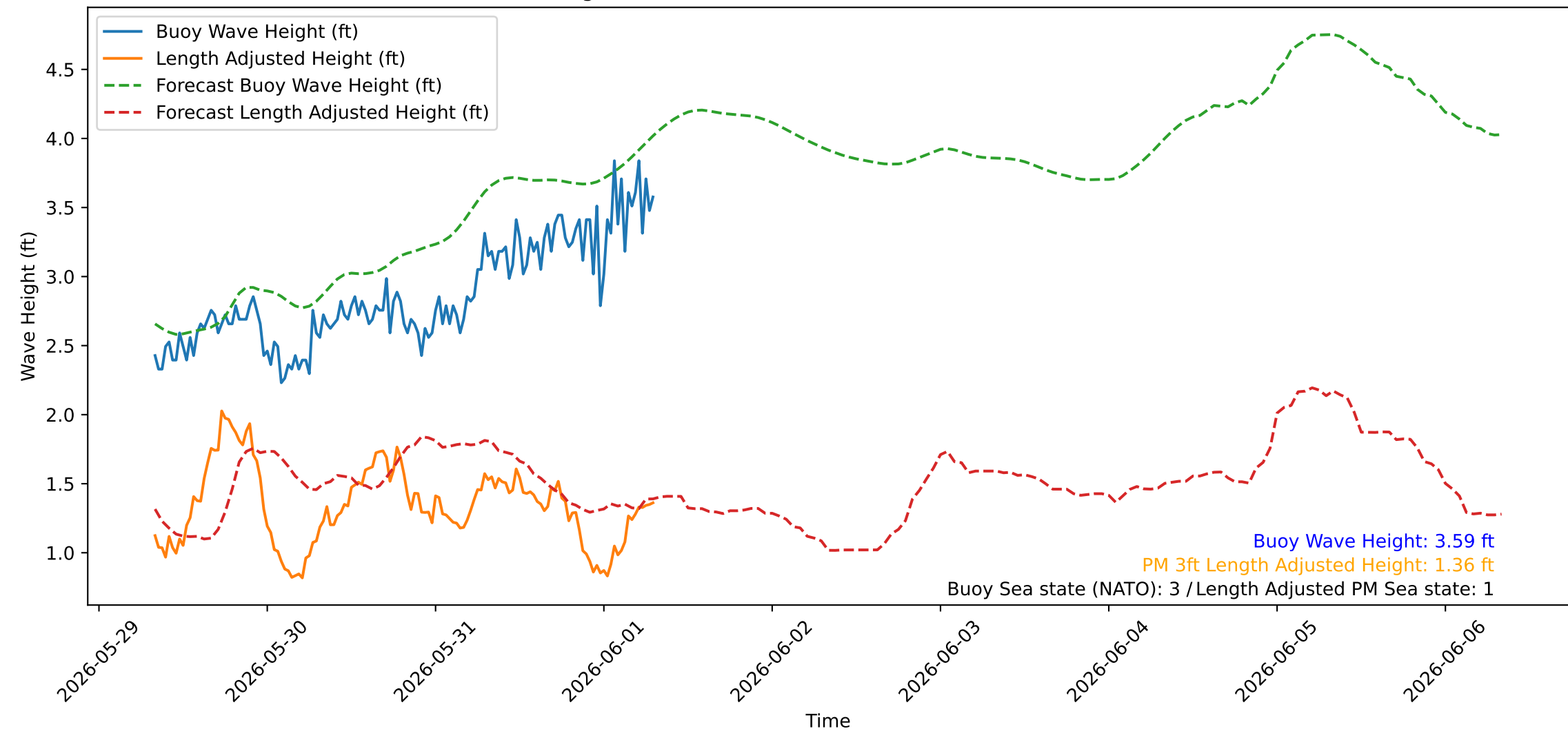
Wave Heights over Time for Red Beach at 2026-06-01 07:50:47
