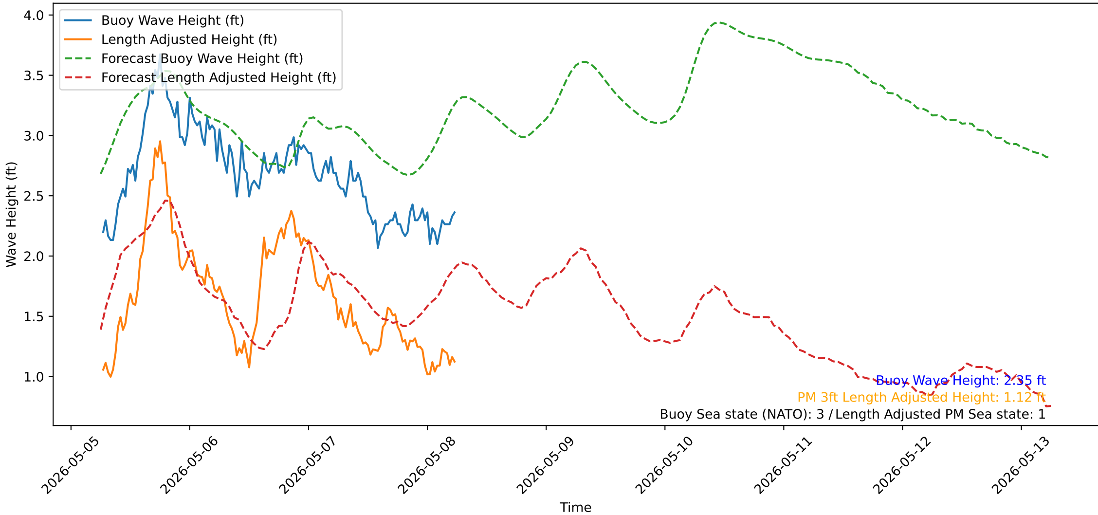
Wave Heights over Time for Green Beach at 2026-05-08 06:21:15
