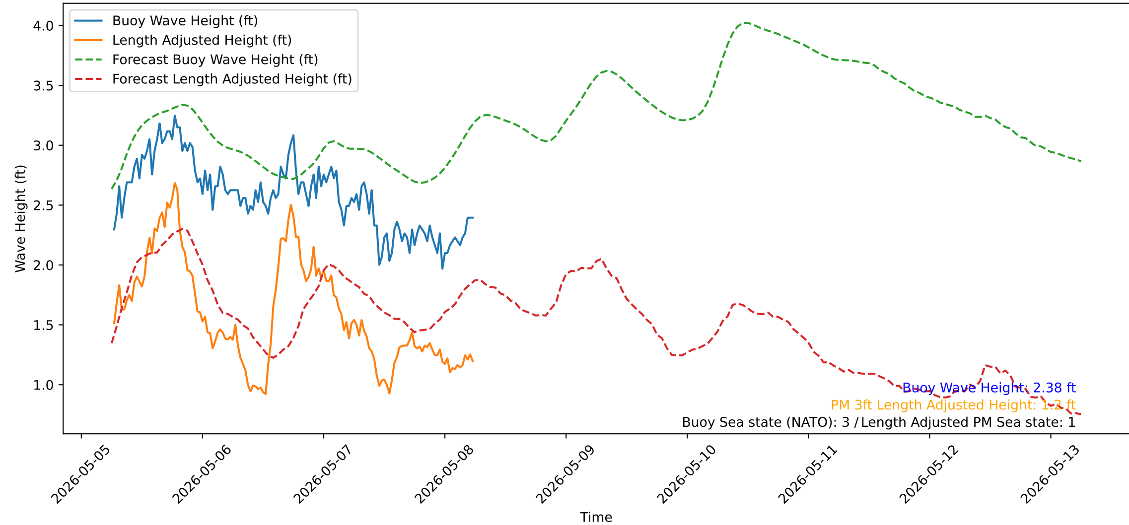
Wave Heights over Time for Oceanside Harbor at 2026-05-08 06:20:32
