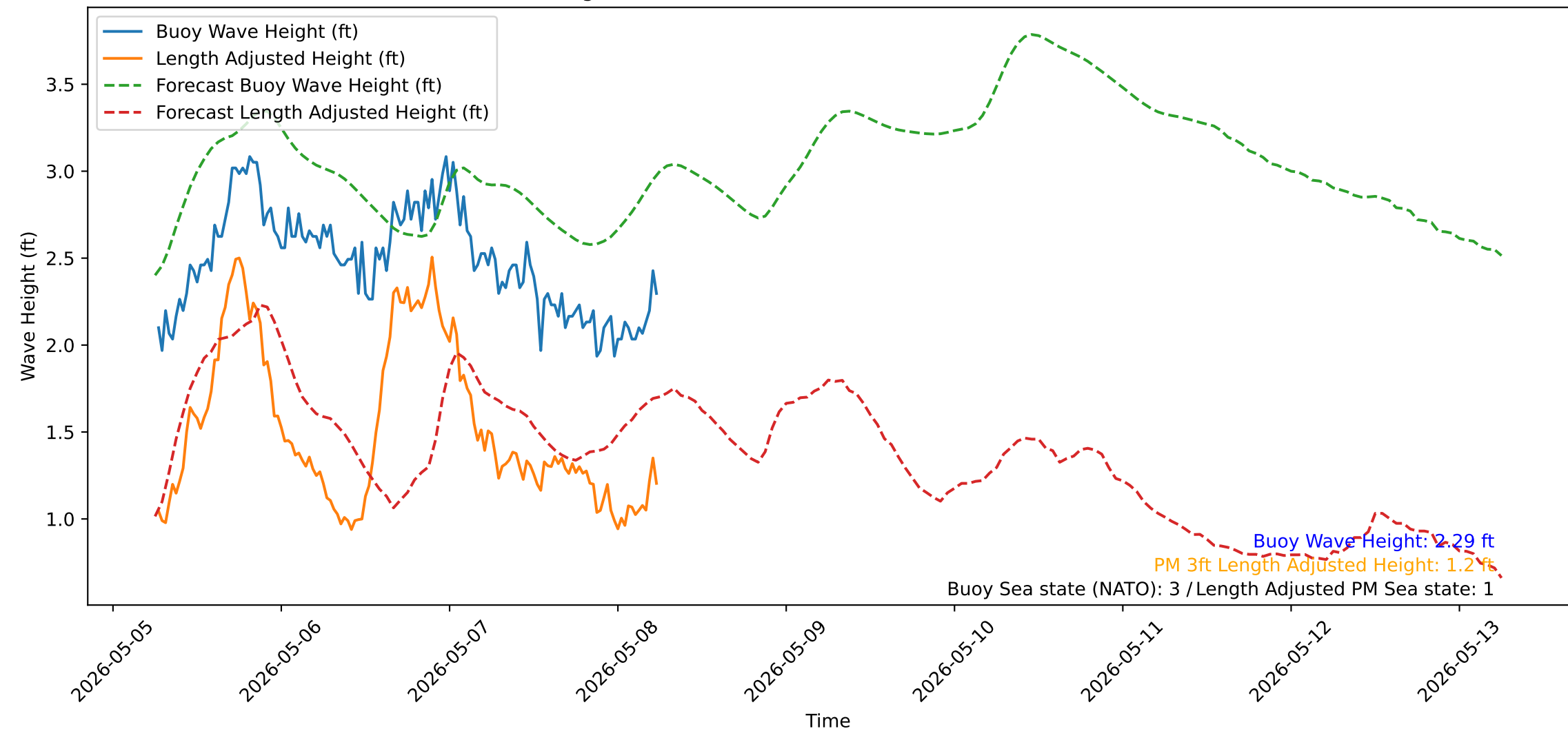
Wave Heights over Time for Red Beach at 2026-05-08 06:20:52
