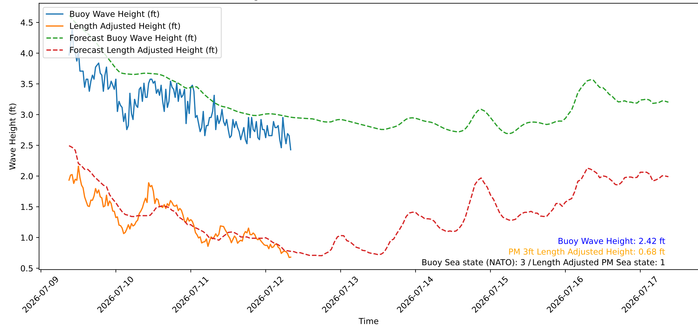
Wave Heights over Time for Green Beach at 2026-07-12 08:51:09
