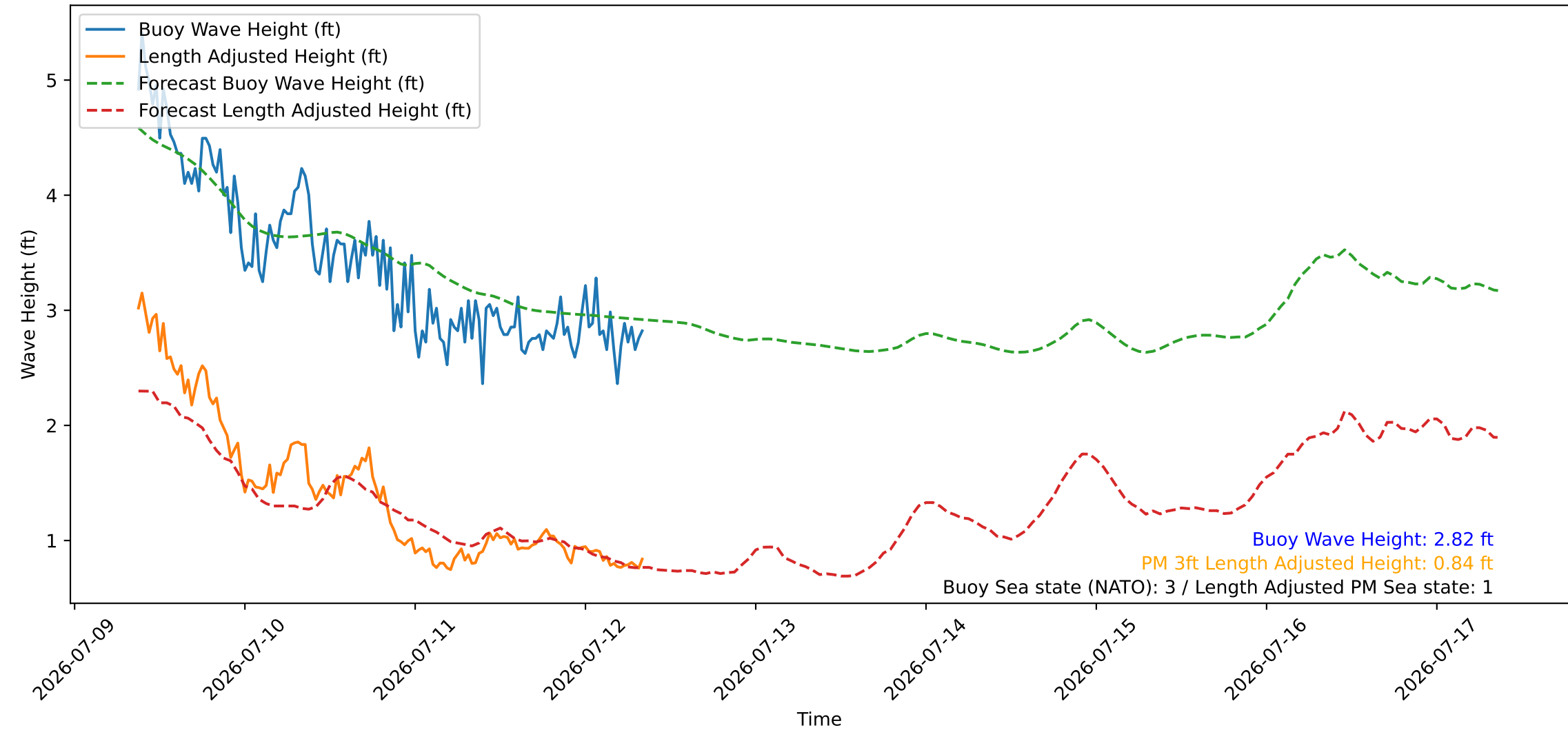
Wave Heights over Time for Oceanside Harbor at 2026-07-12 08:50:26
