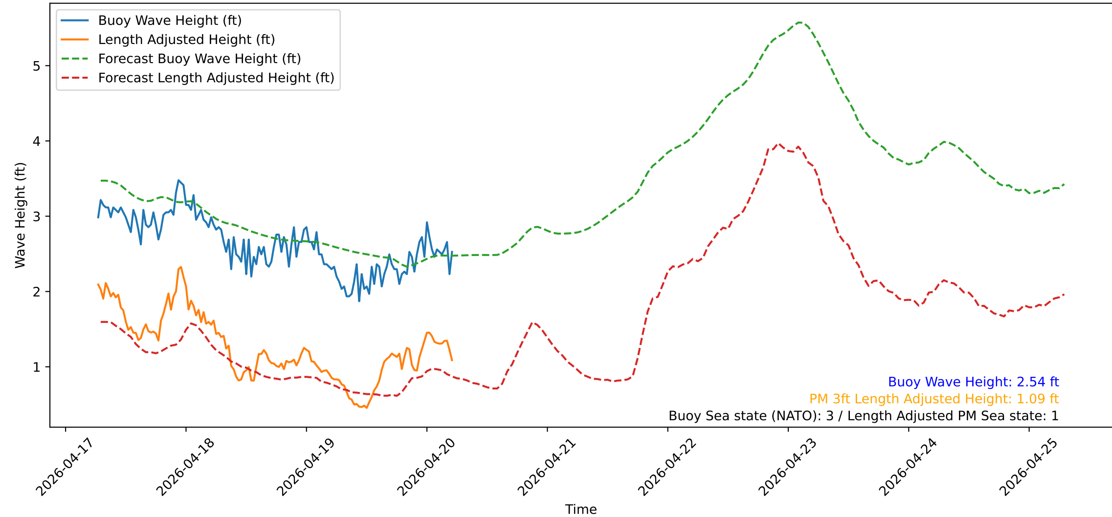
Wave Heights over Time for Green Beach at 2026-04-20 06:31:12
