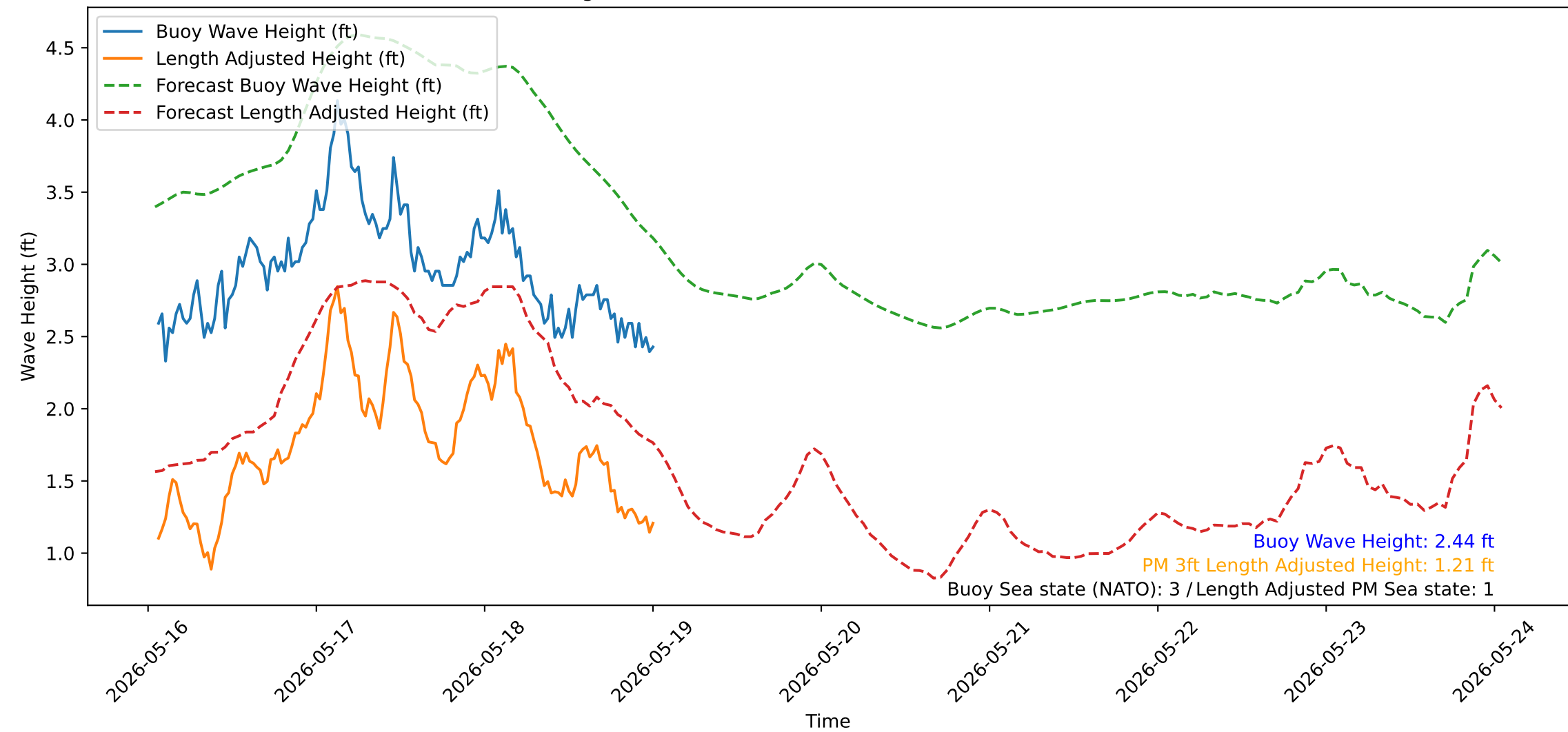
Wave Heights over Time for Red Beach at 2026-05-19 01:00:51
