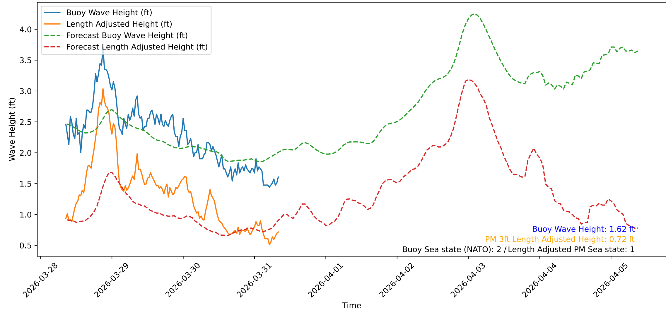
Wave Heights over Time for Green Beach at 2026-03-31 08:41:10
