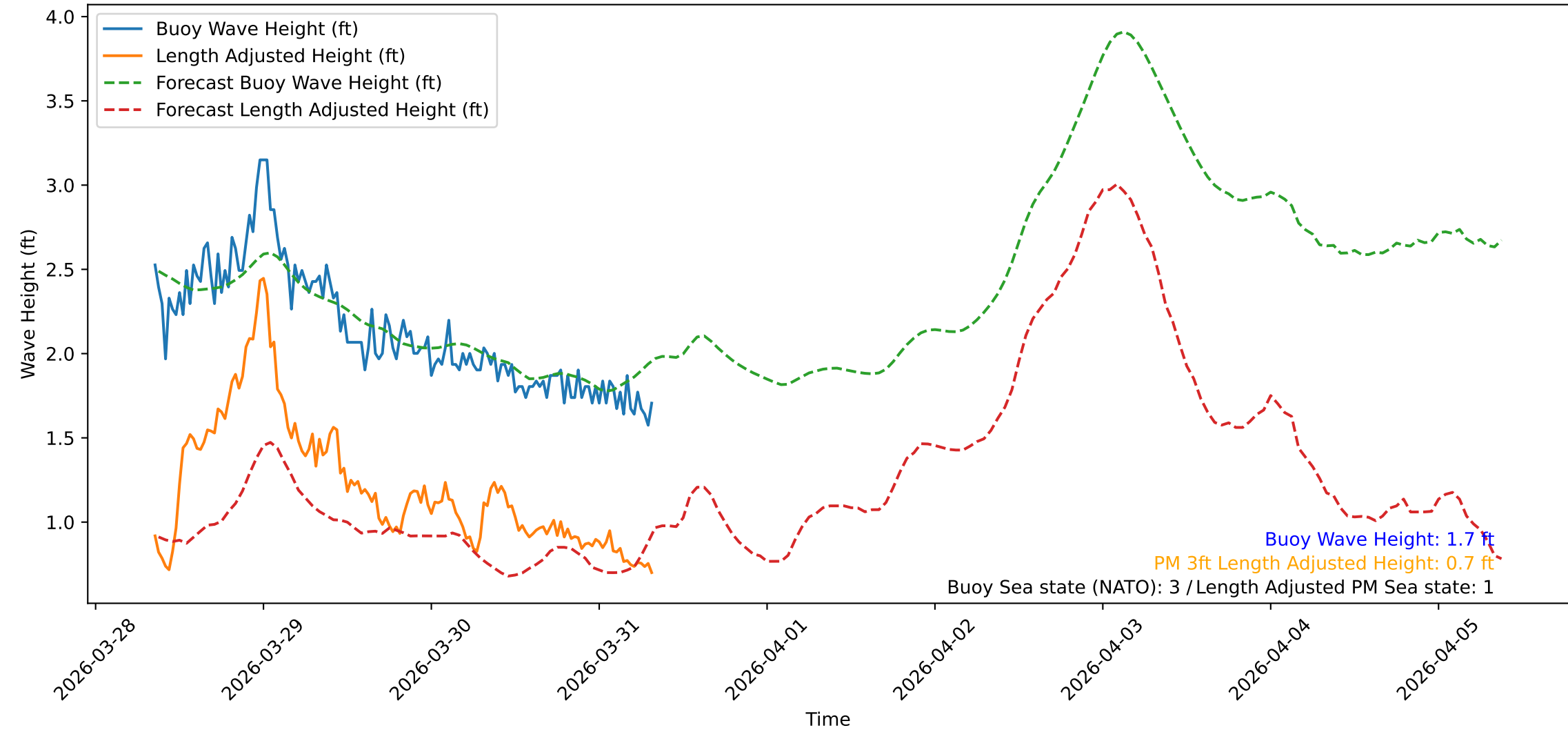
Wave Heights over Time for Oceanside Harbor at 2026-03-31 08:40:32
