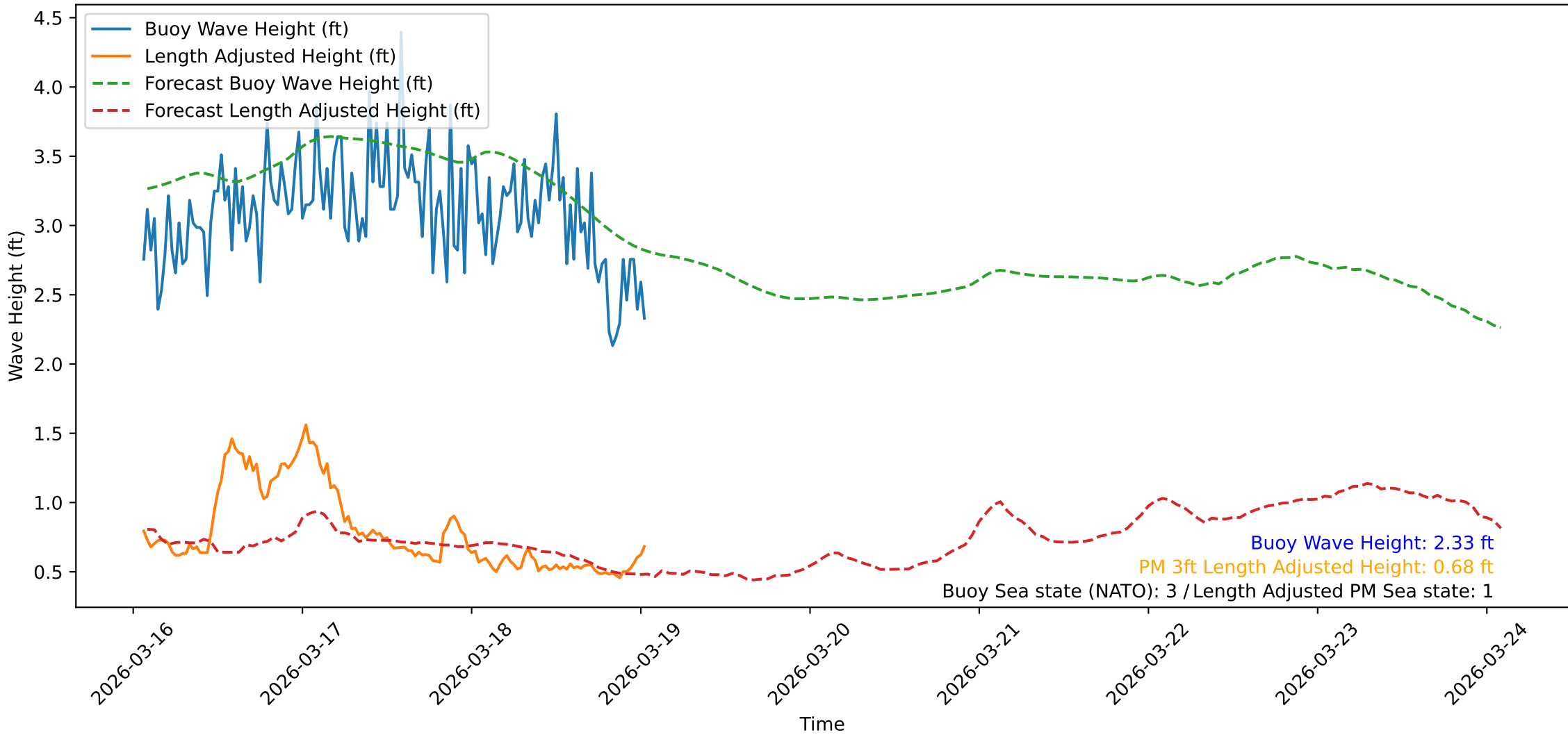
Wave Heights over Time for Oceanside Harbor at 2026-03-19 01:30:31
