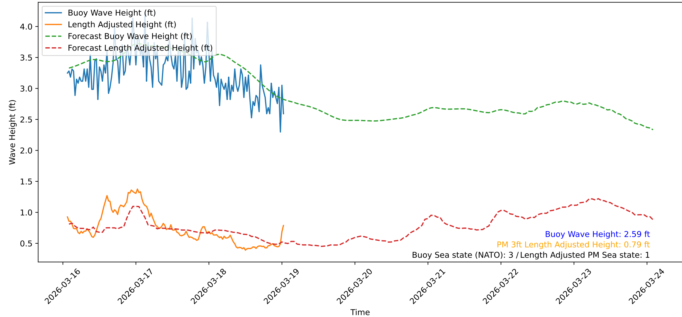
Wave Heights over Time for Green Beach at 2026-03-19 01:31:10
