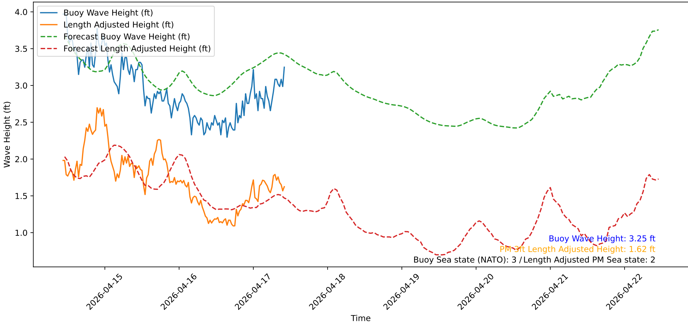
Wave Heights over Time for Oceanside Harbor at 2026-04-17 10:40:31
