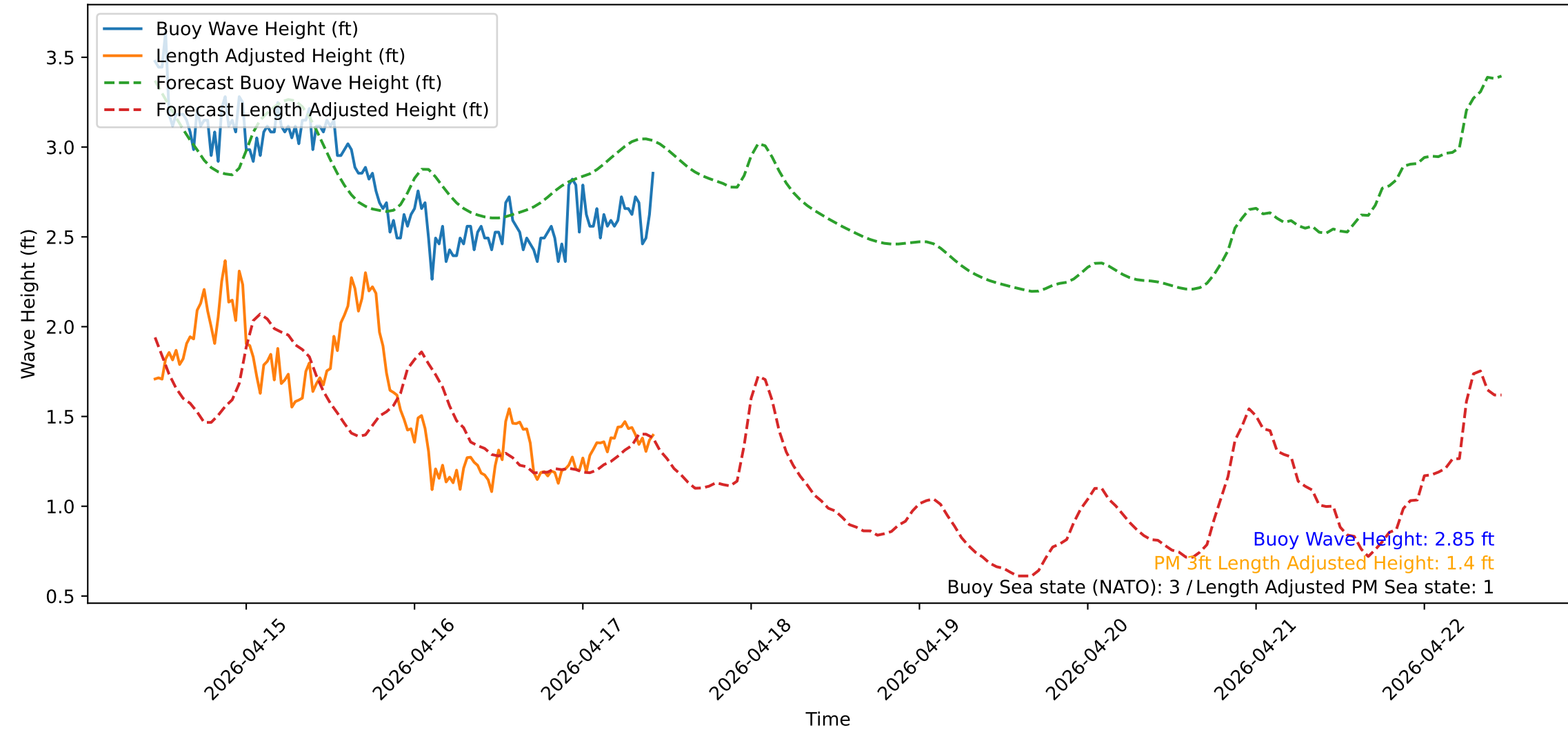
Wave Heights over Time for Red Beach at 2026-04-17 10:40:51
