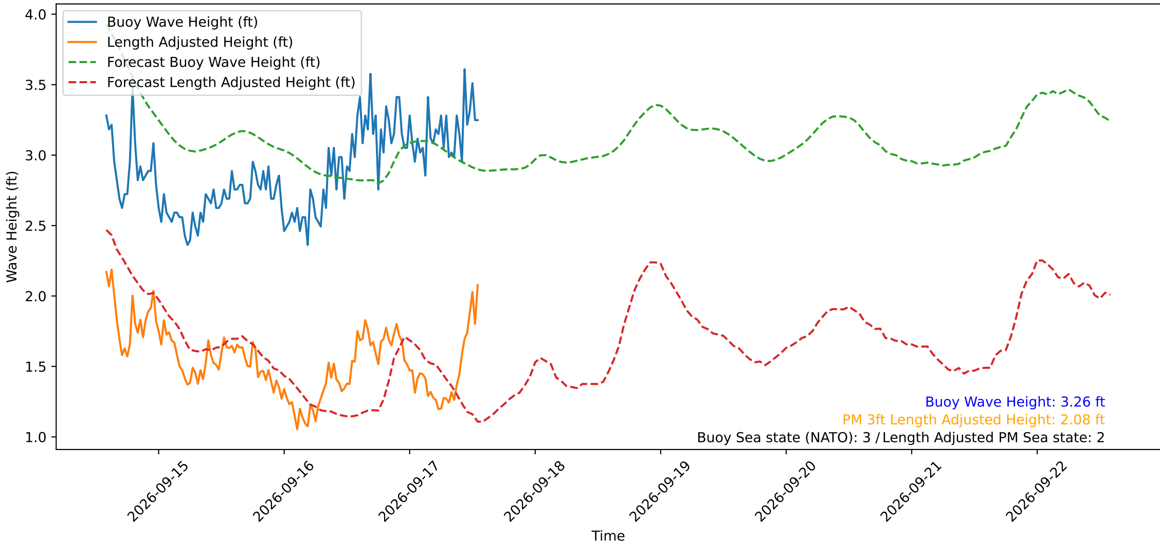
Wave Heights over Time for Oceanside Harbor at 2026-09-17 13:50:29
