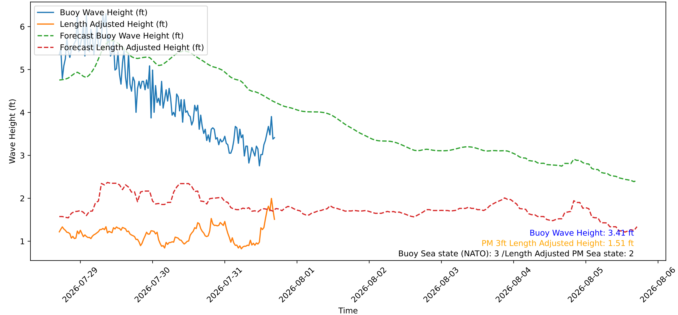
Wave Heights over Time for Green Beach at 2026-07-31 17:11:09
