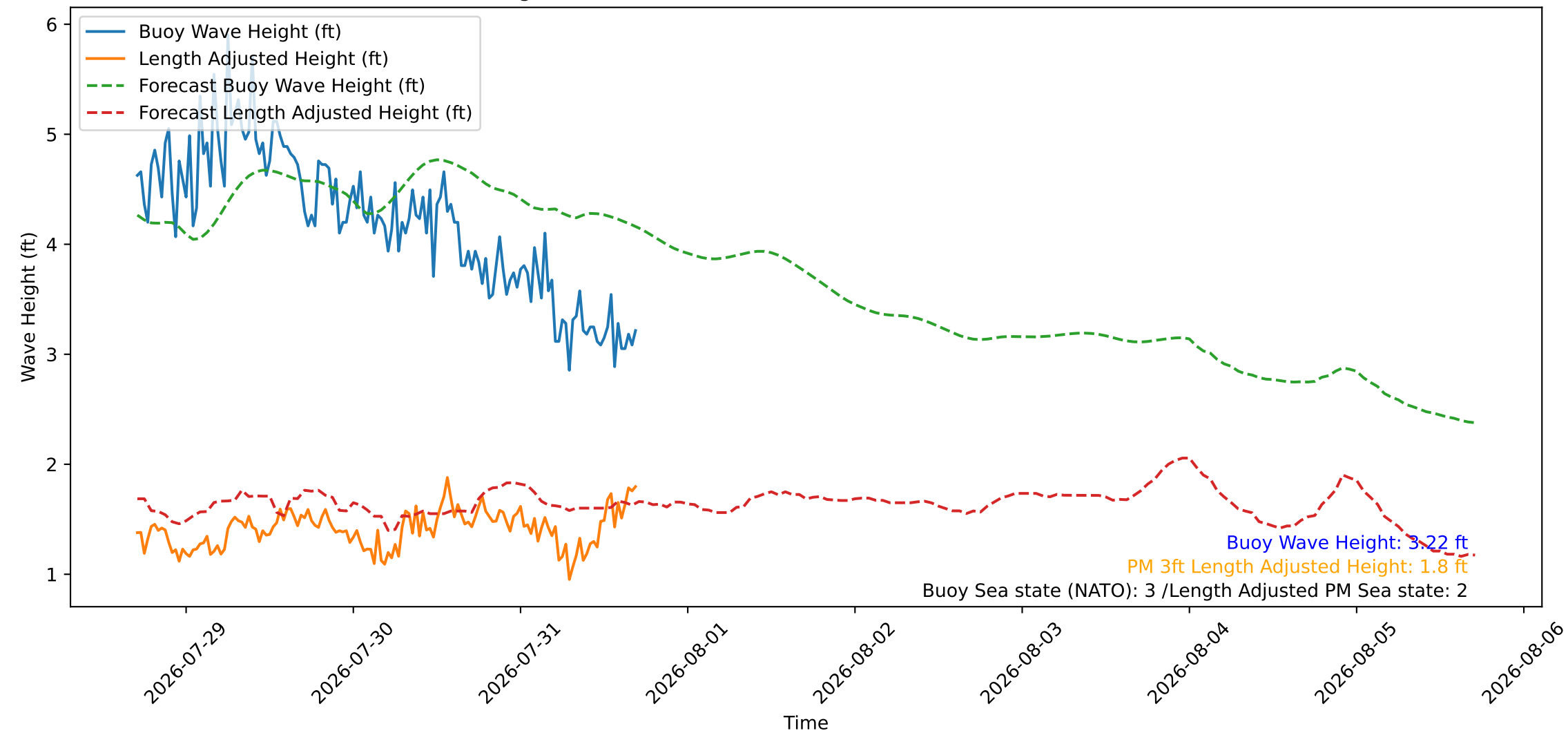
Wave Heights over Time for Oceanside Harbor at 2026-07-31 17:10:26
