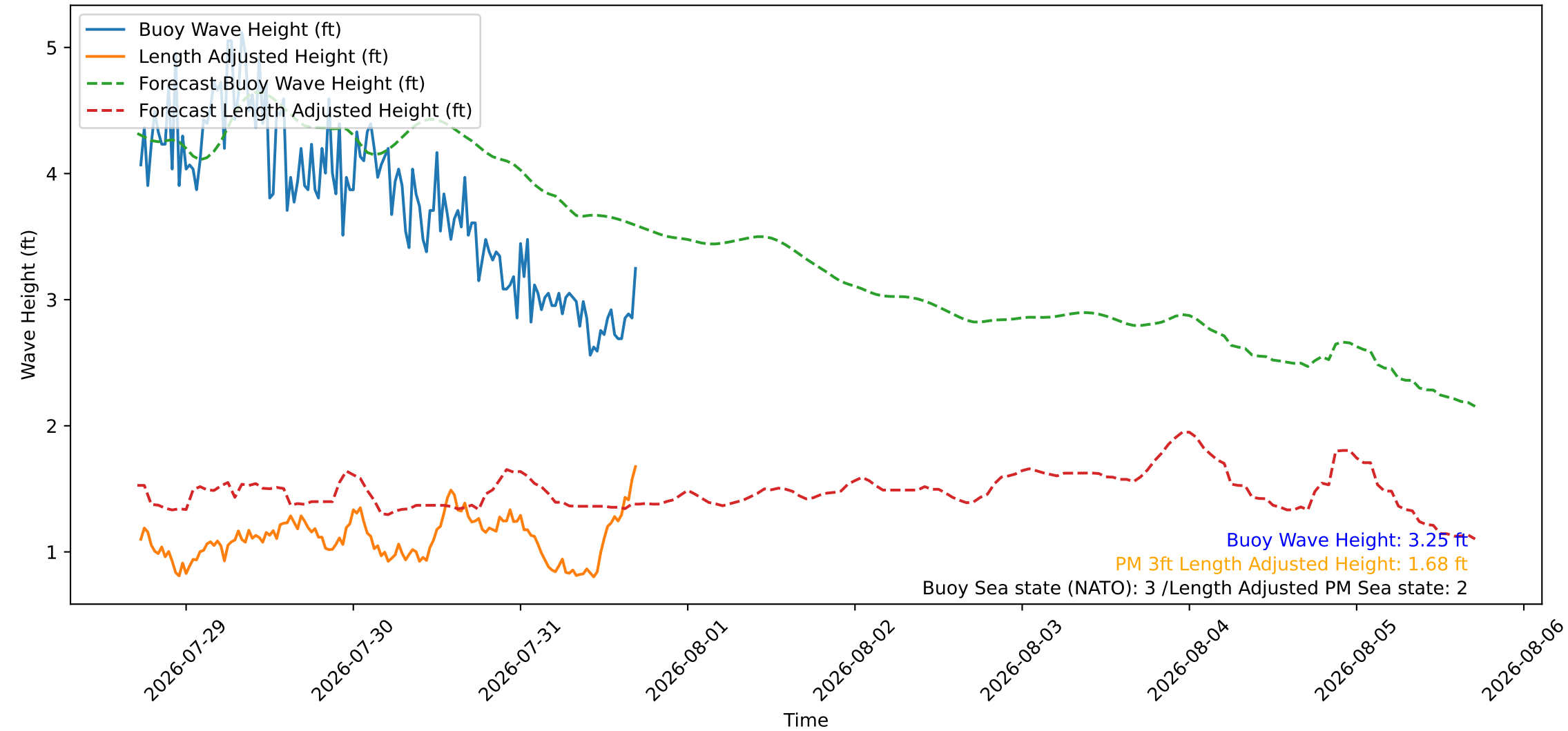
Wave Heights over Time for Red Beach at 2026-07-31 17:10:46
