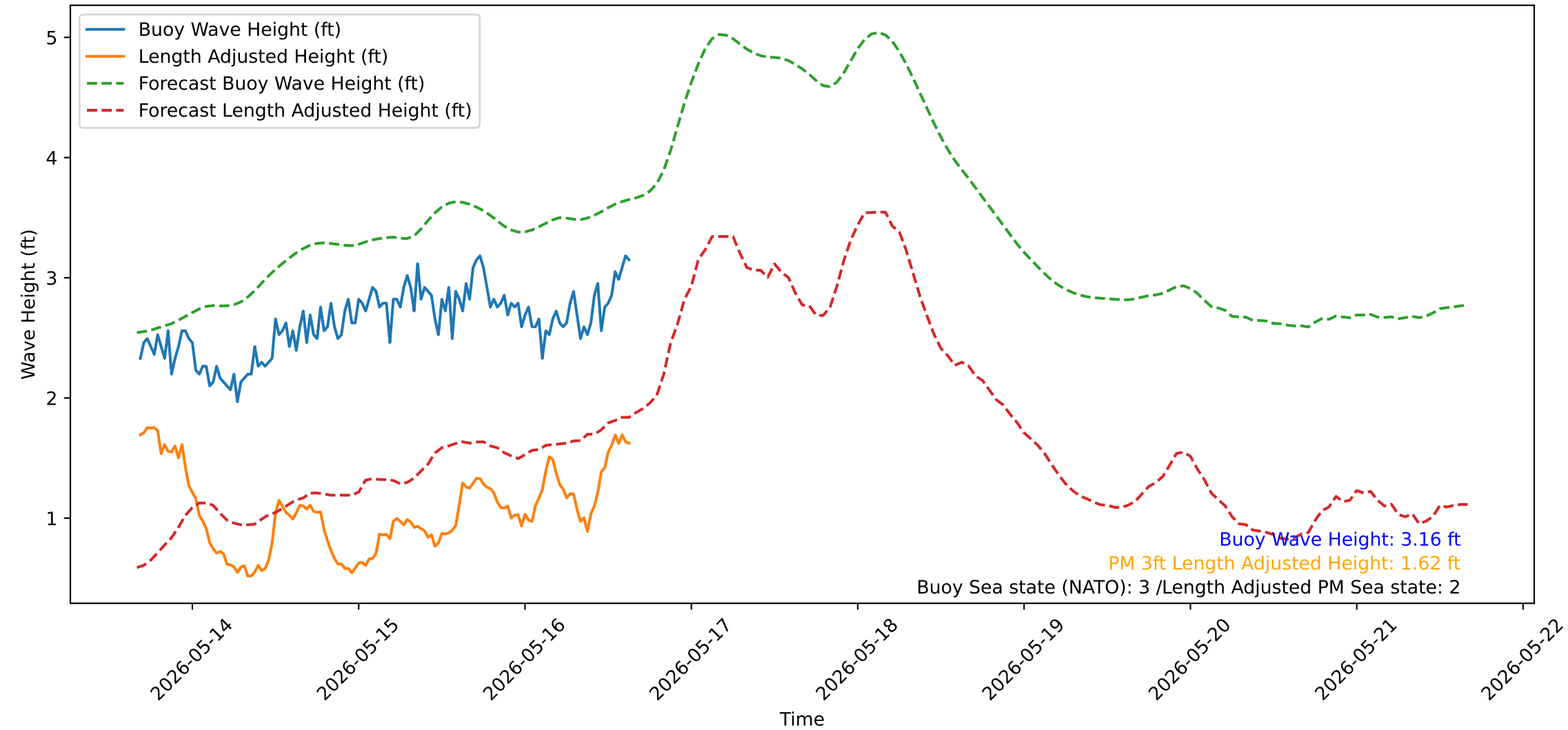
Wave Heights over Time for Red Beach at 2026-05-16 16:00:50
