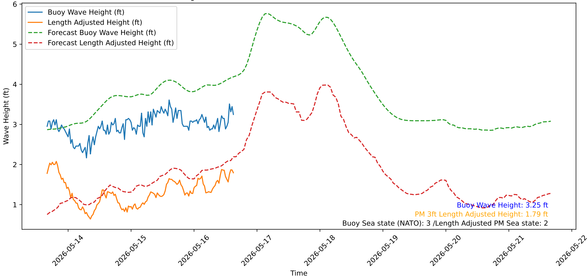
Wave Heights over Time for Oceanside Harbor at 2026-05-16 16:00:30
