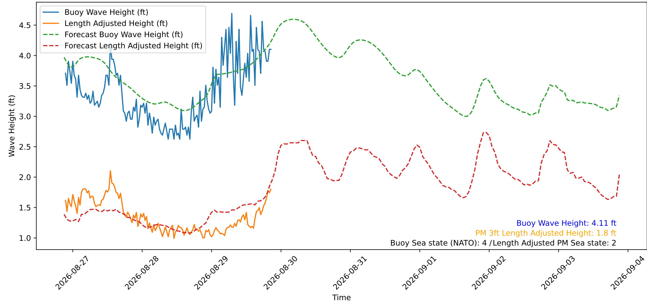
Wave Heights over Time for Red Beach at 2026-08-29 21:20:51
