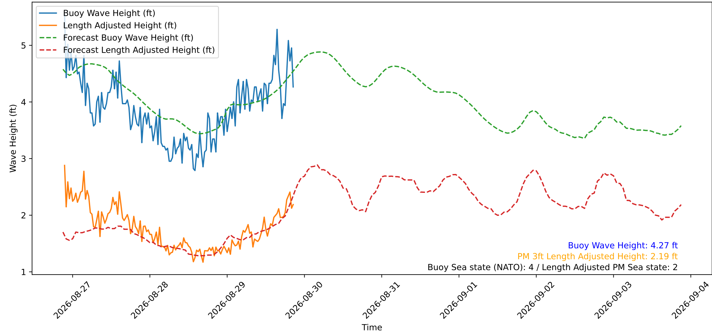
Wave Heights over Time for Oceanside Harbor at 2026-08-29 21:20:29
