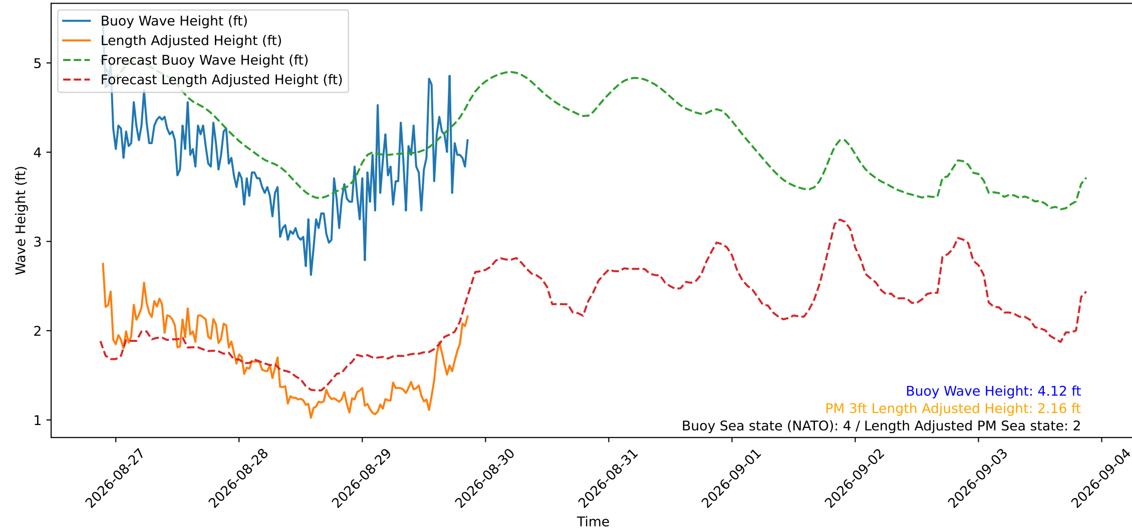
Wave Heights over Time for Green Beach at 2026-08-29 21:21:15
