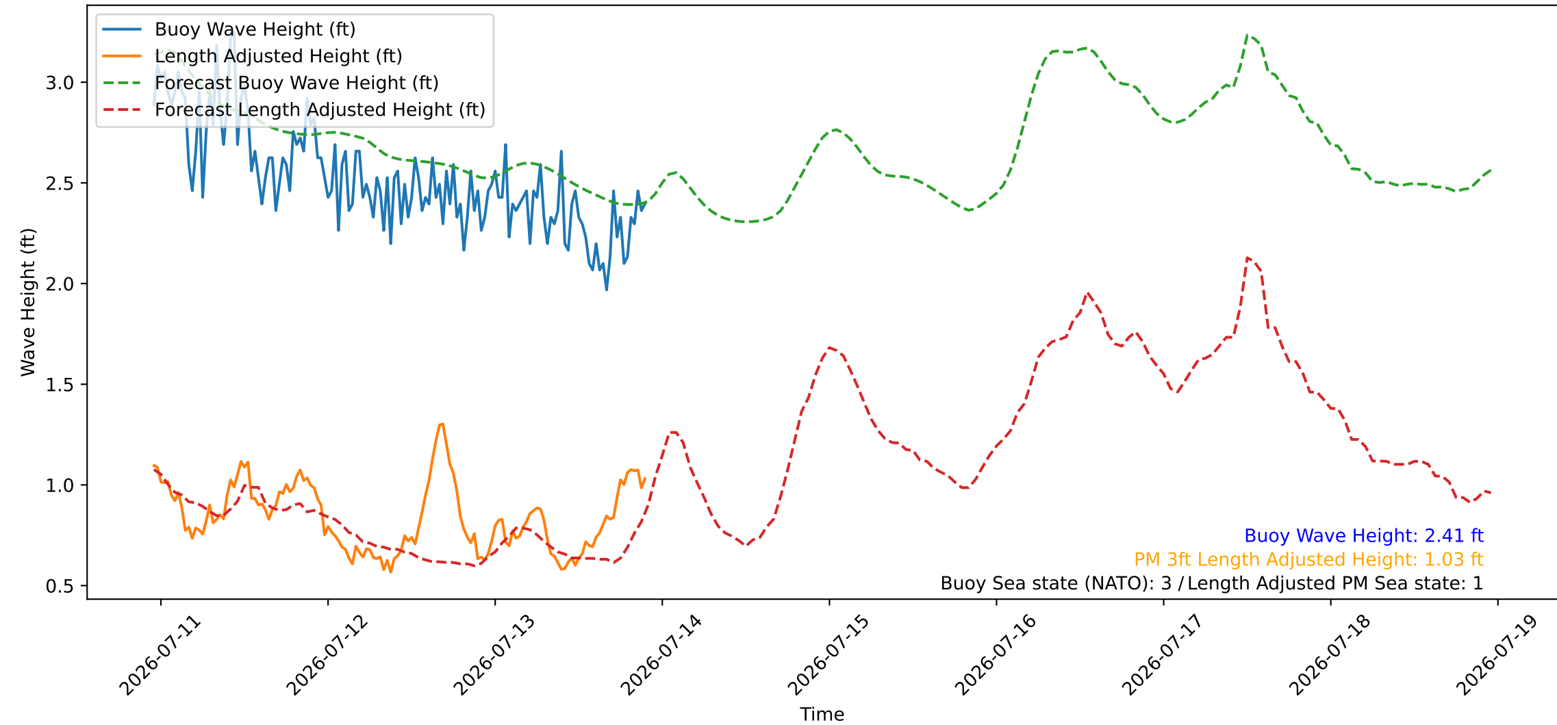
Wave Heights over Time for Red Beach at 2026-07-13 22:40:46
