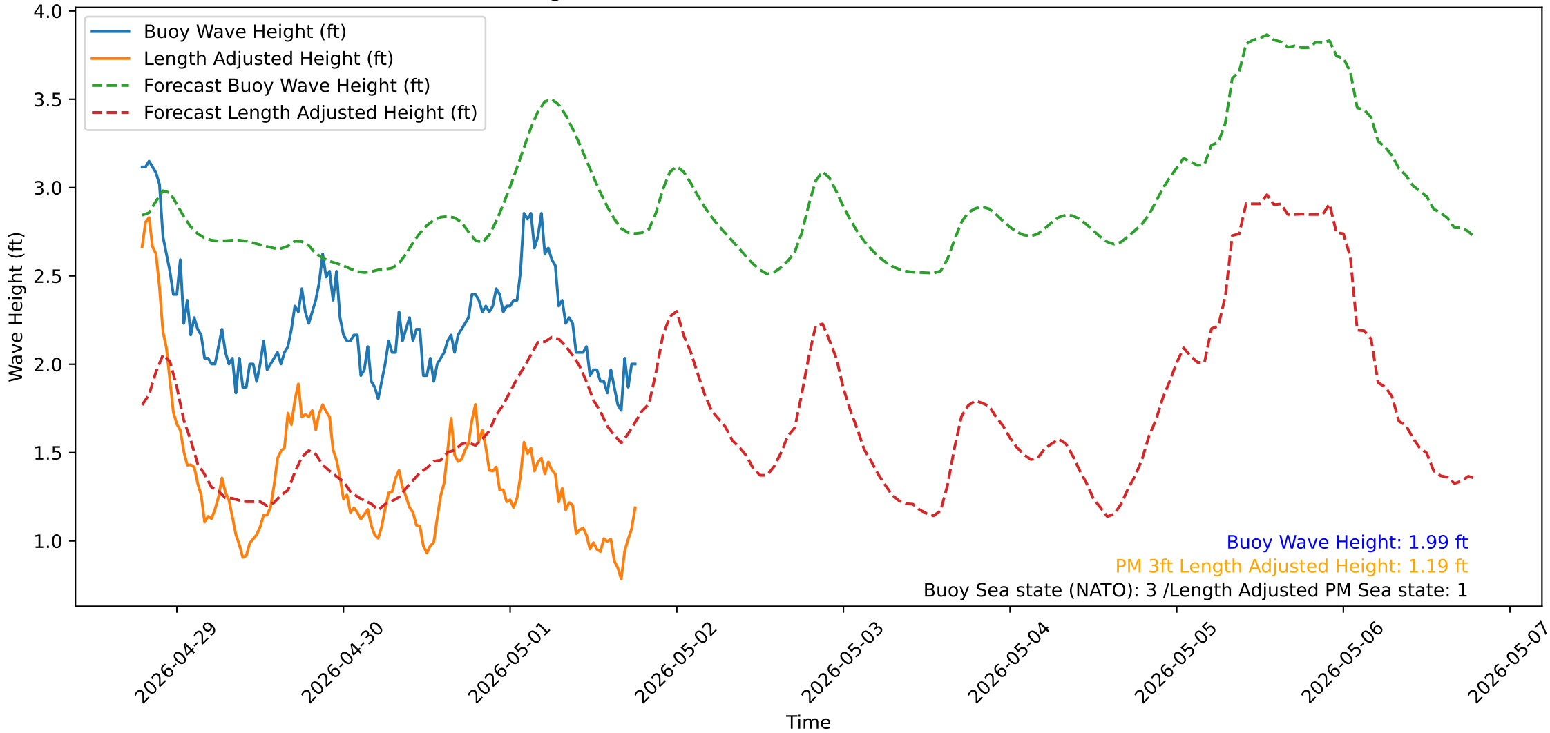
Wave Heights over Time for Green Beach at 2026-05-01 18:51:15
