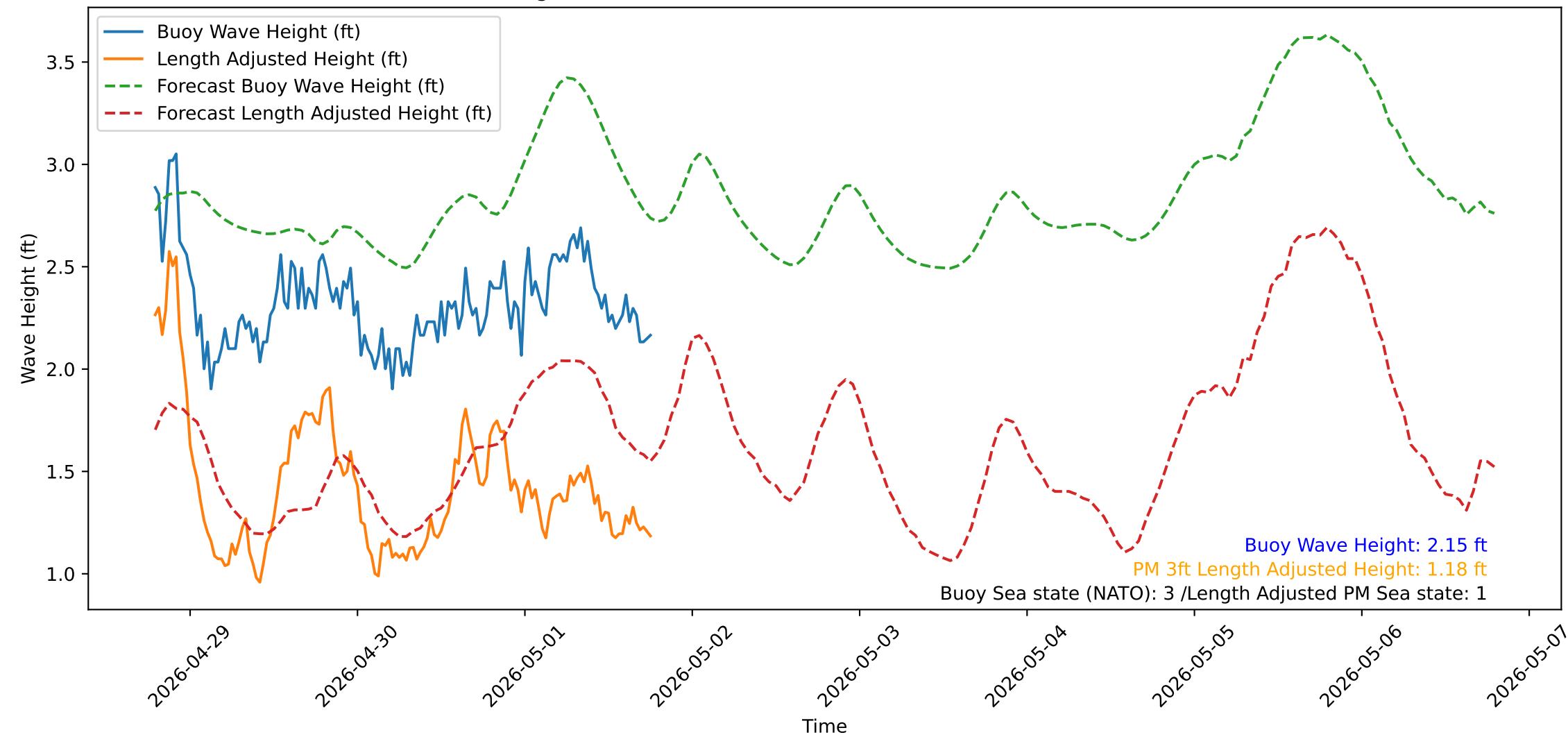
Wave Heights over Time for Oceanside Harbor at 2026-05-01 18:50:31
