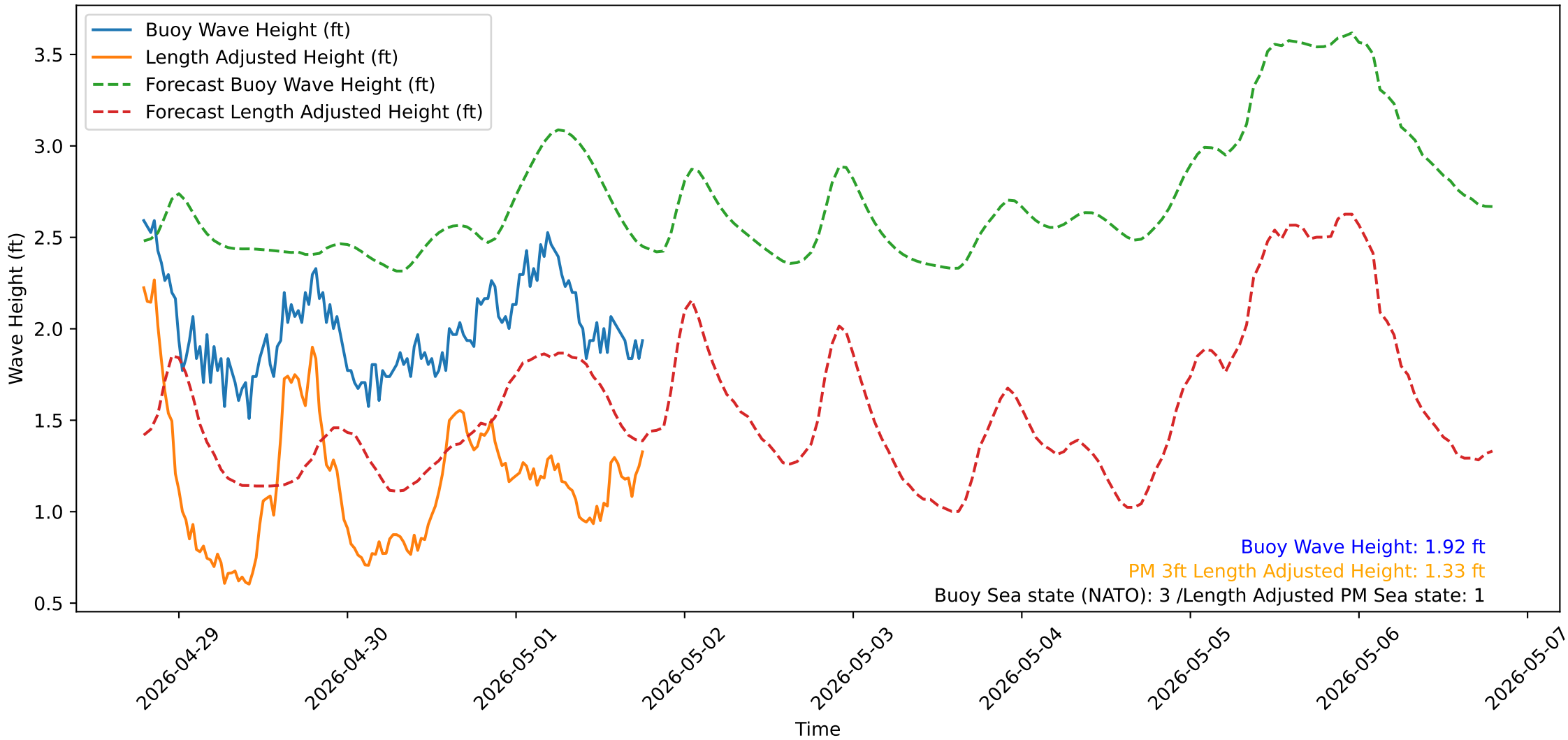
Wave Heights over Time for Red Beach at 2026-05-01 18:50:53
