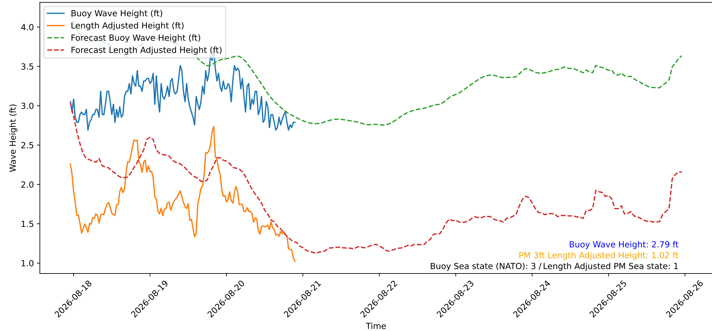
Wave Heights over Time for Green Beach at 2026-08-20 22:31:08
