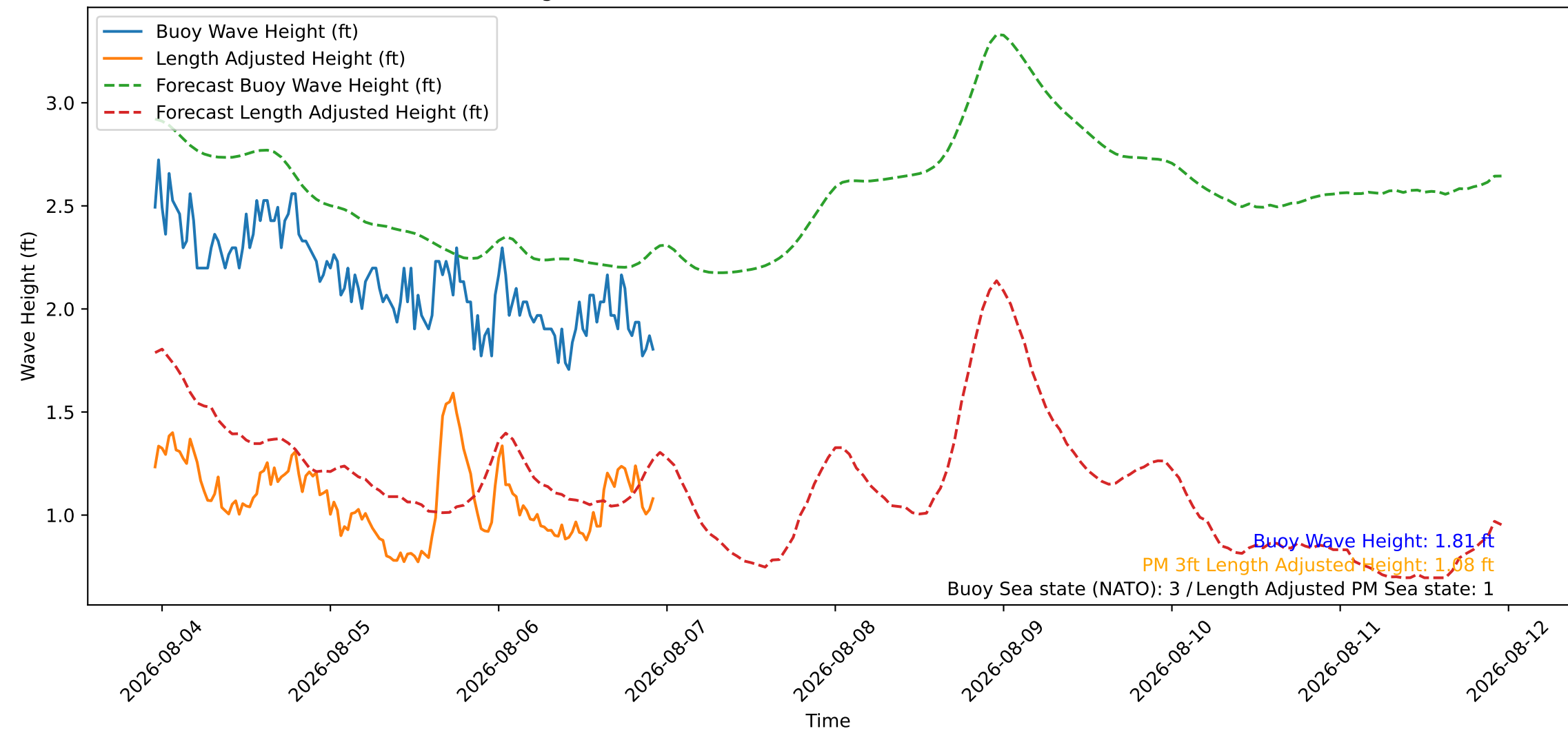
Wave Heights over Time for Oceanside Harbor at 2026-08-06 22:50:26
