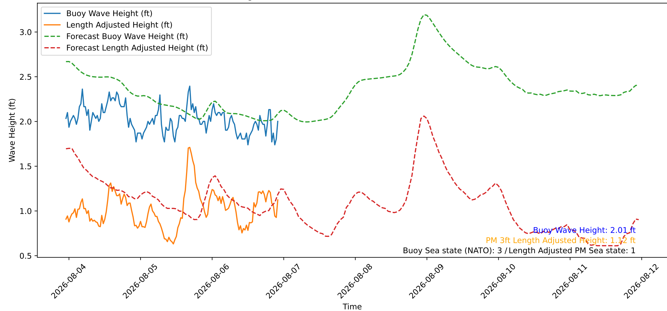
Wave Heights over Time for Red Beach at 2026-08-06 22:50:47
