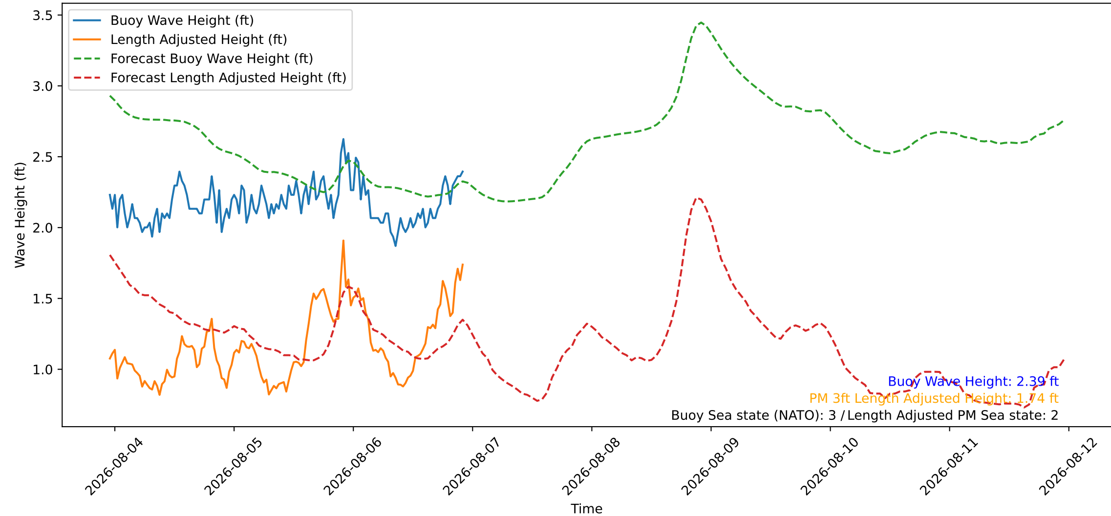
Wave Heights over Time for Green Beach at 2026-08-06 22:51:10
