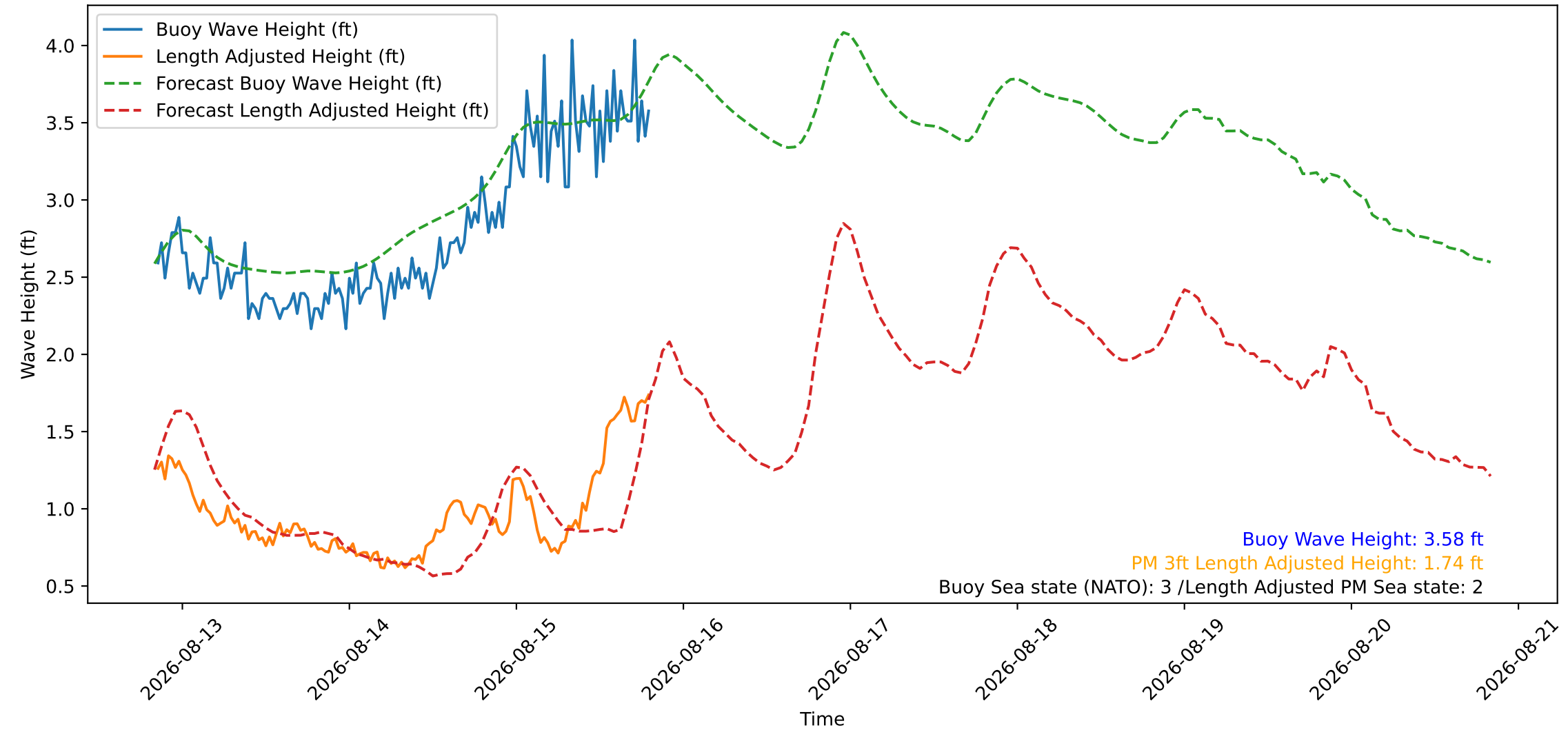
Wave Heights over Time for Red Beach at 2026-08-15 20:00:46
