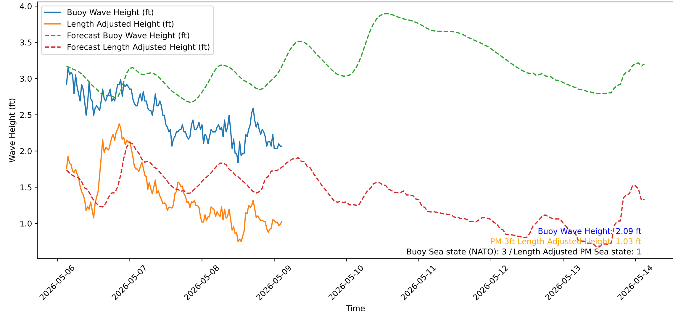
Wave Heights over Time for Green Beach at 2026-05-09 03:11:13
