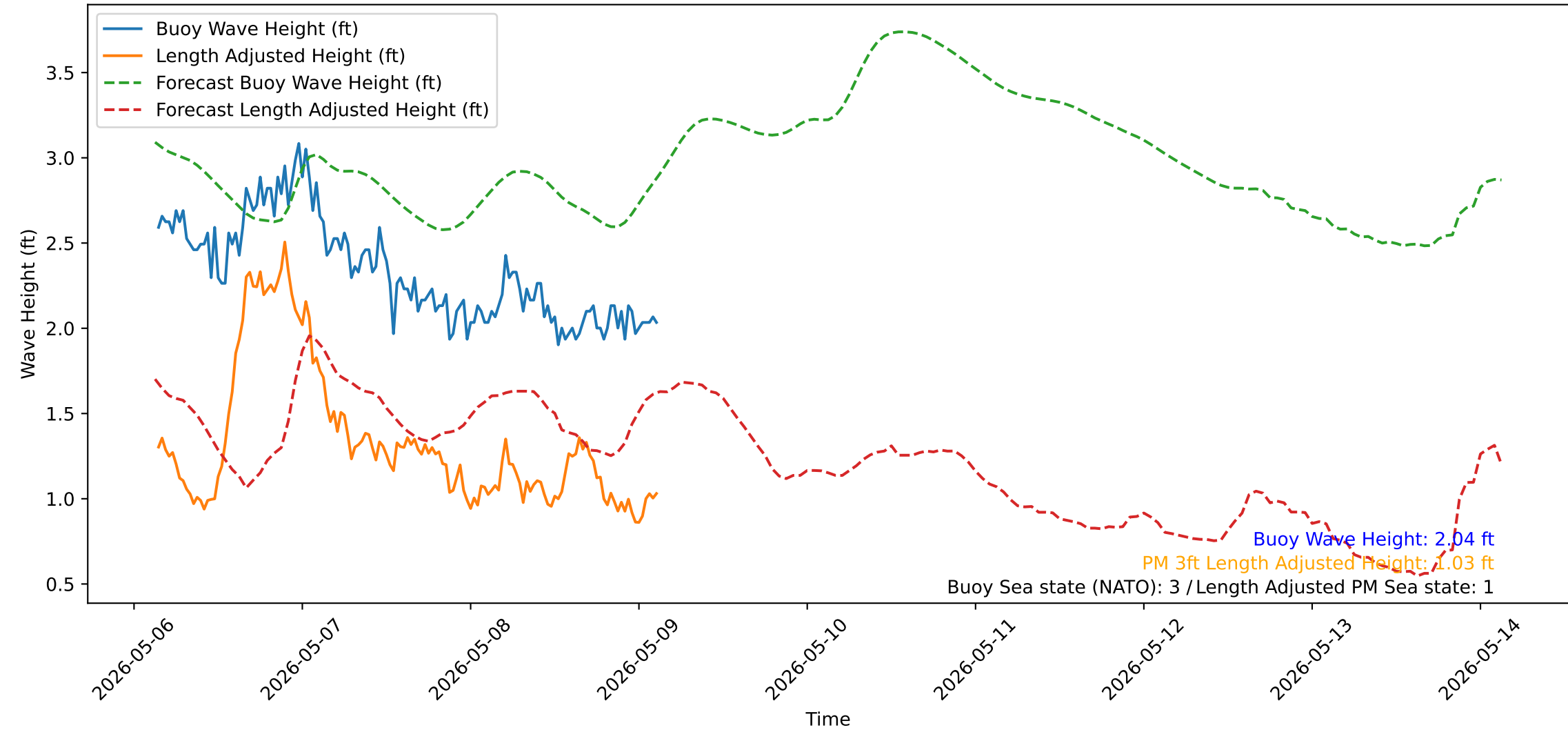
Wave Heights over Time for Red Beach at 2026-05-09 03:10:51
