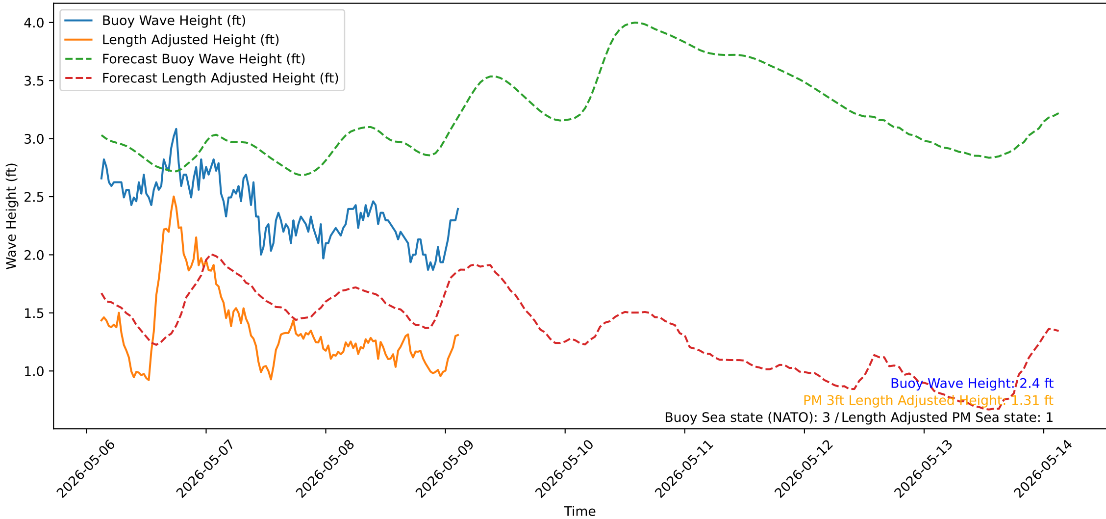
Wave Heights over Time for Oceanside Harbor at 2026-05-09 03:10:31
